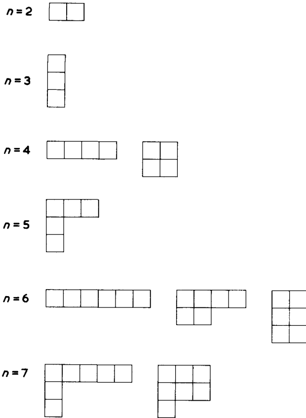
FIG. 2. Frames for tensors of rank n .
