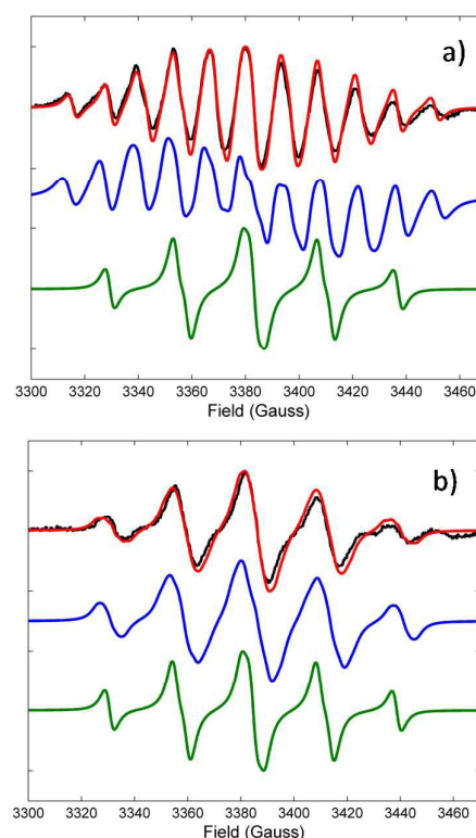
Figure 2. EPR spectra of \text{A}^0 (a) and its deuterated form (b). In each panel black, red and blue lines correspond to experimental, fitted and predicted from DFT spectra, respectively. Spectra obtained with hydrogen and deuterium
