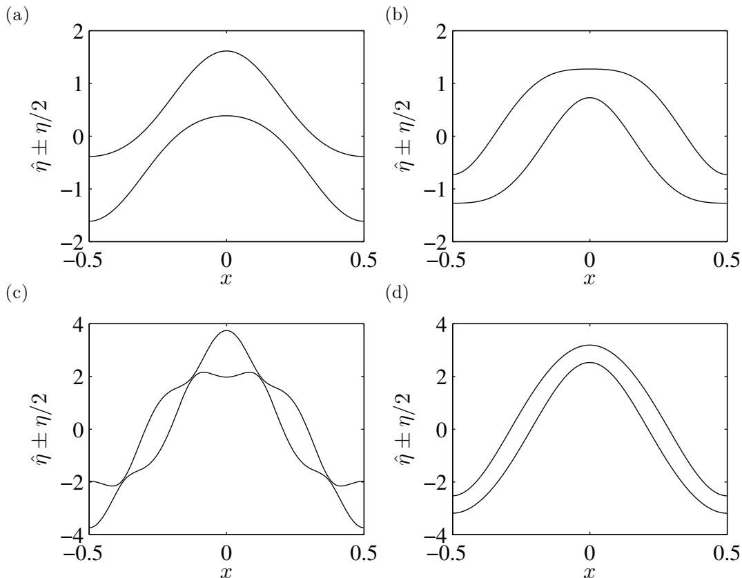
Figure 7: The deformed wall positions for four mixed-mode travelling wave solutions of (50) and (51). (a) \delta = 0.1 , \hat{\eta}(0) = 0.1 , \tilde{c} = 11.7 , (b) \delta = 0.1 , \hat{\eta}(0) = 0.1 , \tilde{c} = 13.6 , (c) \delta = 0.07 , \hat{\eta}(0) = 0.2 , \tilde{c} = 7.85 , and (d) \delta = 0.07 , \hat{\eta}(0) = 0.2 , \tilde{c} = 13.4 . These parameter choices are indicated by the small crosses in figure 6 above.
