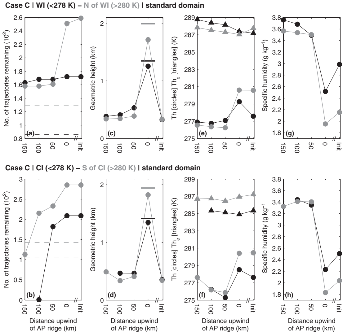
Figure 15. Lagrangian changes for mean back trajectories, as in Figure 12, but for back trajectories initiated at 2200 UTC on 15 November 2010 during case C. Diagnostics illustrated are (a, b) number of trajectories; (c, d) geometric height; (e, f) \theta (Th; circular markers) and equivalent \theta (The; triangular markers); and (g, h) q .
