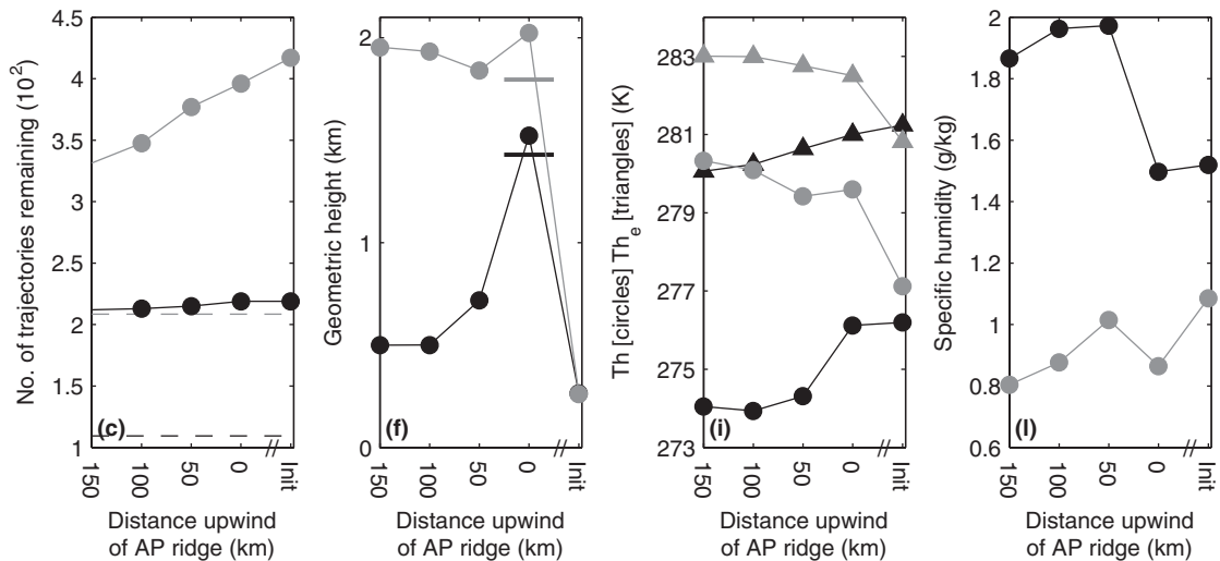
Figure 12. Lagrangian changes following back trajectories initiated at 1000 UTC 5 February 2011 during case A within each of the jet (black lines) and wake (grey lines) regions. The five diagnostics illustrated are (a–c) number of trajectories; (d–f) geometric height; (g–i) \theta ( \theta ; circular markers) and equivalent \theta ( \theta_e ; triangular markers); and (j–l) q . The x-axis is trajectory distance upwind of the AP, but also includes an increment for trajectory initiation ('Init') above the Larsen. The dashed horizontal lines in the left panels correspond to half the total number of trajectories. The horizontal lines in the trajectory height panels are the mean estimated peak heights of orography traversed for each set of trajectories.
