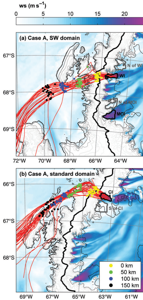
Figure 10. Case A back trajectories (red) initiated within (a) the WI jet region in the SW domain and (b) the CI jet region in the standard domain, overlaying wind speed at the 950 hPa level at the time of trajectory initiation (1000 UTC 5 February 2011). To enhance legibility only one in four trajectories is plotted. The yellow, green, blue and black dots indicate the positions of air parcels respectively 0, 50, 100 and 150 km upwind of the AP’s crest line (solid black line) for each trajectory. The six trajectory initiation regions are marked and labelled; black boundaries enclose ‘jet’ regions, whilst grey boundaries enclose ‘wake’ regions.
