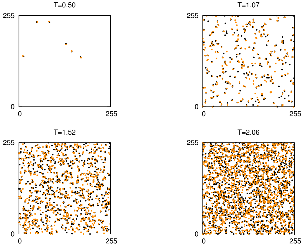
FIG. 14. (Color online) Numerically detected quantum vortices in the final steady states for four simulations with L = 256 and different temperatures. Clockwise and anti-clockwise vortices are shown by dark yellow and black colours respectively. Vortex number increases when increasing the temperature and clear hydrodynamic dipoles are only observed at very low temperatures, well below the estimated T_{BKT} .
