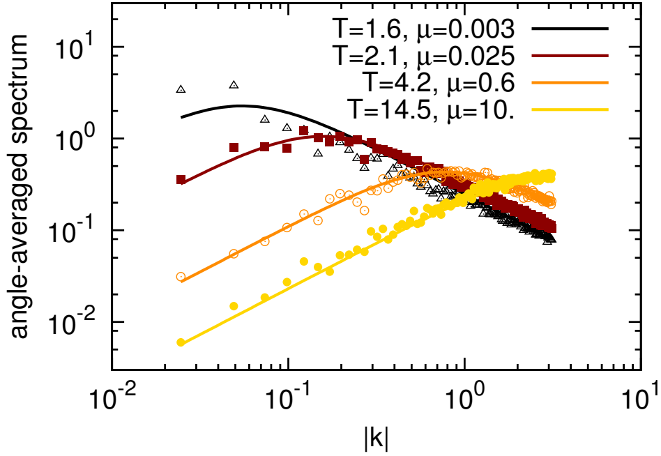
FIG. 10. (Color online) Angle-averaged steady state spectra (points) measured in different simulations having high free-particle energy densities and negligible condensate fraction. The spectra are fitted with curves corresponding to the Rayleigh-Jeans distribution (18) integrated over angles, that is N_k = \int_0^{2\pi} n_k k d\theta . Corresponding fitted values of temperature and chemical potential are shown in the labels. Results are taken from simulations with L = 256 .
