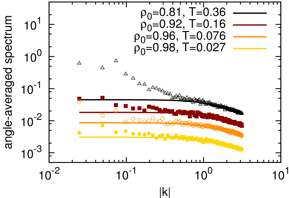
FIG. 11. (Color online) Angle-averaged steady state spectra (points) of Bogoliubov normal variables (23) measured in different simulations having low free-particle energy densities and strong condensate fraction. The spectra are fitted with curves corresponding to the Rayleigh-Jeans distribution (32) integrated over angles, that is N_k = \int_0^{2\pi} n_k k d\theta . Corresponding fitted values of temperature and condensate fraction are shown in the labels. Results are taken from simulations with L = 256 .
