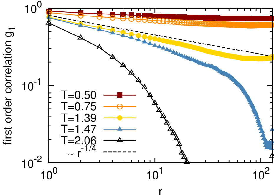
FIG. 7. (Color online) Real part of the first-order correlation function of the field \psi for different temperatures as a function of an angle-averaged distance r in a log-log plot. Results are taken from simulations having system size L = 256 . The change from exponential to power-law behaviour characteristic to the BKT transition is clearly observed. The power-law having slope \alpha = -1/4 at the transition temperature T_{BKT} is also shown.
