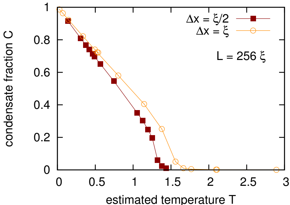
FIG. 13. (Color online) Measured condensate fraction with respect to the estimated temperatures fitted from spectra for systems having same size L = 256\xi but different resolution \Delta x = \xi and \Delta x = \xi/2 . Results indicate that a better resolved system manifests a lower condensation temperature.
