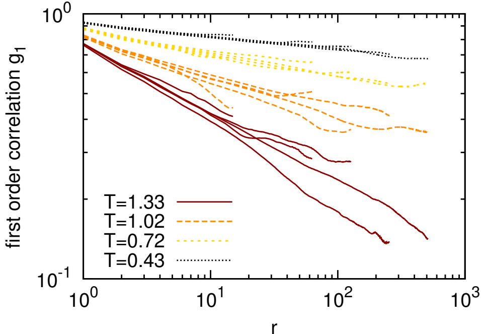
FIG. 8. (Color online) Real part of the first-order correlation function of the field \psi for different temperatures below the estimated T_{BKT} as a function of an angle-averaged distance r in a log-log plot. Same coloured lines refer to simulations having the same temperature but different system sizes: similar exponents in the power-laws are observed for the same temperature.
