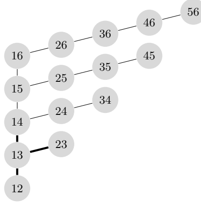
FIGURE 1. An example of the \leq ordering for n = 6 , r = 2 . The bold edges correspond to the regions of the graph \Delta(P_r) drawn in Figure 2.
