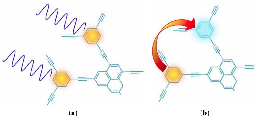
Figure 8. A mechanism for delivering the energy of two photons to a single site (specific dendrimer components shown only for illustration); (a) two peripheral antenna chromophores are excited; (b) the energy acquired by one of the chromophores is transferred to the other, which becomes doubly excited.
