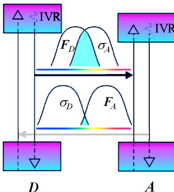
Figure 1. Energetics for pair-wise RET and associated spectral overlaps: (top) transfer from D to A ; (below) potential backward transfer, A to D : F —fluorescence spectrum; \sigma —absorption spectrum; IVR—intramolecular vibrational relaxation.
