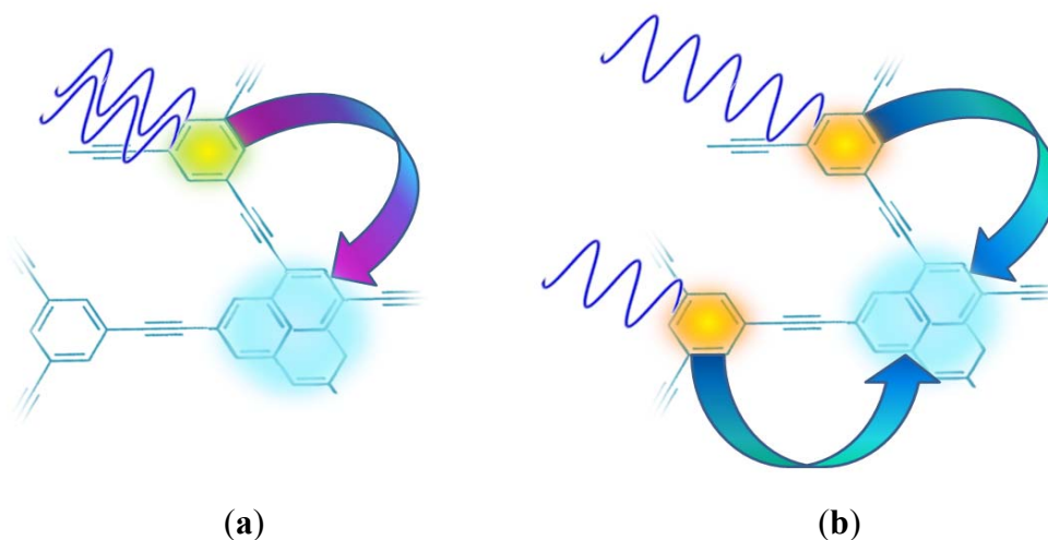
Figure 9. Alternative mechanisms for delivering the energy of two photons, captured by one or more higher-generation or peripheral antenna chromophores, to a lower generation neighbour (specific dendrimer components shown only for illustration): (a) direct transfer of the energy acquired by two-photon absorption in a single outer chromophore (b) the pooling of energy from two outer chromophores, each individually excited by single-photon absorption.
