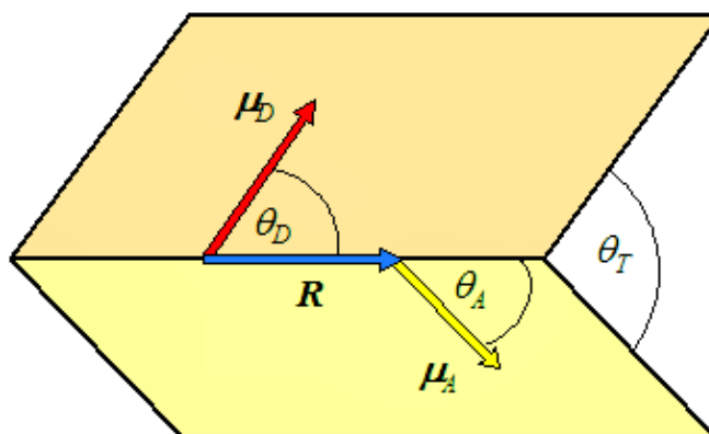
Figure 2. Relative orientations and positions of donor and acceptor and their transition moments: angles \theta_D and \theta_A are subtended by the donor and acceptor dipole transition moments ( \mu_D and \mu_A , respectively) against the inter-chromophore displacement vector, R ; \theta_T is the angle between the transition moments.
