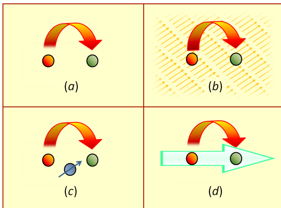
Figure 4. Schematic depictions of: (a) resonance energy transfer; (b) electric-field induced energy transfer; (c) third-body (dipole-assisted) energy transfer; (d) laser-assisted resonance energy transfer, the throughput beam being off-resonant with respect to the donor and acceptor spectra.
