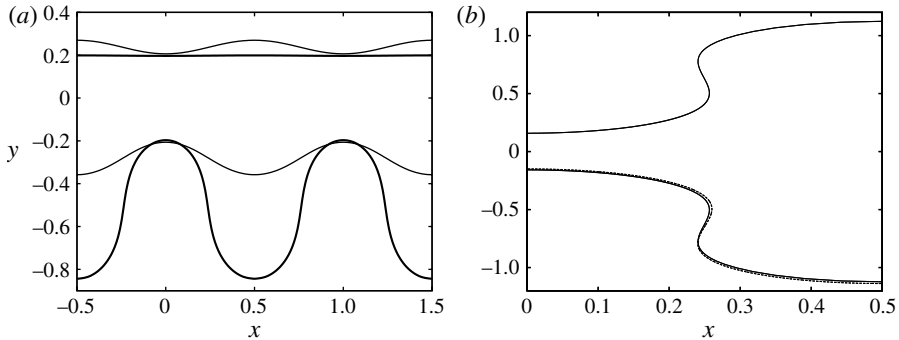
FIGURE 9. Q = -0.5 . (a) Profiles on the upper bifurcation branch for D = 0.005 ( N = 80 , thin lines) and D = 0.05 ( N = 200 , thick lines). (b) An overturning profile for \sigma = 0.9 ( N = 1900 ). The broken line overlaid onto the lower wave is the static wave prediction for d = 40.3 .
