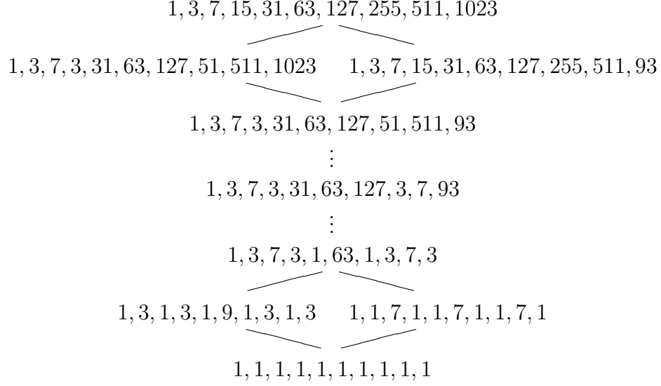
FIGURE 1. Part of the Hasse diagram for [\mathbb{K}(t - 2)] .
