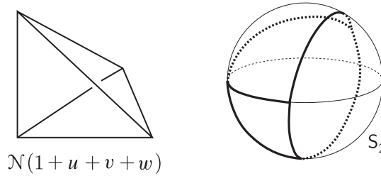
FIGURE 4. The non-expansive set for 3-dimensional Ledrappier.
