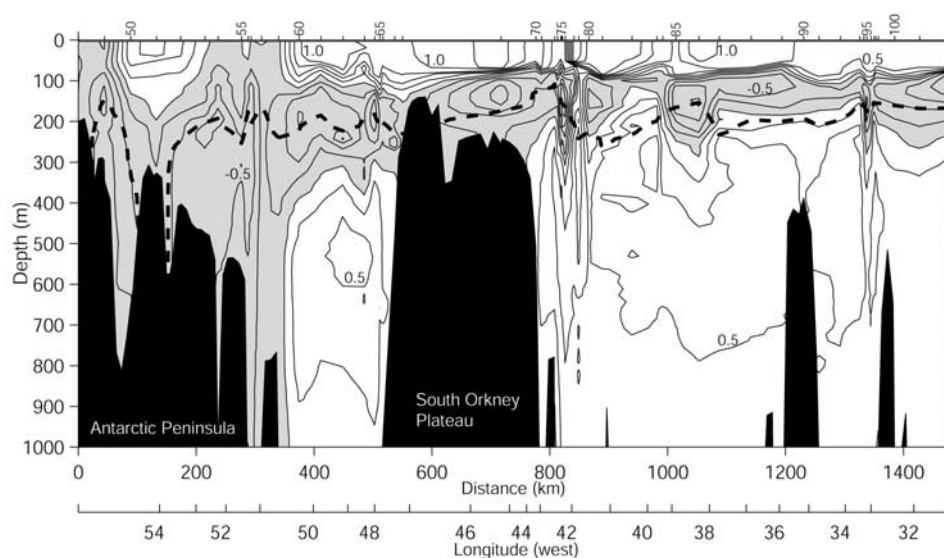
Figure 2a. Potential temperature (°C) section from the ALBATROSS survey along the South Scotia Ridge showing the top 1000 m only. Contour interval is 0.25°C, and values < 0°C are shaded. The thick dashed line marks the \gamma^n = 28.0 neutral density surface. Selected station numbers are indicated on the upper axis.
