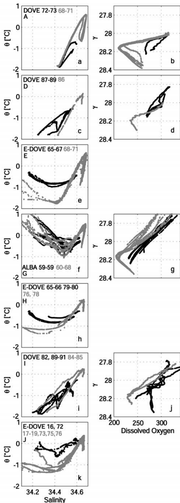
Figure 4. Diagrams of (left) potential temperature–salinity (right) and neutral density–dissolved oxygen ( \mu\text{mol kg}^{-1} ) across the Antarctic Slope Front (ASF) for (a, b) Joinville Island, east of the Antarctic Peninsula; (c–e) northwestern Powell Basin; (f–h) Philip Passage; and (i–k) Hesperides Trough. Stations in gray are to the south or east of the ASF; stations in black are to the north or west of the ASF. Dissolved oxygen data are not available for the E-DOVETAIL survey. For locations of subsections, indicated by capital letters, see Figure 1 and Table 1. DOVETAIL, E-DOVETAIL, and ALBATROSS are indicated by DOVE, E-DOVE, and ALBA, respectively.
