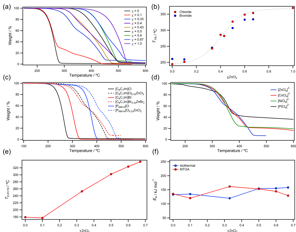
Fig. 2 TGA data and derived parameters of halometallate ionic liquids in N_2 , showing: (a) 10 °C min -1 ramping experiments for [C_8C_1Im]Cl_xZnCl_2 ; (b) plot of T_{1\%} as a function of ZnCl_2 mole fraction for [C_8C_1Im]Cl_xZnCl_2 , with bromide analogues; (c) 10 °C min -1 ramping experiments for [Cation]X_{0.33}ZnX_2 with metal-free analogues; (d) 10 °C min -1 ramping experiments for [C_8C_1Im]Cl_xMCl_2 for four tetrahedral metals; (e) long term thermal stability parameter T_{0.01/10} as a function of mole fraction for [C_8C_1Im]Cl_xZnCl_2 ; (f) E_a of thermal decomposition for [C_8C_1Im]Cl_xZnCl_2 from isothermal and MTGA.
