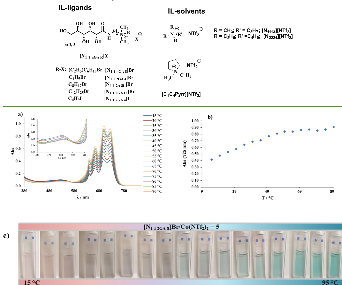
Figure 1. (a) UV-vis spectra of [N_{1\ 1\ 2GA\ 8}]Br/Co(NTf_2)_2/[N_{2224}][NTf_2] at a ligand/metal molar ratio equal to 5 (inset: high energy band); (b) trend of absorbance at 725 nm as a function of temperature; (c) color shades.
