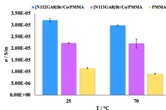
Figure 10. Conductivity ( \sigma ) values at variable temperature for PMMA layer and thermochromic films: [N_{112GA8}]Br/[N_{2224}][NTf_2]_2/PMMA (3:1) (85% of PMMA) and [N_{113GA8}]Br/[N_{2224}][NTf_2]_2/PMMA (3:1) (84% of PMMA).
