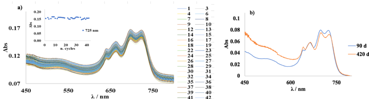
Figure 8. (a) UV-vis spectra recorded for [N_{1\ 1\ 3GA\ 8}]Br/Co(NTf_2)_2 (3:1)/PMMA film at 60 °C (inset: absorbance at 725 nm as a function of the number of cycles); (b) UV-vis spectra after 90 and 420 days.
