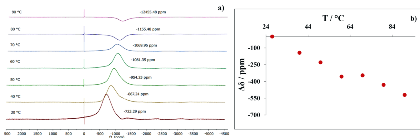
Figure 5. VT ^{59}\text{Co} NMR for the system [\text{N}_{1.12}\text{GA}_8]\text{Br}/\text{Co}(\text{NTf}_2)_2/[\text{N}_{2.22}\text{A}_4][\text{NTf}_2] (7:1) (a) spectra recorded in the range 30–90 °C ( ^{59}\text{Co} signal for \text{K}_3[\text{Co}(\text{CN})_6] fixed at 0 ppm); (b) trend of \Delta\delta as a function of the temperature in the range 30–90 °C.
