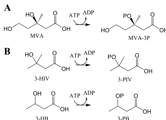
FIG 6 M3K reaction scheme. (A) The natural substrate of M3K is ( R )-mevalonate (MVA), which is converted to ( R )-mevalonate-3-phosphate (MVA-3P). (B) PtM3K is also active on 3-hydroxyisovalerate (3-HIV) and 3-hydroxybutyrate (3-HB) to produce 3-phosphoisovalerate (3-PIV) and 3-phosphobutyrate (3-PB), respectively.
