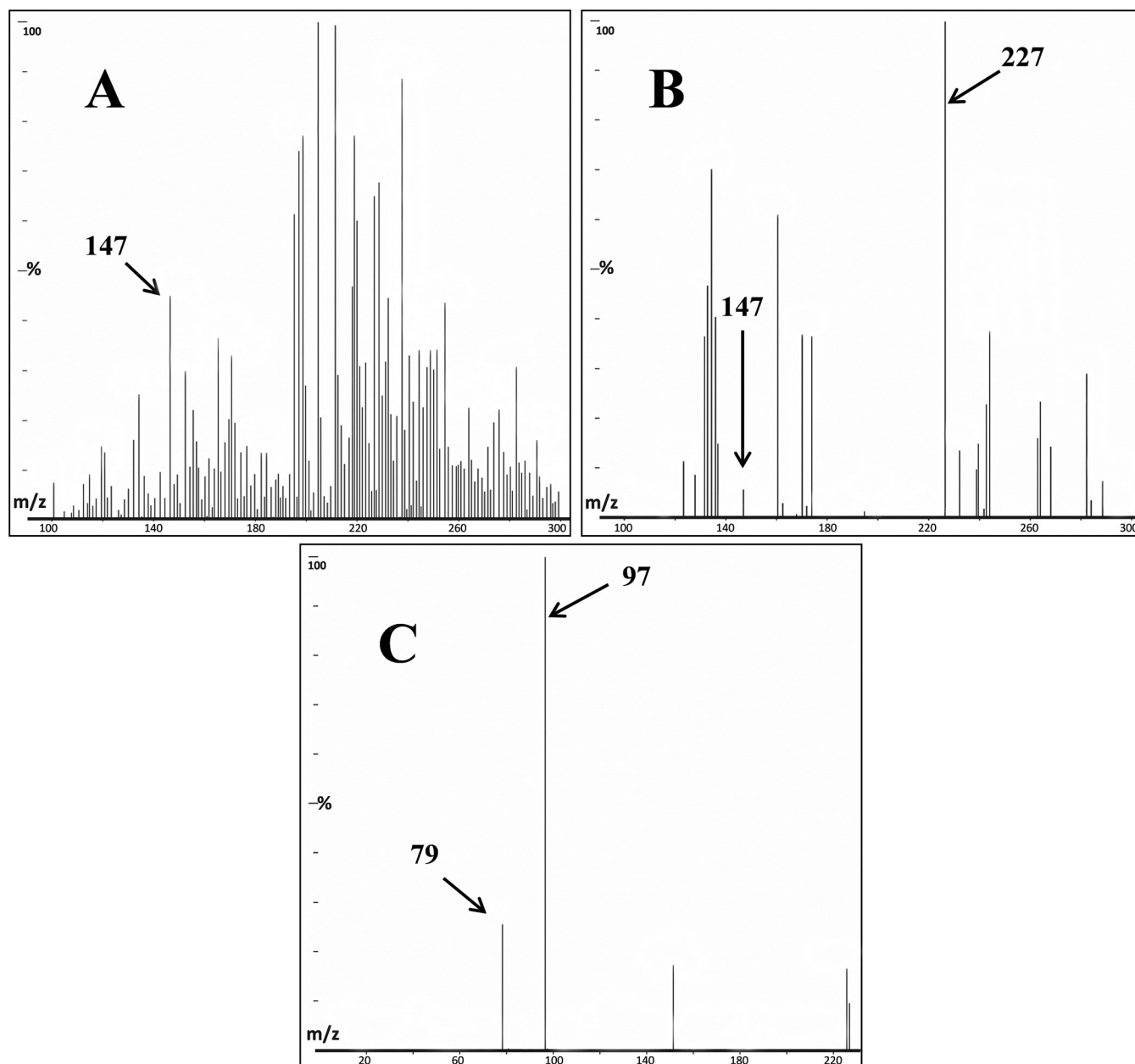
FIG 4 ESI-MS analysis. All spectra were collected in negative ion mode. The mass spectra are shown. (A) Control sample containing MVA but without added enzyme; (B) sample containing MVA and P ut PtMVD; (C) MS-MS spectrum of 227 m/z ion yielding phosphate ions (97 and 79 m/z ). The reaction was performed in 50 mM Tris-HCl buffer, pH 7.5, with the addition of 10 mM MgCl 2 and 20 mM KCl. Samples were analyzed after 24 h.
