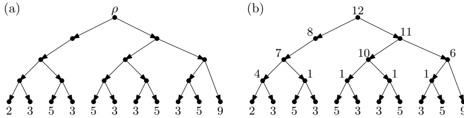
Figure 3: (a) A leaf-labeled tree (\mathcal{T}, \lambda) . (b) The full labeling \phi = \phi_{(\lambda, \preceq)} of the leaf-labeled tree in (a) produced by Algorithm 1 using as \preceq the lexicographic ordering. All the leaf-labeled trees (\mathcal{T}_u, \lambda_u) for vertices u with \phi(u) = 1 are isomorphic (cf. Lemma 1).
