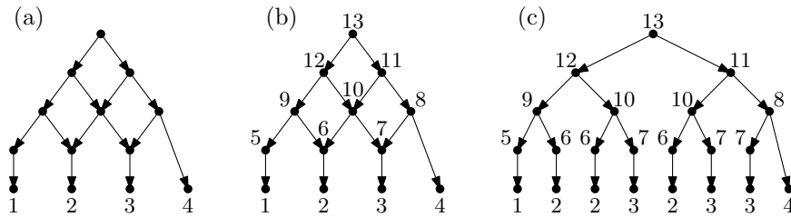
Figure 8: (a) A phylogenetic network on [4] . (b) The fully labeled network obtained by applying Algorithm 1 to the phylogenetic network using as \preceq the ordering considered in [10]. (c) The fully labeled tree resulting from unfolding the fully labeled network.
