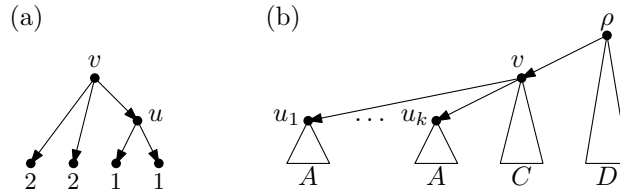
Figure 5: (a) A leaf-labeled tree illustrating that the lexicographic ordering of \mathbb{M} is not labeling-consistent with respect to Algorithm 1. (b) The structure of the leaf-labeled tree used in the proof of Lemma 7. Each triangle represents a set of leaves that are bijectively labeled by the elements of the multiset below the triangle.
