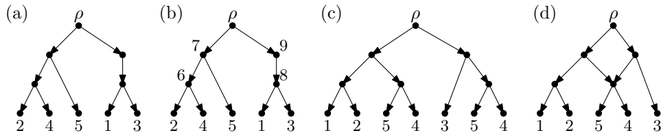
Figure 1: (a) A semi-labeled tree with \ell = 5 and n = 9 . (b) The semi-labeled tree in (a) with vertices (except the root) bijectively labeled with the elements of [9] . Taking for each non-leaf vertex v the subset of [9] labeling the children of v , yields the partition \{\{1, 3\}, \{2, 4\}, \{5, 6\}, \{8\}, \{7, 9\}\} of [9] . (c) A multi-labeled tree. (d) The phylogenetic network obtained by folding the multi-labeled tree in (c).
