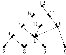
Figure 7: The fully labeled network obtained as the folding of the fully labeled tree in Figure 3(b).
