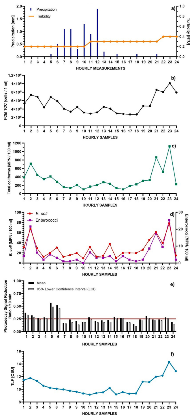
Fig. 6. Results from BD1 monitoring: a) precipitation and turbidity data, b) FCM total cell counts, c) total coliforms, d) E. coli and enterococci, e) FWCs analysis, and f) tryptophan-like fluorescence.
