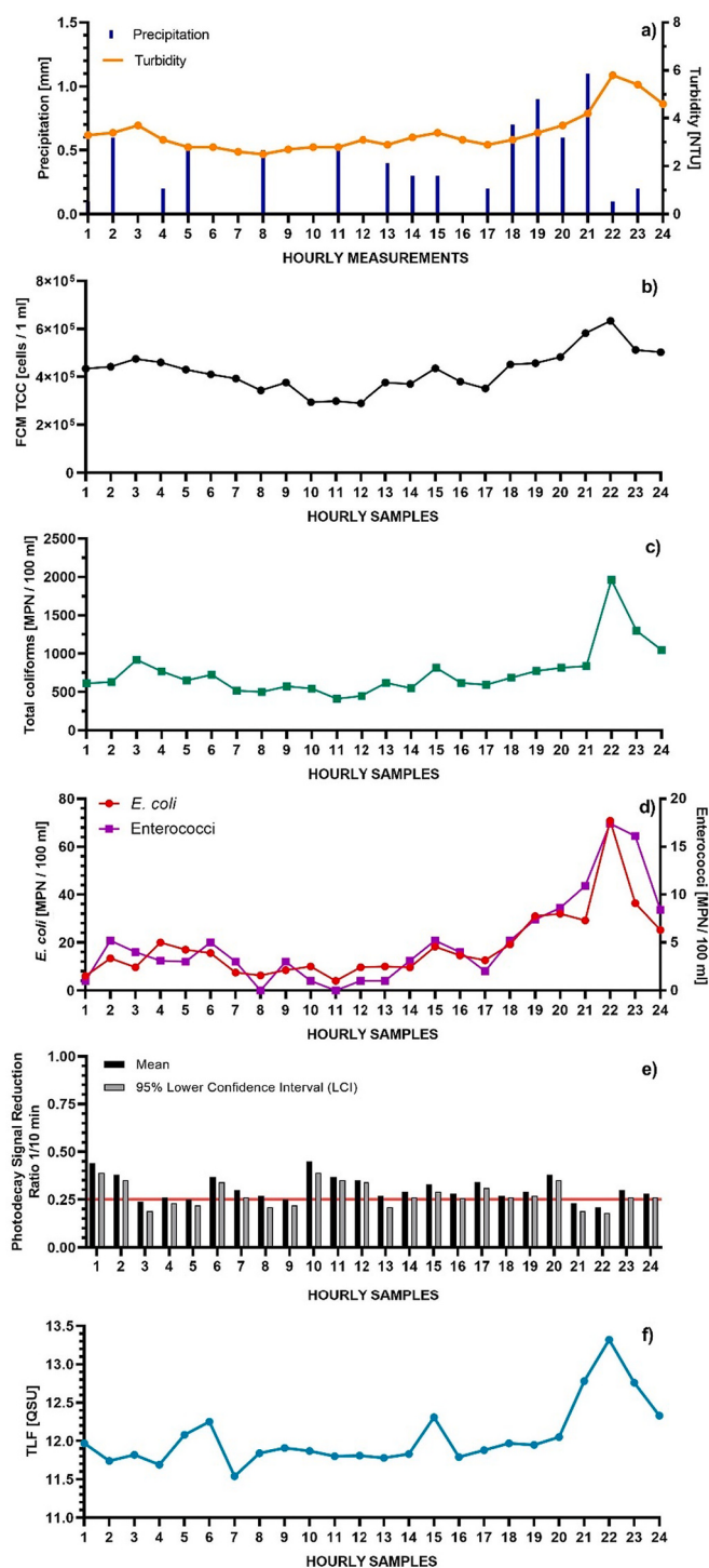
Fig. 4. Results from EL2 monitoring: a) precipitation and turbidity data, b) FCM total cell counts, c) total coliforms, d) E. coli and enterococci, e) FWCs analysis, and f) tryptophan-like fluorescence.
