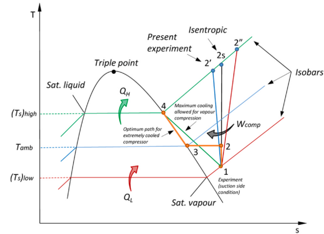
Fig. 6. T-s diagram showing optimum path (1–2–3–4) for cooled refrigeration compressor.
