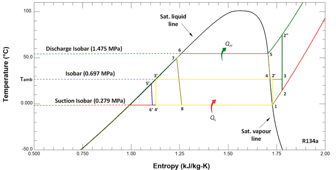
Fig. 9. T-s diagram showing optimum path (2–3–5'–6'–2) for extremely cooled refrigeration compressor.
