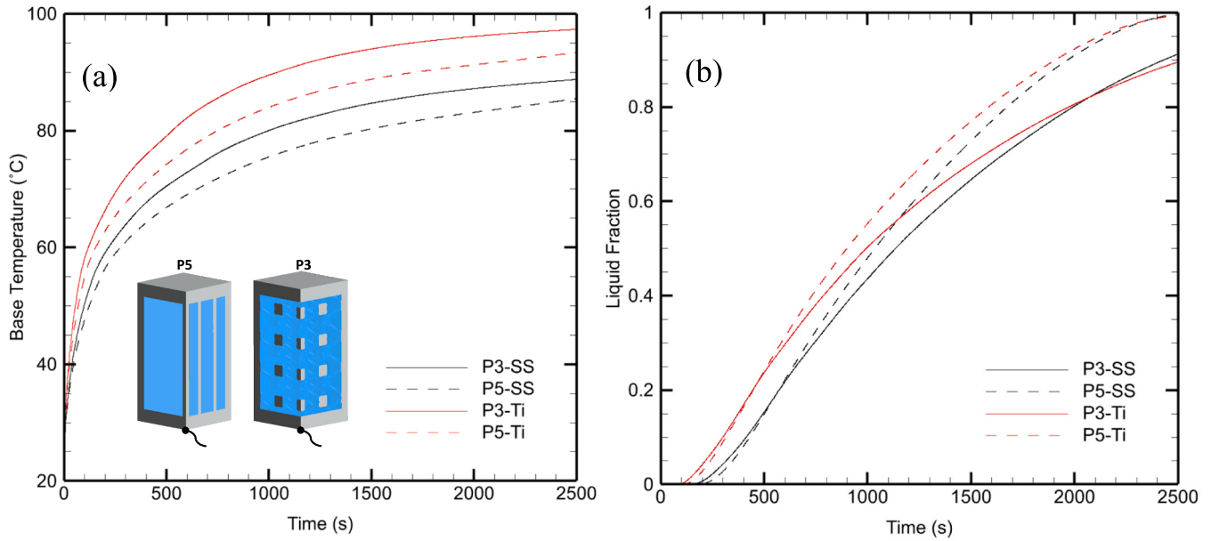
Fig. 10. Effect of base heating (a) base temperature with points of measurement (b) liquid fraction.
