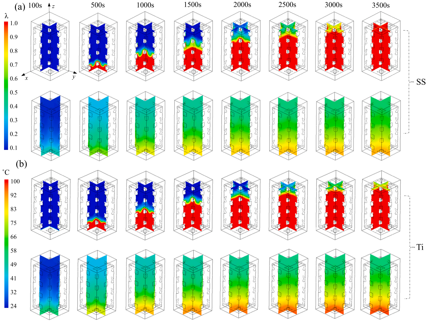
Fig. 6. Transient contours at full heater power (8.6 W) (a) liquid fraction and temperature profiles for stainless steel; (b) liquid fraction and temperature profiles for titanium.
