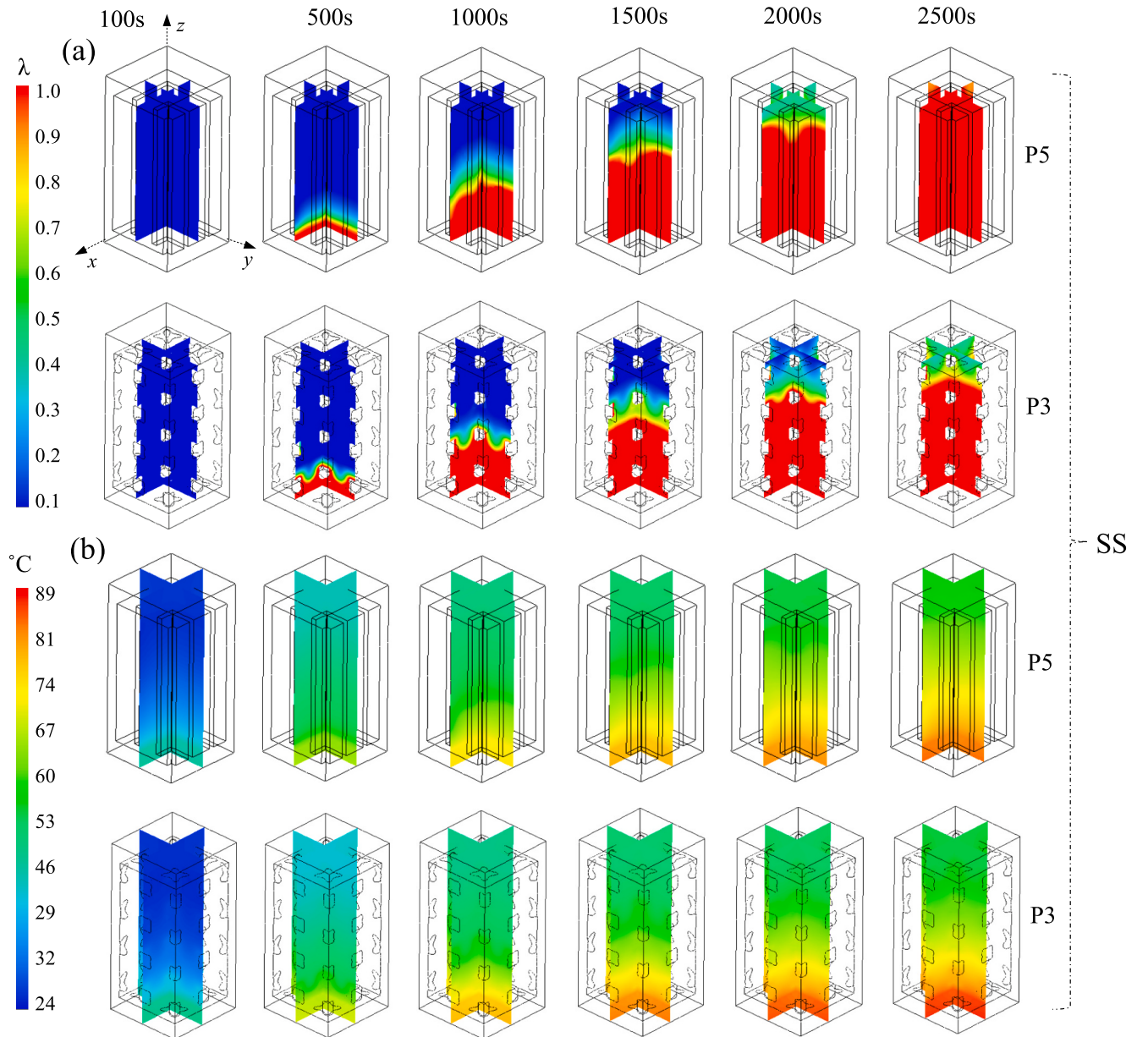
Fig. 9. Effect of base heating (a) liquid fraction; (b) average temperature.
