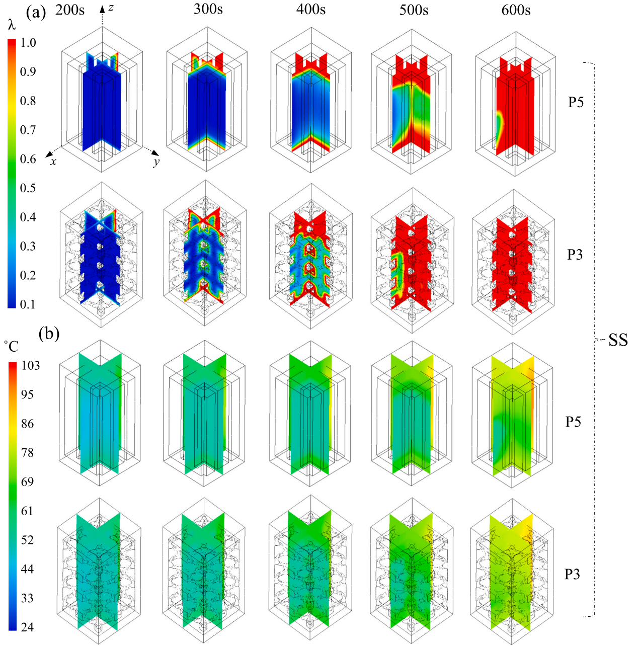
Fig. 12. Effect of side heating (a) liquid fraction; (b) average temperature.
