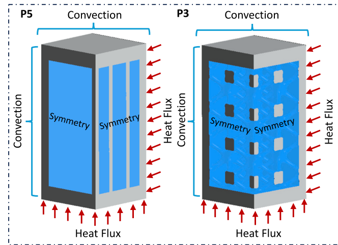
Fig. 14. Initial and boundary conditions for design P5 and P3.
