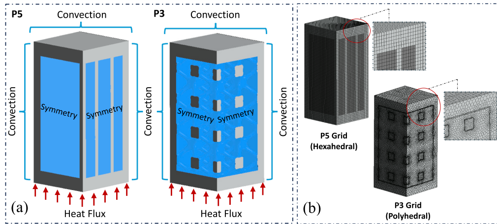
Fig. 8. P3 and P5 simulation models: (a) initial and boundary conditions; (b) computational grids.
