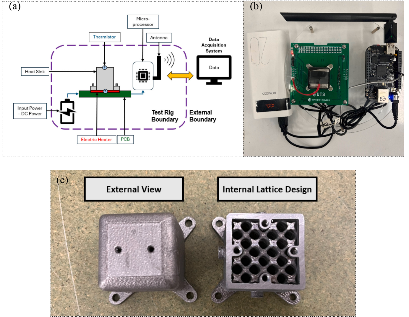
Fig. 4. Experimental set-up (a) 2-D schematic showing different components used in the experiment; (b) picture depicting actual PCB board, battery, sensors and a microprocessor; (c) actual prints of design P3.
