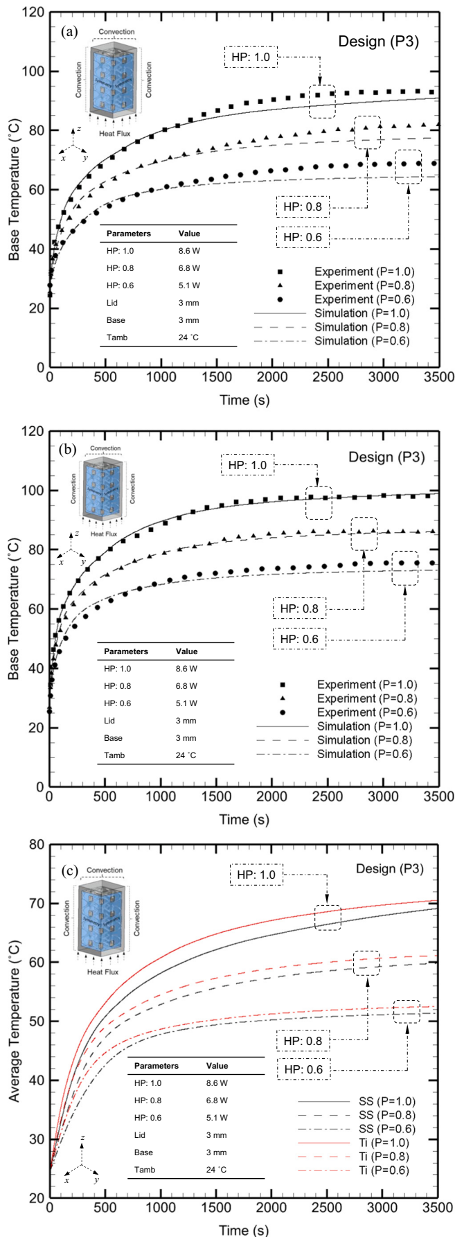
Fig. 5. (a) Base temperature evolution of the stainless-steel heat sink over time; (b) base temperature evolution of the titanium heat sink over time; (c) volume-averaged temperature of the entire heat sink (metal + PCM) for both stainless steel and titanium heat sinks, providing a holistic comparison of thermal performance.
