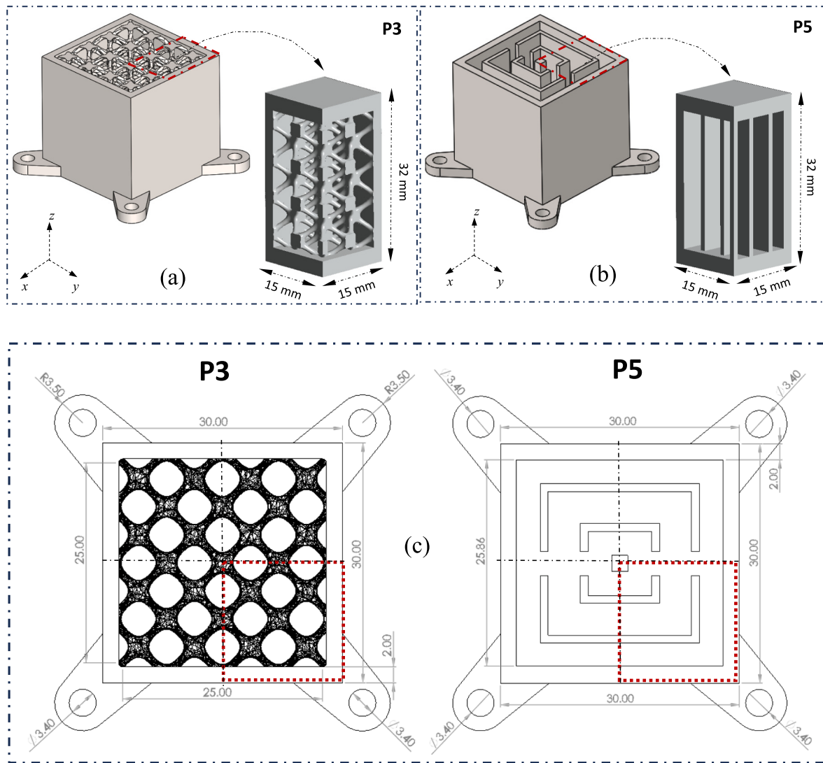
Fig. 1. Schematic diagram of heat sinks (a) CAD model of Design P3; (b) CAD model of Design P5; (c) Dimensions – all in mm.
