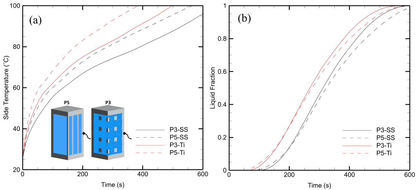
Fig. 13. Effect of side heating (a) side temperature with points of measurement (b) liquid fraction.
