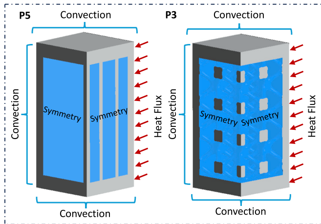
Fig. 11. Initial and boundary conditions for designs P5 and P3.
