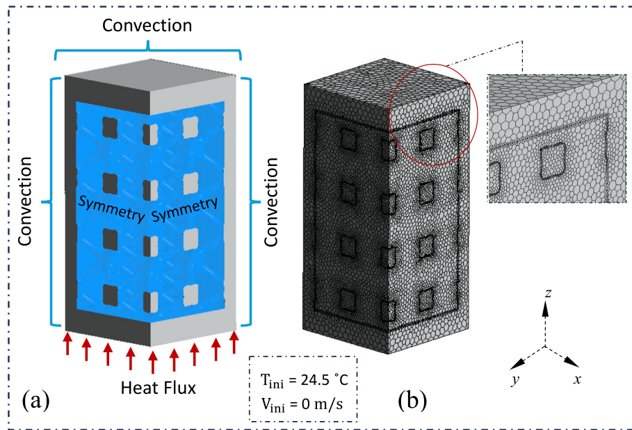
Fig. 2. (a) Initial and boundary conditions; (b) computational grid.
