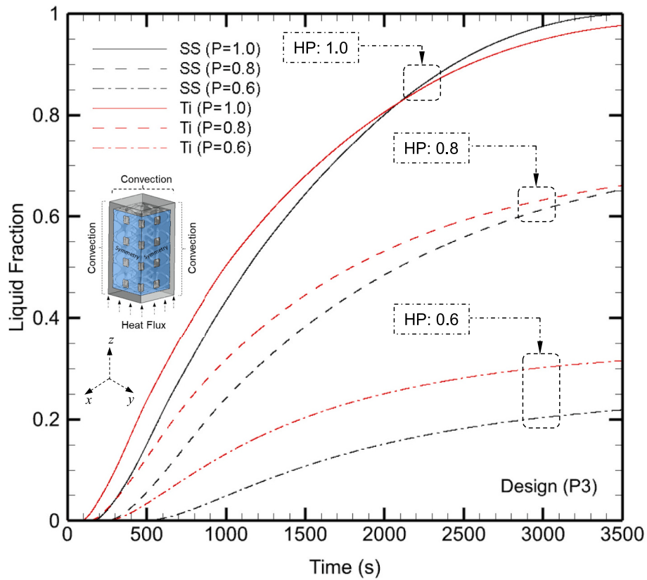
Fig. 7. Liquid fraction of stainless steel and titanium at all heater power inputs.
