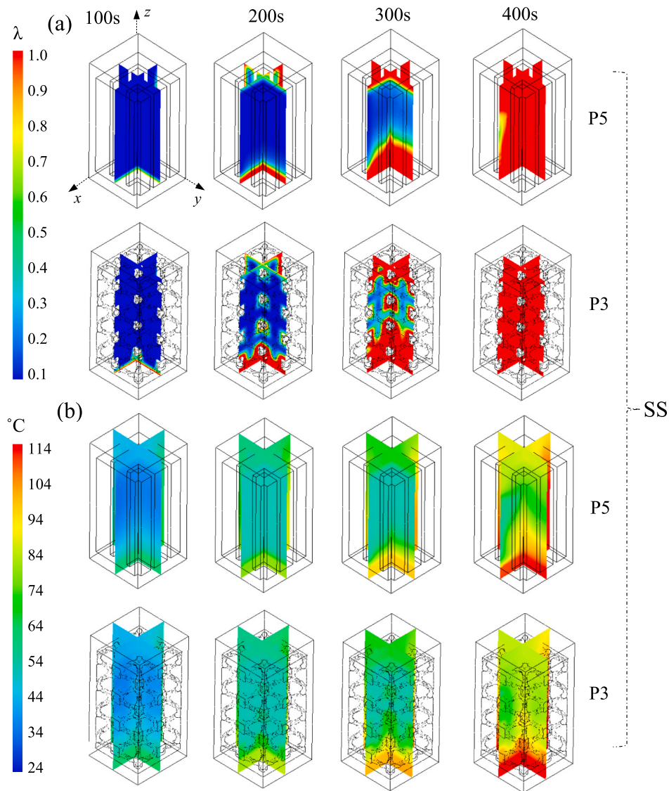
Fig. 15. Effect of base and side heating (a) liquid fraction; (b) average temperature.
