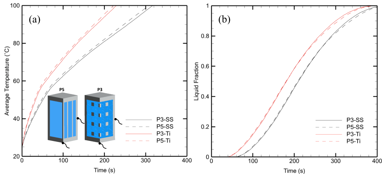
Fig. 16. Effect of base and side heating (a) average temperature of points of measurement; (b) liquid fraction.
