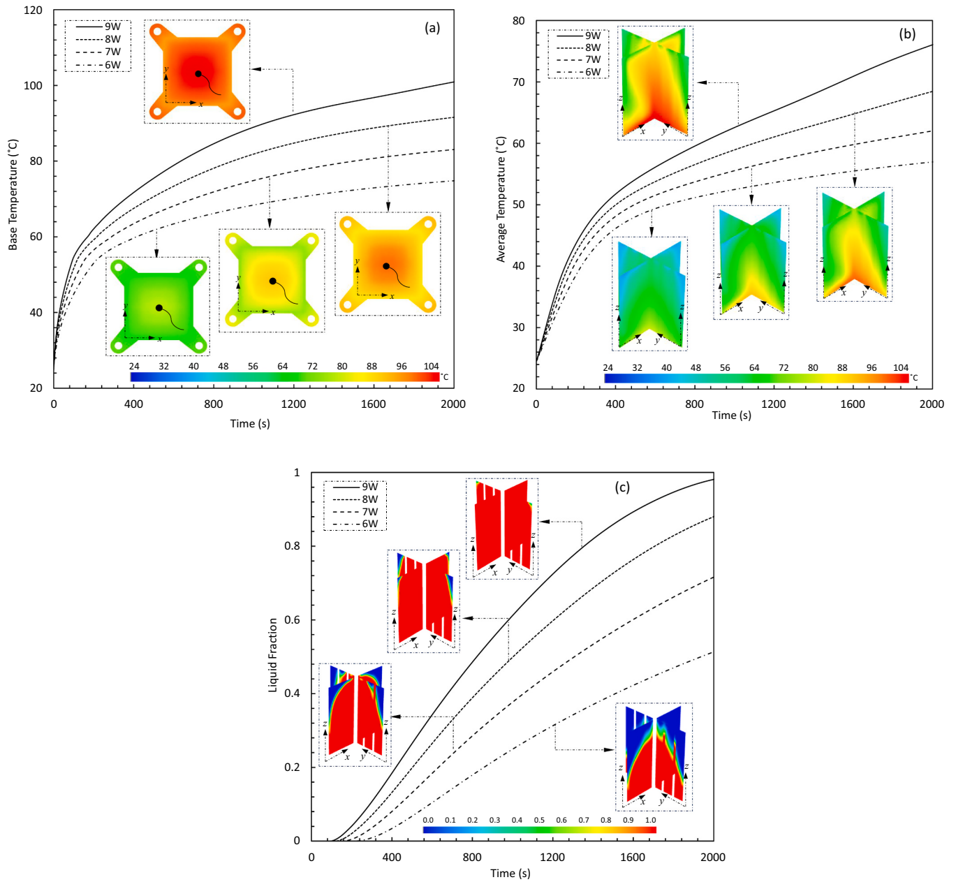
Fig. 8. Effect of power input (a) base temperature; (b) average temperature; (c) liquid fraction.
