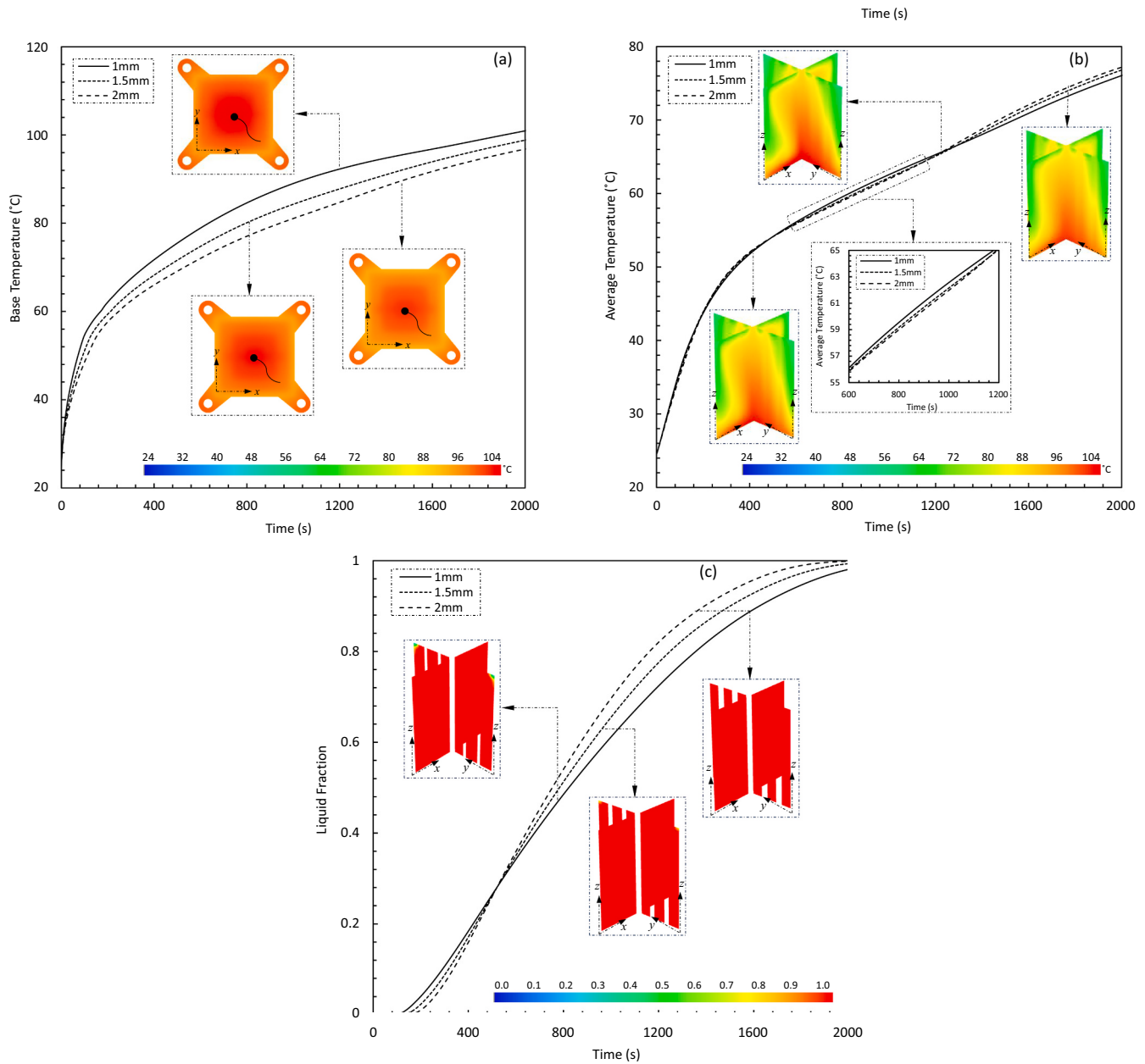
Fig. 11. Effect of fin thickness (a) base temperature; (b) average temperature; (c) liquid fraction.
