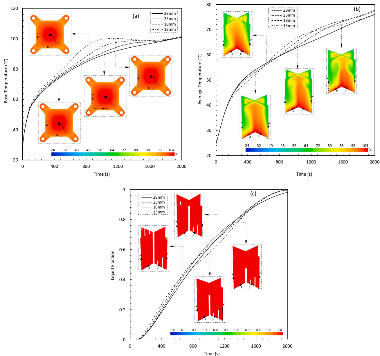
Fig. 12. Effect of fin height (a) base temperature; (b) average temperature; (c) liquid fraction.
