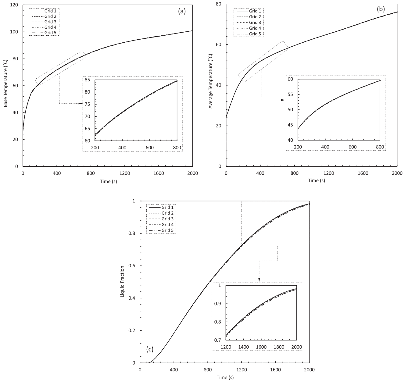
Fig. 3. Grid sensitivity analysis (a) base temperature; (b) average temperature; (c) liquid fraction.
