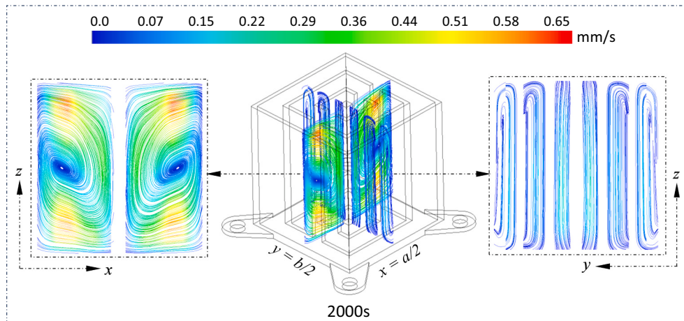
Fig. 7. Velocity streamlines at 2000s.
