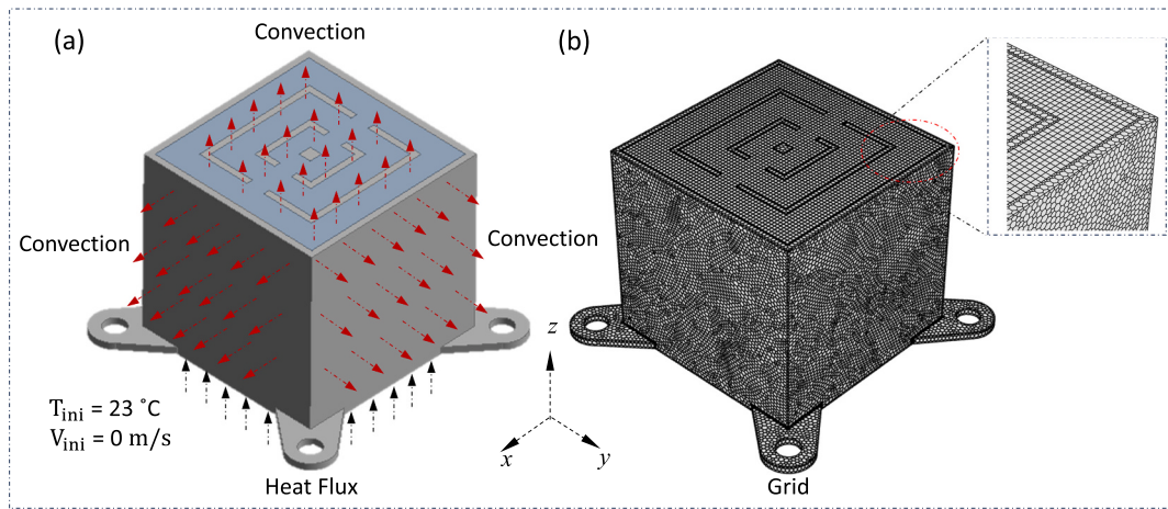
Fig. 2. (a) Initial and boundary conditions; (b) computational grid.
