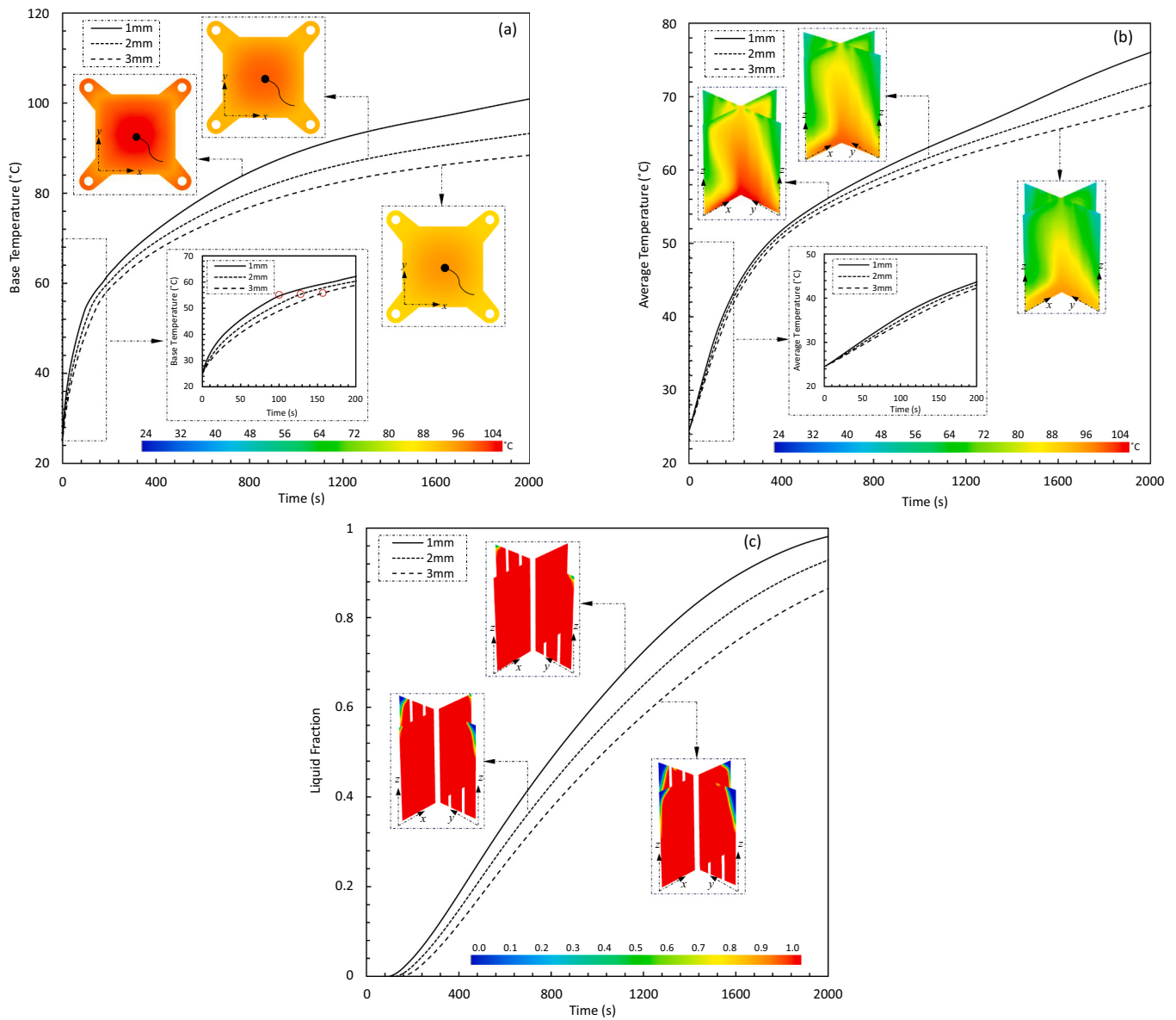
Fig. 10. Effect of base thickness (a) base temperature; (b) average temperature; (c) liquid fraction.
