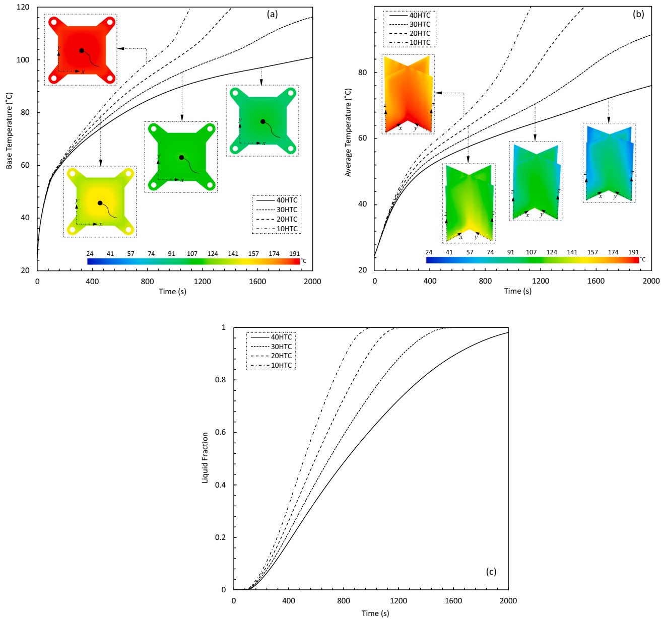
Fig. 9. Effect of convective heat transfer coefficient (a) base temperature; (b) average temperature; (c) liquid fraction.
