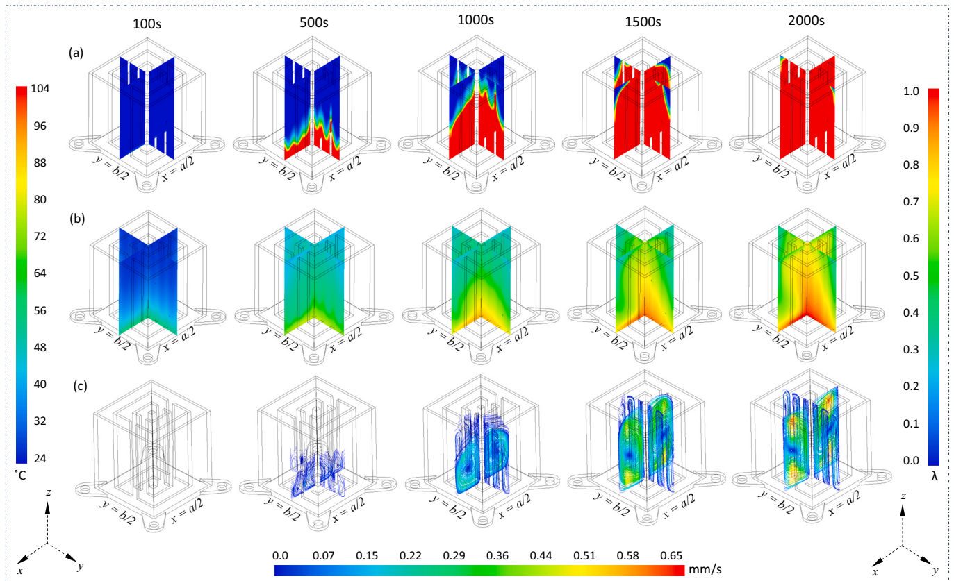
Fig. 6. Transient contours (a) liquid fraction; (b) volume average temperature; (c) velocity streamlines.
