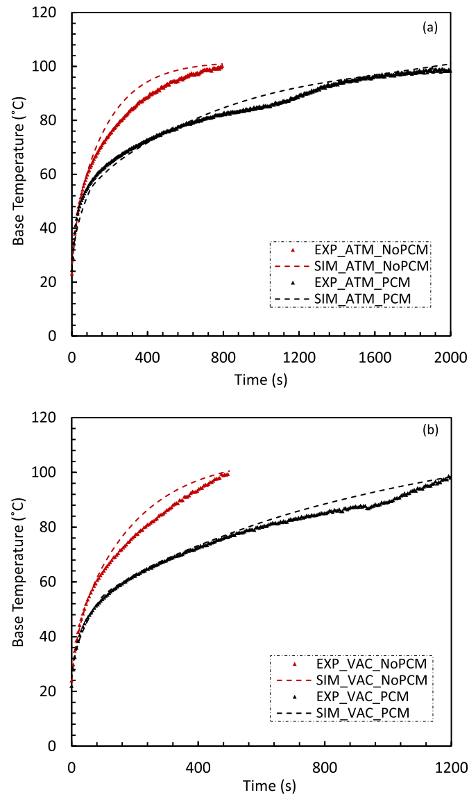
Fig. 5. Experimental validation (a) base temperature (atmosphere); (b) base temperature (vacuum).
