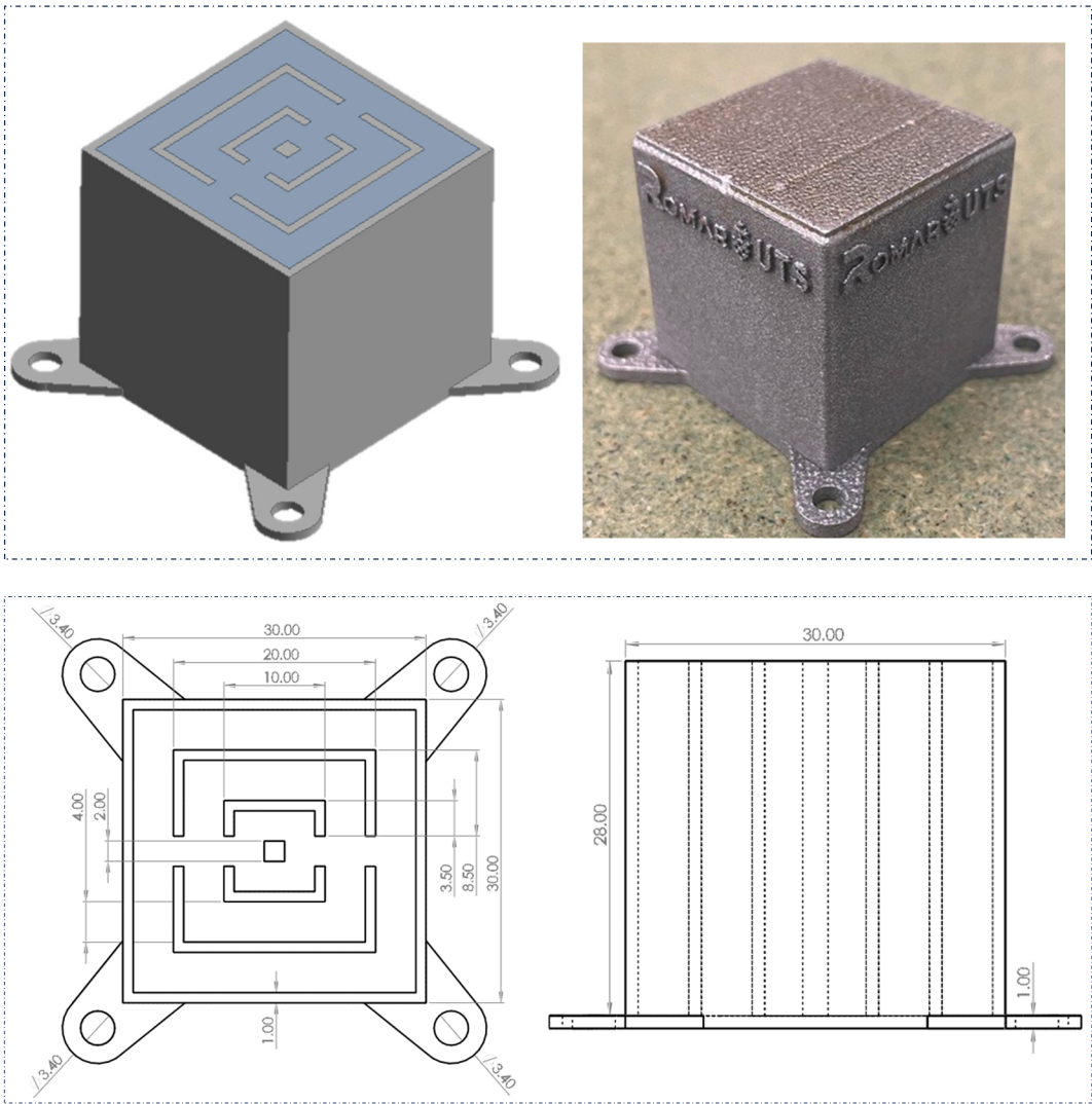
Fig. 1. Schematic diagram of heat sink (a) CAD model (b) 3D printed heat sink (c) heat sink dimensions – all in mm.
