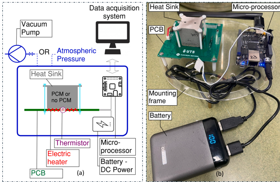
Fig. 4. Experimental set-up (a) schematic; (b) picture.
