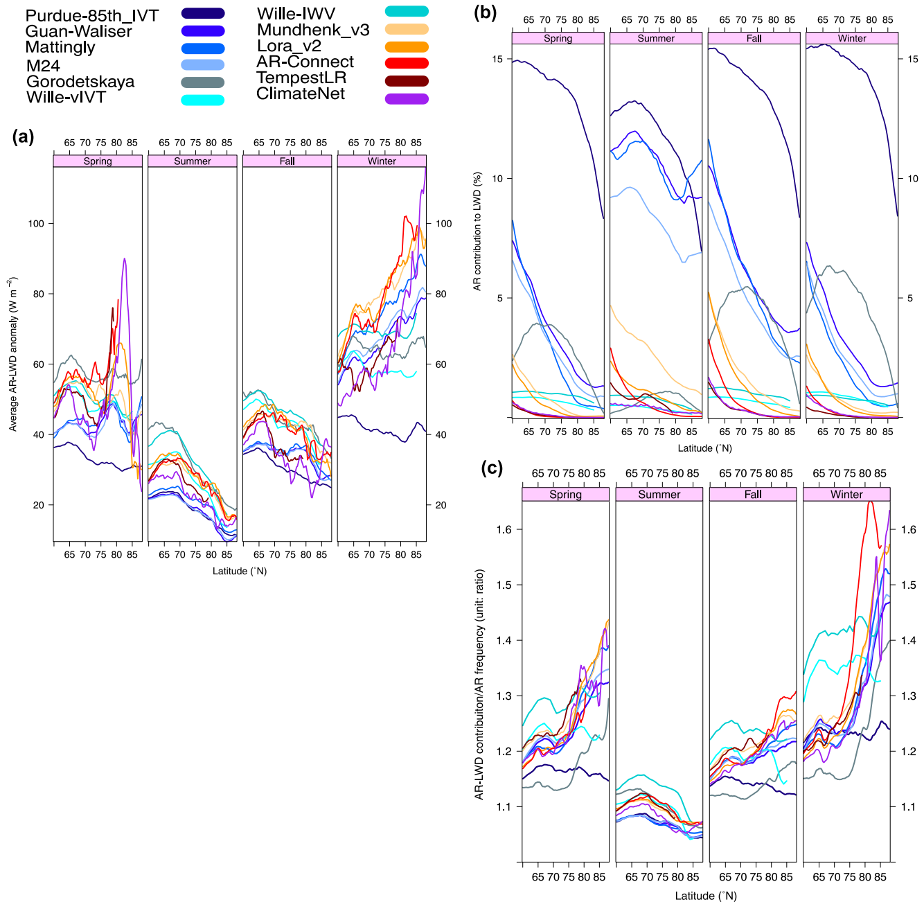
Figure 4. (a) Zonal mean distribution of average LWD anomalies (unit: \text{W m}^{-2} ) during AR occurrences across latitudes from 60°N to 88°N during each season from 2000 to 2019 using 12 ARDTs. (b) Zonal mean distribution of AR contribution to seasonal climatological LWD (unit: %) cross latitudes from 60°N to 88°N during each season from 2000 to 2019 using 12 ARDTs. (c) Zonal mean distribution of the ratio of AR contribution to total LWD (panel (b)) to AR occurrence frequency (Figure 1a) from 60°N to 88°N during each season.
