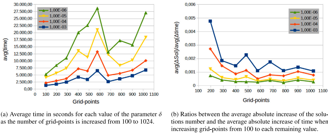
Fig. 3. Representation of data relative to the tuning of AUGMECON-R parameters.
