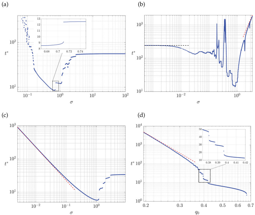
Figure 7. The overturning time, t^* , shown against modulation frequency \sigma , for the governing equation (2.8) with initial condition equation (2.10) and starting profile h_0 . (a) b = 0.3, h_0(\theta) \in \mathcal{H} with \mathcal{Q}_0 = q_0 \Omega_0^{3/2} , q_0 = 0.5 , (b) b = 0.3, h_0 \notin \mathcal{H} solving h_0 - (1/3)h_0^3 \cos \theta = 1/2 , and (c) b = 0.5, h_0 \in \mathcal{H} with \mathcal{Q}_0 = q_0 \Omega_0^{3/2} , q_0 = \sqrt{2}/3 = 0.471 . For (a) the point (b, q_0) = (0.3, 0.5) lies in the white region in figure 10 corresponding to a regular asymptotic solution in the small- \sigma limit (refer to §5b). In (b) the black dashed line indicates the overturning time obtained by integrating equation (5.16) with \Omega_2(T) frozen at \Omega_0 ; the red dashed line shows the curve t^* = 160\sigma^2 , the coefficient having been chosen to obtain a reasonable fit. In (c) the point (b, q_0) = (0.5, 0.471) lies in the blue blow-up region in figure 10, and the red dashed line shows the curve t^* = T_s^* \sigma^{-1} , where T_s^* = 2.270 is computed by integrating equation (5.26) subject to q(0) = \sqrt{2}/3 . (d) The overturning time t^* versus q_0 for b = 0.5 and \sigma = 0.6 . The initial condition is equation (2.10) with h_0 \in \mathcal{H} and \mathcal{Q}_0 = q_0 \Omega_0^{3/2} , where \Omega_0 = \Omega(0) ; the red dashed line shows the curve t^* = 0.27q_0^{-6} , the coefficient having been chosen to obtain a reasonable fit.
