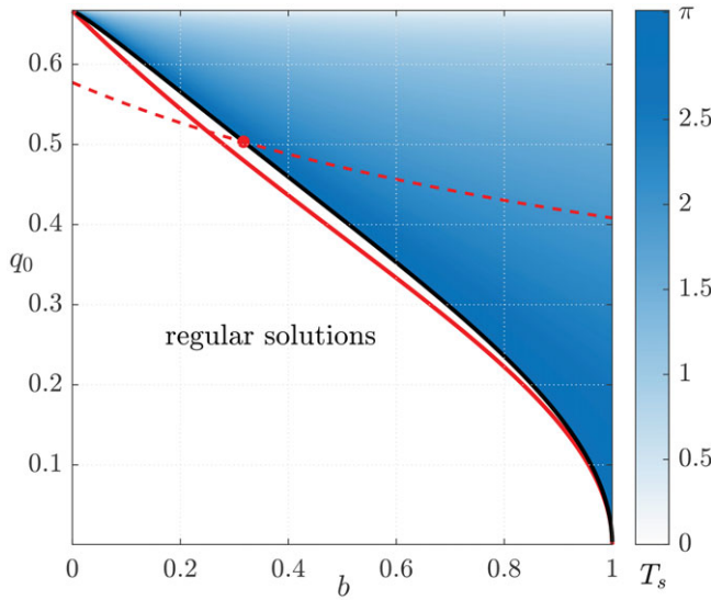
Figure 10. Regularity map for q(T) solving equation (5.26) in the limit \sigma \rightarrow 0 . The black curve delineates the boundary q^*(b) between regular behaviour ( q(T) periodic in T ) and blow-up behaviour ( q(T) \rightarrow 2/3 as T \rightarrow T_s ). The red curve shows the approximation to the q^*(b) boundary given in equation (5.36). The dashed red line shows 1/q_0 = \sqrt{3(1+b)} , whose intersection with the black line at b = 0.317 , shown with a red marker point, determines the location of the red marker point in figure 4.
