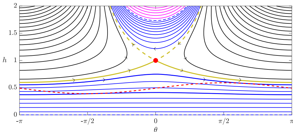
Figure 2. One period, \theta \in [-\pi, \pi) , of the phase portrait for the system equation (3.3) corresponding to the steady MP problem with \Omega = 1 ( b = 0 ). Each trajectory is described by equation (3.2) and corresponds to a particular value of Q . Black lines show Q > 2/3 , blue lines show 0 < Q < 2/3 , and magenta lines show Q < 0 . The blue dashed lines indicate Q = 0 . The separatrix, shown with a thick gold line (both solid and dashed), corresponds to Q = Q^* = 2/3 ; the solid part delineates the boundary between regular solutions to the characteristic equations (3.3) and those exhibiting finite-time blow-up. The minimum value of h along the separatrix occurs at \theta = \pm\pi and is h_{\min} = p^{1/3} - 1/p^{1/3} \approx 0.5961 , where p = 1 + \sqrt{2} . The red dots indicate the location of the saddle points for equation (3.3) , and the arrows on the trajectories indicate the direction of travel as \tau increases. The broken red line indicates a typical initial film profile, H(\theta) , bounded by envelope trajectories shown with thick blue lines.
