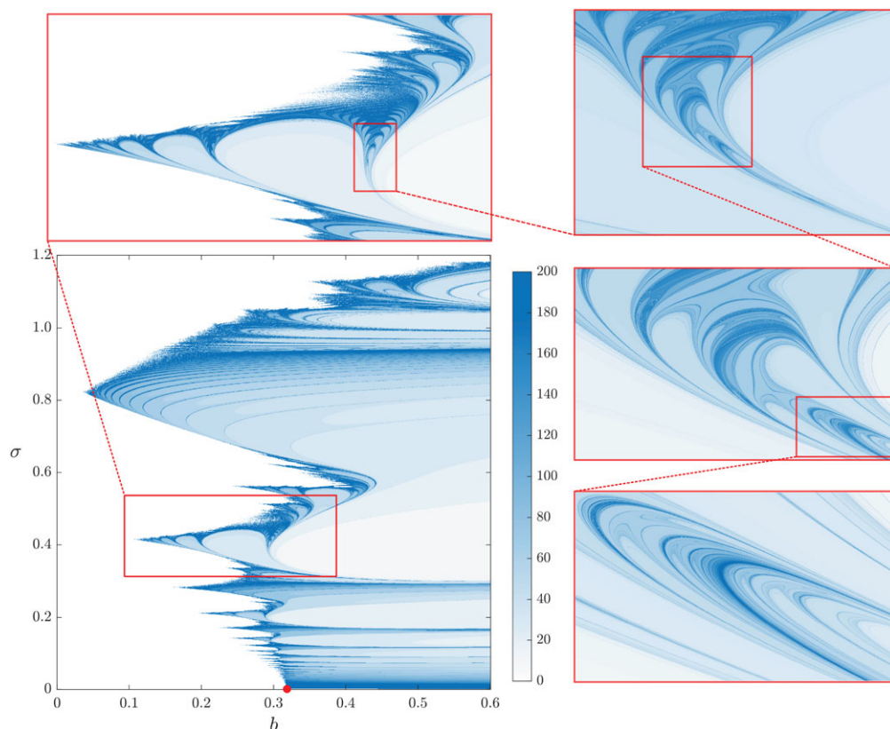
Figure 4. The blow-up map obtained by integrating the characteristic equations (3.3) with the initial condition equation (4.3) taking h^* = 1/\sqrt{3} , with \Omega(t) given by equation (2.7). Points in the b\sigma -plane are coloured white if the solution remains bounded occurs and blue if blow-up occurs. The shade of blue is determined by the time at which blow-up occurs indicated in the colour bar: darker blue corresponds to later blow-up times. Here blow-up is deemed to have occurred when h = 5.0 is reached. The red marker point at (\sigma, b) = (0, 0.317) indicates the predicted blow-up threshold from the small- \sigma analysis of §5b.
