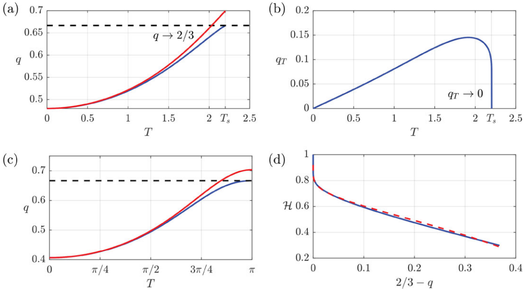
Figure 9. (a,b) Numerical solution of equation (5.26) (solid blue curves) for q(0) = 0.48 and b = 0.5 . The integration is stopped at T = T_s where q(T_s) = 2/3 . In this case T_s = 2.2 . The solid red curve shows the approximate q(T) given in equation (5.35). (c) Numerical solution of equation (5.26) (solid blue curve) for b = 0.5 and q(0) = q^*(0.5) \approx 0.4063 , with the approximate solution equation (5.35) shown with a red curve. (d) Comparison between \mathcal{H} as defined in equation (5.27), shown with a blue solid line, and the approximation for \mathcal{H} valid as q \rightarrow 2/3 given by equation (5.30), shown with a red dashed line.
