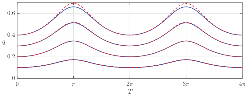
Figure 11. Numerical integration (blue curves) of equation (5.26) for b = 0.5 and q(0) = 0.1, 0.2, 0.3, 0.4 (bottom to top). The dashed red lines show the approximation equation (5.35). In this case q^*(0.5) = 0.4063 .
