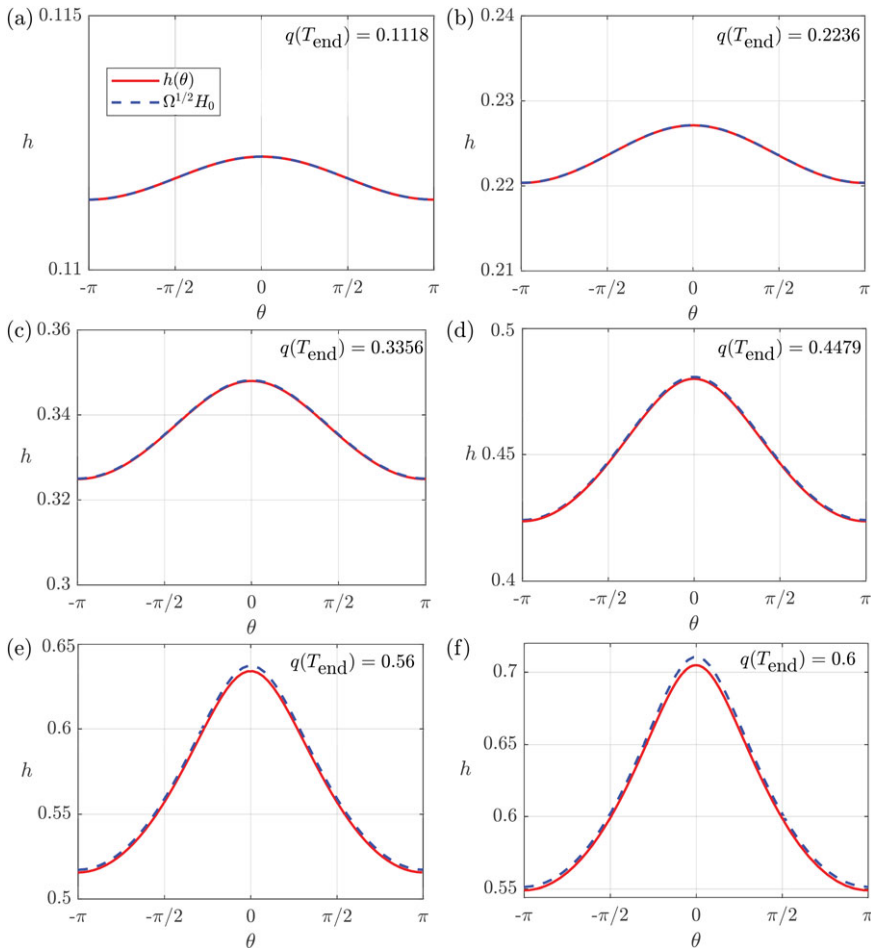
Figure 12. Film profiles (solid red curves) obtained by integrating equation (2.8) numerically up to t_{\text{end}} = T_{\text{end}}/\sigma = 2000/\sigma for the case b = 0.25 and \sigma = 0.01 . The initial condition is equation (2.10) with h_0 \in \mathcal{H} and Q_0 = q_0 \Omega_0^{3/2} where \Omega_0 = \Omega(0) = 1 + b and (a) q_0 = 0.1 , (b) q_0 = 0.2 , (c) q_0 = 0.3 , (d) q_0 = 0.4 , (e) q_0 = 0.5 , and (f) q_0 = 0.5385 . For panel (f) q_0 is very close to the critical value q^*(0.25) \approx 0.538725 . The dashed blue lines show \Omega^{1/2}H_0 , where H_0 is the leading-order solution in the small- \sigma analysis of §5b, satisfying equation (5.18) with q(0) = q_0 and using the approximate solution equation (5.35) for q(T) .
