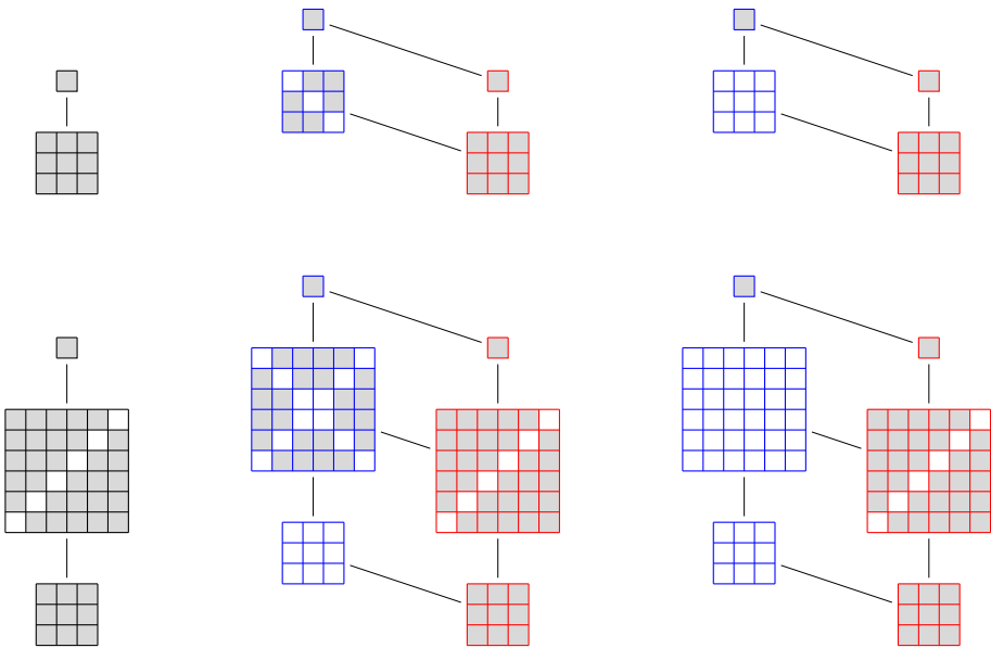
Fig. 5. Egg-box diagrams of the Brauer monoids \mathcal{B}_3 (top row) and \mathcal{B}_4 (bottom row), and two each of their twisted products. See Remark 5.3 for more details.
