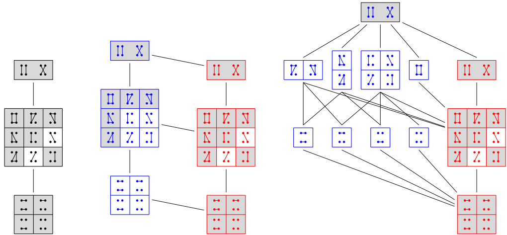
Fig. 3. Egg-box diagrams of the partition monoid \mathcal{P}_2 , and two of its twisted products. See Remark 5.3 for more details.
