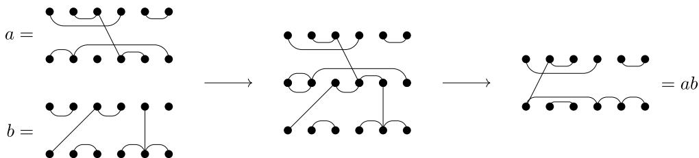
Fig. 2. Multiplication of partitions a, b \in \mathcal{P}_6 , with the product graph \Pi(a, b) in the middle.
