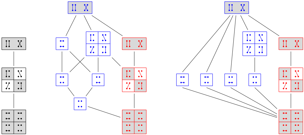
Fig. 4. Egg-box diagrams of the partial Brauer monoid \mathcal{PB}_2 , and two of its twisted products. See Remark 5.3 for more details.
