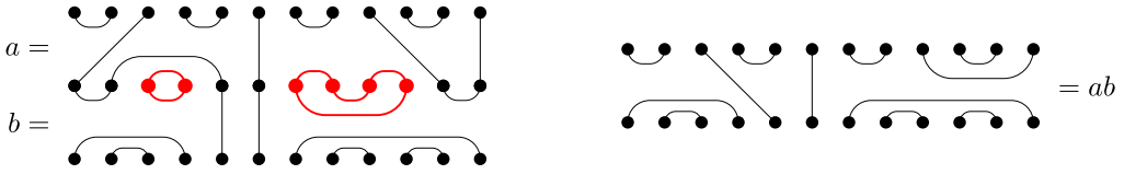
Fig. 1. Stacking Temperley–Lieb diagrams a and b (left). Here there are two floating loops (shown in red), so \Phi(a, b) = 2 . Removing these components leads to the product ab (right). (For interpretation of the colours in the figure(s), the reader is referred to the web version of this article.)
