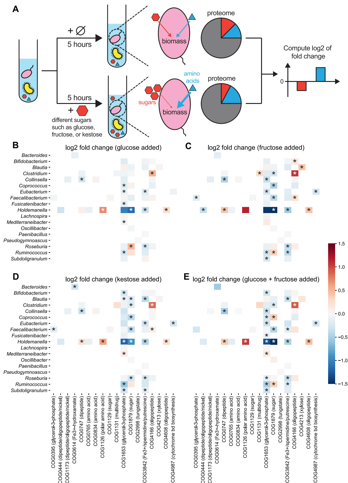
Figure 6. Microbes modify their expression for ABC-type transporters to adapt to added sugars; all heatmaps share the same color bar on the right; (A) schematic of in vitro cultures of a collected human gut microbiome; in the treatment group, one sugar is added to the community; metaproteomic measurements 5 h later were used to compare the intensity of each taxon-specific protein using the log2 fold change of each protein's fraction (i.e. normalized intensity over each genus) from the treatment group divided by that from the control group; Log2 fold changes of ABC-type transporters were computed 5 h after (B) glucose, (C) fructose, (D) kestose, or (E) glucose and fructose is added; the transported metabolites for each COG are added to the brackets.
