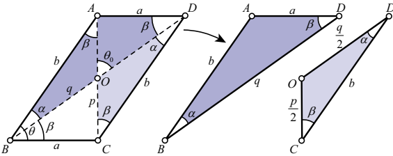
Figure 1: A (\theta, \theta_0) -parallelogram with an interior angle \theta and an diagonal angle \theta_0 . If \theta = \theta_0 , it is a \theta -parallelogram, which possesses two similar triangles \triangle ABD \approx \triangle ODC with equal edge ratios a : b : q = \frac{p}{2} : \frac{q}{2} : b .
