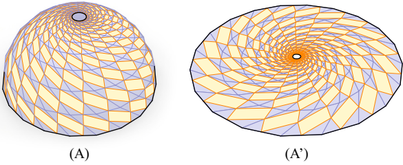
Figure 10: (A) From Fig. 9-(B), an I-net with similar parallelograms covers part of a unit sphere. (A') Under stereographic projection, it is mapped to the plane, preserving the angles of all similar parallelograms.
