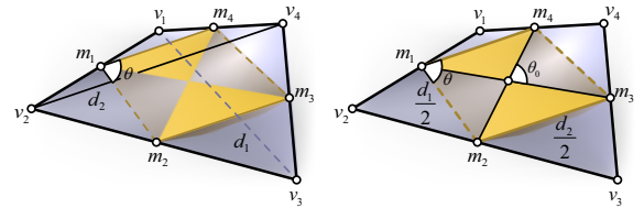
Figure 4: Mid-edge subdivided parallelogram within a general spatial (\theta, \theta_0) -quad. The interior angle \theta and the diagonal angle \theta_0 of the parallelogram are functions of the ratio \lambda of the diagonal lengths and the ratio \mu of the medial-line lengths of the quad. The quad is referred to as a \theta -quad, if the parallelogram is a \theta -parallelogram, where the angles \theta = \theta_0 .
