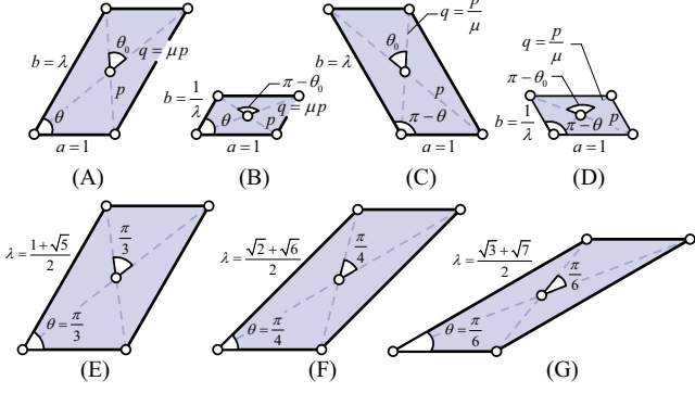
Figure 2: (A–D) (\theta, \theta_0) -parallelograms with different edge ratios ( b : a, q : p ): (A) (\lambda, \mu) , (B) (\frac{1}{\lambda}, \mu) , (C) (\lambda, \frac{1}{\mu}) , (D) (\frac{1}{\lambda}, \frac{1}{\mu}) . (E–G) \theta -parallelograms with \theta = \frac{\pi}{3}, \frac{\pi}{4} , and \frac{\pi}{6} , respectively.
