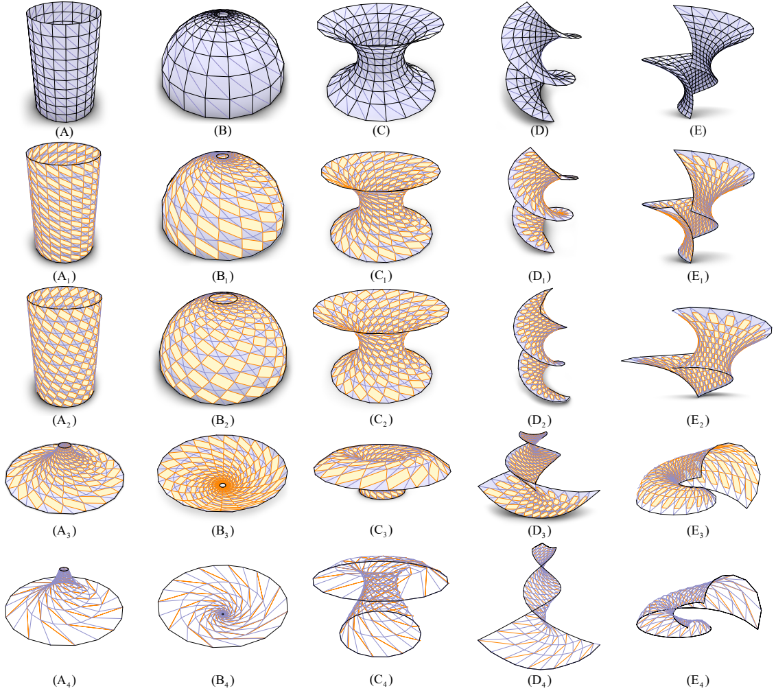
Figure 9: (A_1 - E_1) I-nets with similar inscribed parallelograms, characterized by angles (\theta, \theta_0) = (\arccos \frac{1}{\sqrt{5}}, \frac{\pi}{4}) can be extracted from the isothermal parametrization on surfaces. Examples include (A) a cylinder, (B) a sphere, (C) a catenoid, (D) a helicoid, and (E) a conjugate minimal surface combined by catenoid and helicoid. These I-nets can be further optimized to have (\theta, \theta_0) = (\frac{4\pi}{9}, \frac{\pi}{4}) in (A_2 - E_2) , approximating the corresponding surfaces. Alternatively, they can be transformed conformally under Möbius transformations to new surface shapes in (A_3 - E_3) , and then optimized to have \theta = \theta_0 = \frac{5\pi}{18} approximated on the surfaces in (A_4 - E_4) . The Hausdorff distances between the meshes in (A_4 - E_4) and the underlying subdivided meshes in (A_3 - E_3) are 1.959, 0.016, 38.593, 3.120 and 9.464, respectively, relative to their corresponding diagonal lengths of the bounding boxes.
