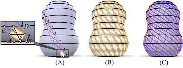
Figure 11: On a general surface of revolution, an I-web is constructed using three families of loxodromes and the parallel circles. (A) The process begins with two neighboring loxodromes that form a constant angle \frac{\pi}{2} - \theta_0 with the meridians and intersect a parallel circle at points A and B . Two neighboring points C and D on the loxodromes are computed to satisfy Eq. (16). Subsequently, a strip of quads with similar inscribed (\theta, \theta_0) -parallelograms is modeled using the propagation algorithm outlined in Alg. 1. By uniformly rotating around the axis, an I-net covering the rotational surface with congruent strips is constructed and its discretization can be extracted in (B). (C) The two families of diagonal curves create non-trivial isogonal curve patterns and are also loxodromes with angles related to \lambda and \mu . Loxodromes and parallel circles form an isogonal 4-web. Multiple I-nets with different similar parallelograms can be extracted.
