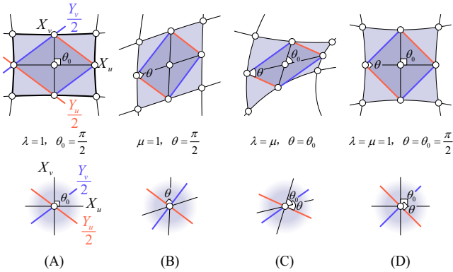
Figure 6: Special cases for I-net and I-web based on the representation of similar parallelograms in the CBP. (A) \lambda = 1 \Leftrightarrow \theta_0 = \frac{\pi}{2} . I-net with similar rhombuses becomes O-net. (B) \mu = 1 \Leftrightarrow \theta = \frac{\pi}{2} . I-net with similar rectangles. (C) \lambda = \mu \Leftrightarrow \theta = \theta_0 . I-net with similar \theta -parallelgrams. \mathbf{X}(u, v) and \mathbf{Y}(u, v) are aligned through rotation. (D) \lambda = \mu = 1 \Leftrightarrow \theta = \theta_0 = \frac{\pi}{2} . O-net with similar squares. \mathbf{X}(u, v) is locally equivalent to \mathbf{Y}(u, v) after a \frac{\pi}{4} rotation.
