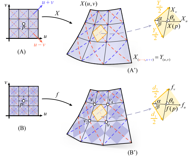
Figure 5: Top: A smooth parametrization \mathbf{X}(u, v) and its diagonal parametrization \mathbf{Y}(u, v) = \mathbf{X}(u - v, u + v) form an I-web when \frac{\|\mathbf{X}_u\|}{\|\mathbf{X}_v\|} and \frac{\|\mathbf{Y}_u\|}{\|\mathbf{Y}_v\|} are constant. Down: Discrete derivative mapping from a regular triangulated grid as parameter domain to a triangle mesh. Discrete derivatives f_u and f_v approximate the second-order smooth derivatives, while \mathbf{d}_1 and \mathbf{d}_2 approximate the first-order smooth derivatives. These discrete derivatives have constant angles between them and form a DI-web.
