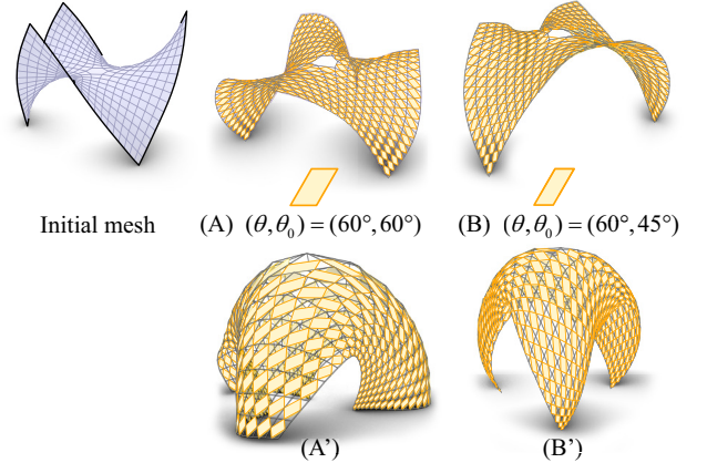
Figure 13: A quad mesh with a singular face at the center is optimized to (A) a DI-net with \theta = \theta_0 = \frac{\pi}{3} and (B) a DI-net with (\theta, \theta_0) = (\frac{\pi}{3}, \frac{\pi}{4}) , respectively. (A'–B') show their corresponding Möbius transformations, preserving the geometric connectivity.
