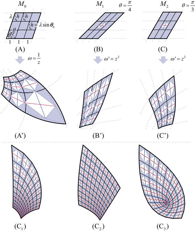
Figure 3: (A–C) Regular sheared grids M_0, M_1 and M_2 with congruent parallelograms in the upper half-plane mapped from rectangular grids. (B) Sheared grid M_1 with \theta_0 = \theta = \frac{\pi}{4} . (C) Sheared grid M_2 with \theta_0 = \theta = \frac{\pi}{3} . Conformal mappings of these grids: (A') The mapping \omega = \frac{1}{z} transforms the straight lines of M_0 into circular arcs. (B'–C') The mapping \omega' = z^2 transforms M_1 and M_2 into curvilinear grids of parabolas. A ten by ten sheared grid with \theta_0 = \theta = \frac{\pi}{3} is mapped to: (C 1 ) under \omega = \frac{1}{z} , (C 2 ) and (C 3 ) under \omega' = z^2 , forming CBPs with similar \frac{\pi}{3} -parallellograms. The difference between (C 2 ) and (C 3 ) is that the origin lies within the pre-image of the sheared grid for (C 3 ).
