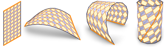
Figure 7: I-nets on developable surfaces are isometric to each other and can be bended from a planar sheared grid with congruent parallelograms continuously to a rotational cylinder. The geodesic curve, which is a straight line in the plane, transforms into a helix on its corresponding rotational cylinder.
