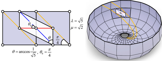
Figure 8: Left: Two parallel diagonals and two parallel edges of two neighboring squares form a parallelogram, whose mid-edge subdivided parallelogram has (\theta, \theta_0) = (\arccos \frac{1}{\sqrt{5}}, \frac{\pi}{4}) and (\lambda, \mu) = (\sqrt{5}, \sqrt{2}) . Right: I-net characterized by these similar parallelograms can be generated from an isothermal net.
