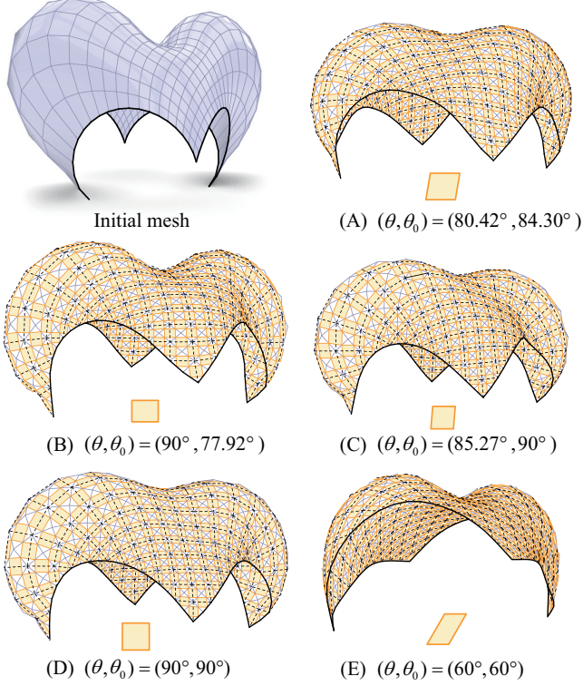
Figure 12: Starting from a general patch, various freeform shapes are designed and covered by I-webs and similar parallelograms. (A) Direct optimization of the initial mesh to an isogonal net results in a general DI-net with similar parallelograms. (B–E) The optimized DI-nets with prescribed angles \theta or \theta_0 lead to special cases of inscribed parallelograms: (B) rectangles, (C) rhombuses, (D) squares, and (E) parallelograms with \theta = \theta_0 = \frac{\pi}{3} . Computational details are provided in Tab. 1.
