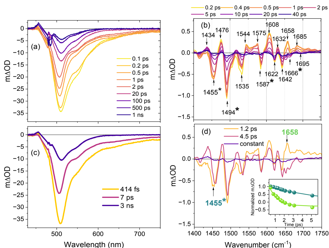
Figure 3 (a) Transient absorption spectra of Kohinoor obtained by 465 nm pump pulse excitation of the off-state ( \text{trans}^- ) in \text{H}_2\text{O} ; oscillations below 500 nm arise from pump pulse scatter. (b) TRIR spectra recorded after excitation of the off-state at 475 nm in \text{D}_2\text{O} . The asterisk marks bleach modes that are mainly associated with the chromophore - see text. (c) EADS obtained from the global analysis of the TA data using the sum of two decay components (assuming a sequential kinetic model) and a fixed 3 ns final component and (d) EADS obtained by global analysis of the TRIR data using the same model as (c) with a constant final component; note
