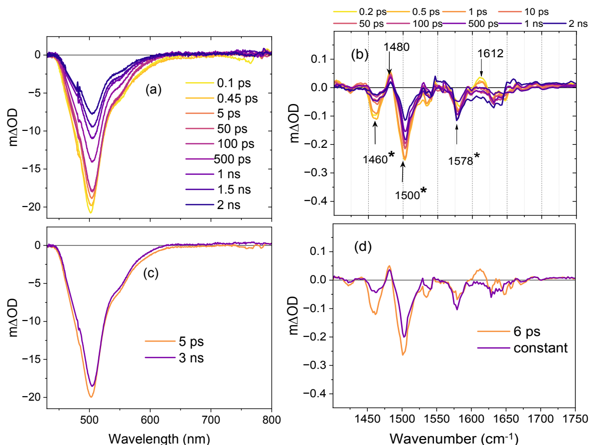
Figure 5 (a) Transient absorption spectra of Kohinoor obtained by 475 nm excitation of the on-state ( \text{cis}^- ) in \text{H}_2\text{O} . Data are presented out to 2 ns to reflect the slower relaxation of the dominant emissive \text{cis}^- state. (b) TRIR spectra recorded after excitation of the on-state at 475 nm in \text{D}_2\text{O} . The asterisk marks bleach modes that are
