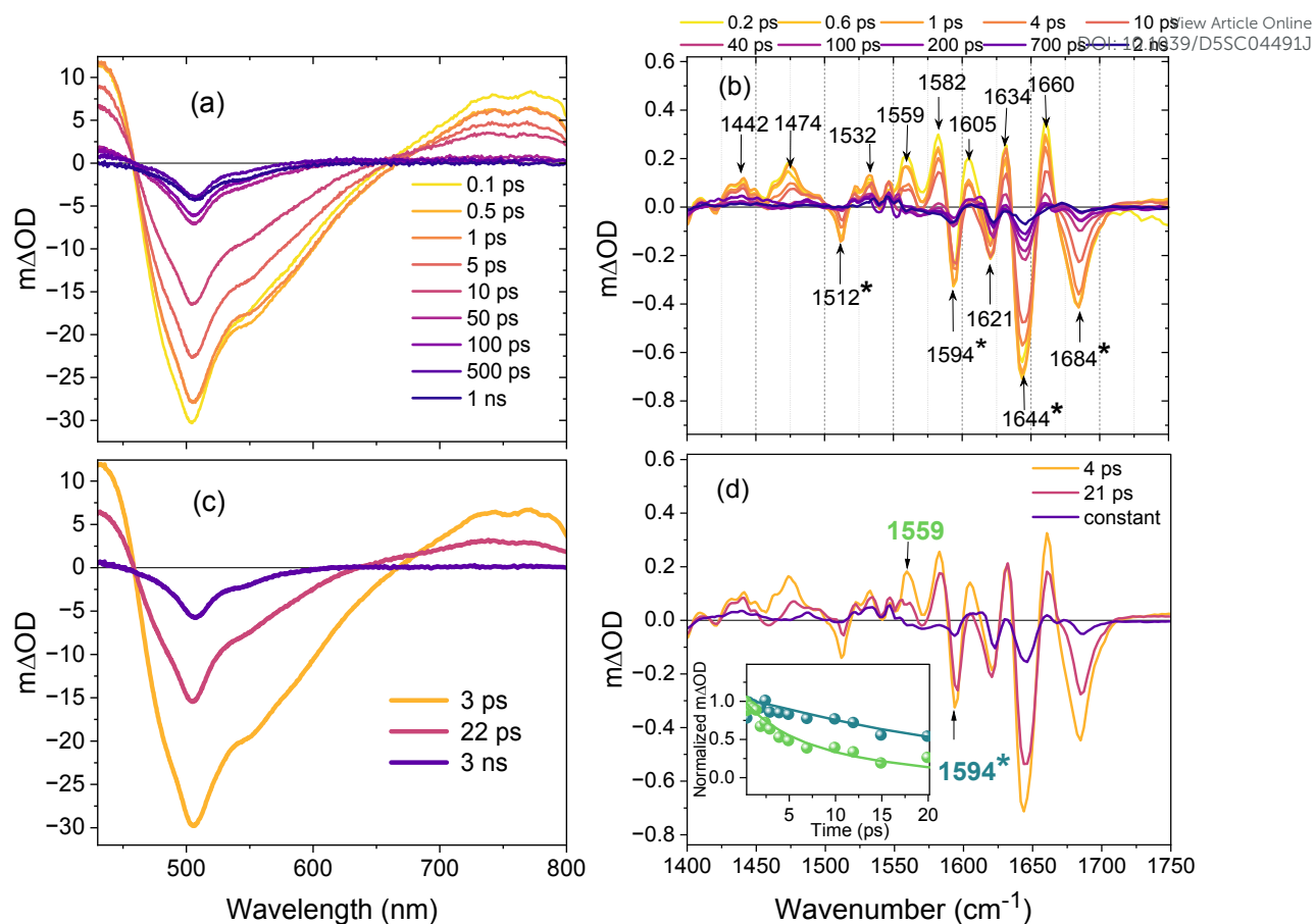
Figure 4 (a) Transient absorption spectra of Kohinoor obtained by 400 nm pump pulse excitation of the on-state (cisH) in H 2 O (b) TRIR spectra recorded after excitation of the on-state at 380 nm in D 2 O. The asterisk marks bleach modes that are mainly associated with the chromophore - see text. The fit lines are from the global analysis to the entire data set. (c) EADS obtained from the global analysis of the TA data using the sum of two decay components (assuming sequential kinetic model) and a 3 ns decay (d) EADS obtained by global analysis of TRIR data. The inset shows intensity normalized temporal evolution of modes identified as protein and chromophore (*) to highlight their different relaxation times. The solid lines are from the global fit. The samples were measured in a flow cell and the reservoir was continuously irradiated with a 505 nm LED to maintain the on-state
