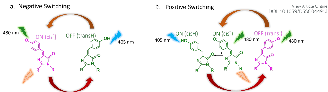
Figure 1: Isomeric form and protonation state for rsFP between on (pink) and off (green) states. (a) The two-state negative switching rsFPs exemplified by Dronpa contrasted with (b) the three state positive photoswitching rsFPs of the Padron type.
