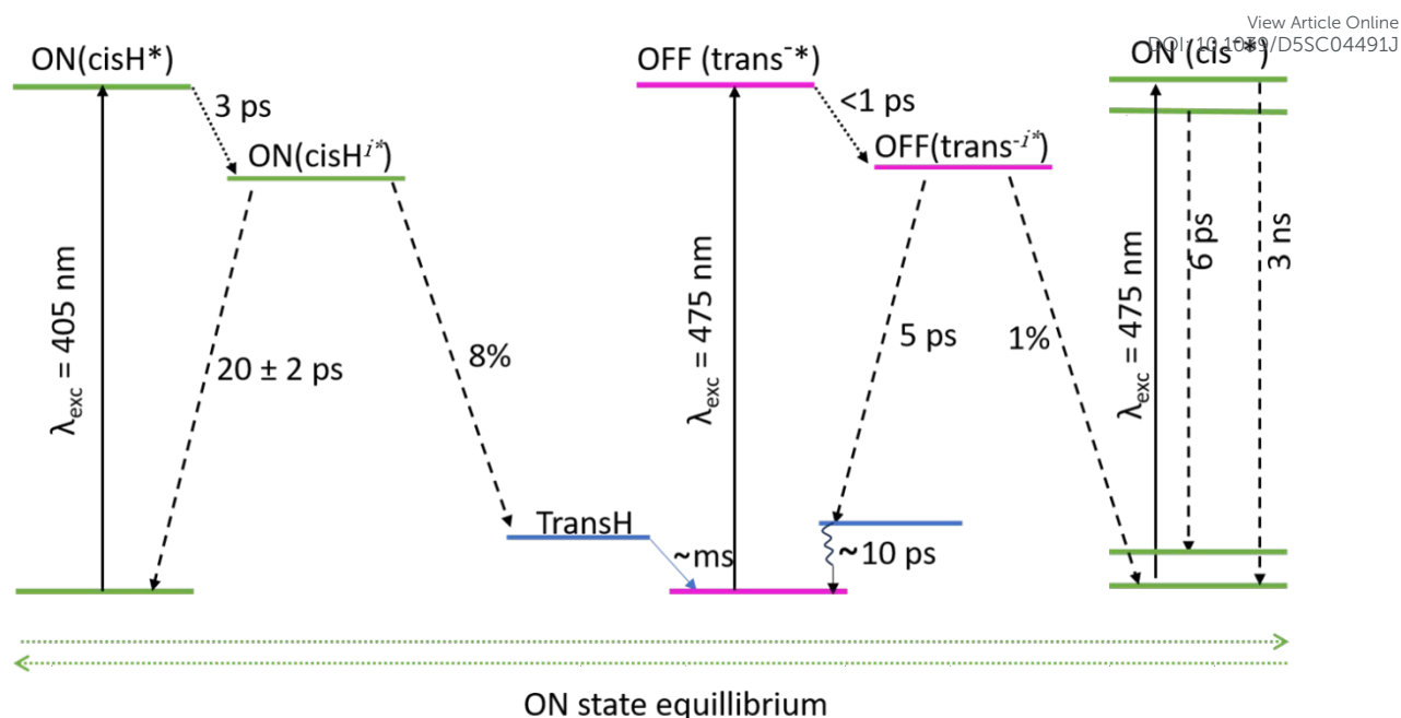
Figure 6 Overview of the phototransformation process in the three states of Kohinoor. Dotted arrows represent relaxation pathways of the chromophore from the Franck-Condon state (denoted by the superscript *), leading to the formation of intermediate states (denoted by the superscript i ). Dashed arrows depict the subsequent relaxation of these intermediate excited states to the ground state(s). Excitation of the cisH forms an intermediate state within ca. 3 ps, which predominantly decays to refill the ground state in ca. 20 ps. A minor fraction (8%) proceeds to populate the transH state, which subsequently forms the trans - on a millisecond timescale. In the off-state, following excitation of trans - an intermediate is formed in <1 ps and primarily (99%) relaxes to a hot-ground state within in ca. 5 ps, which then relaxes over tens of picoseconds (Figure S6) to recover the original state (indicated by the curly arrow). The excited fluorescent on-state (cis - ) undergoes an inhomogeneous decay, involving both a rapid (6 ps) excited-state decay and a long-lived fluorescent pathway (3 ns).
