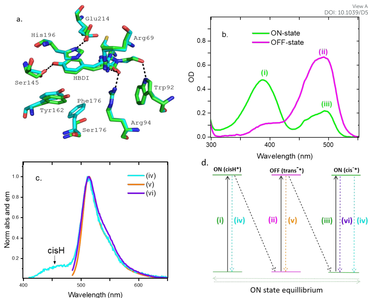
Figure 2 (a) Structure of Kohinoor (cyan) in its on-state (pdb 9DVE) compared with Padron0.9, pdb 3ZUJ (green). The amino acid numbers correspond to Padron. (b) Steady state absorption spectra of the on (cisH/cis - equilibrium) and off (trans - )-states normalised to protein absorbance at 280 nm (c) Peak normalized steady state emission spectra of the on excited at 480 (cis - , purple) and 400 nm (mainly cisH, cyan) and the off (480 nm, mainly trans - , brown) states of Kohinoor in water (d) A level scheme showing the electronic states of the chromophore accessed in Kohinoor and marking the absorption (2b) and emission (2c) transitions between them. Dynamics following each excitation transition are discussed in turn in the following sections, which will establish that each chromophore level structure shown must be adapted to include their specific interactions with the protein.
