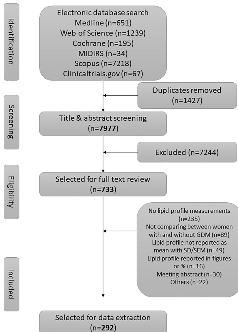
Fig. 1. PRISMA flow chart of selection of studies.
