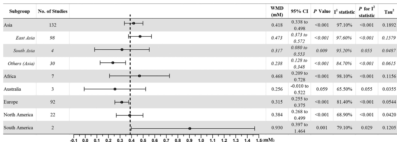
Fig. 2. Forest plot of comparison: Circulating triglyceride levels in women with gestational diabetes mellitus versus control subjects (mM).
