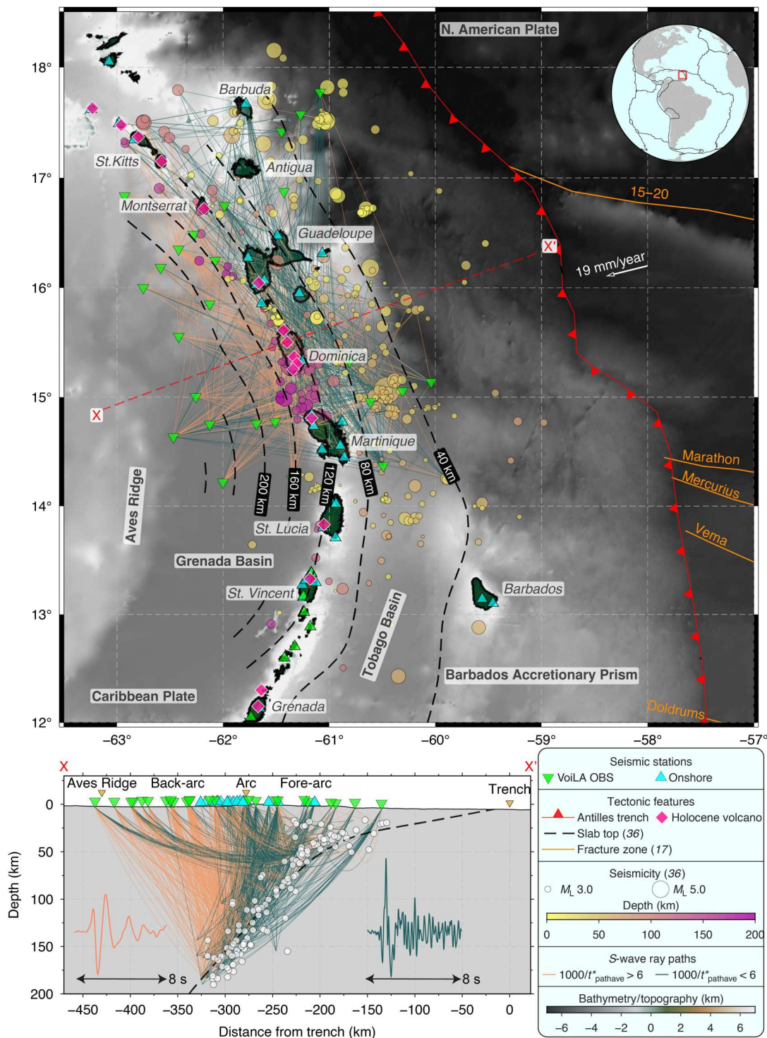
Fig. 1. Seismotectonic context of the Lesser Antilles arc, with S-wave ray-path coverage and path-averaged t_{\text{pathave}}^* results. The red box on the inset map shows the extent of the main map. Island names are labeled in italic ; tectonic features are in bold . Ray-paths in the map (top) and cross-sectional view (bottom) are traced in a three-dimensional (3D) velocity model (42), with ray-path colors showing the path-averaged attenuation operator ( t_{\text{pathave}}^* ). Orange paths have strong attenuation; green paths have weak attenuation. The orientation of the 2D model spanning the northern LAA shown in Fig. 2 is given by the red dashed line labeled X-X'. On the cross-sectional view, representative 8-s-long S waveforms on the transverse component are given for back-arc ray-paths (orange) and a fore-arc path (green) from the same intraslab earthquake at 180 km in depth (details in fig. S1).
