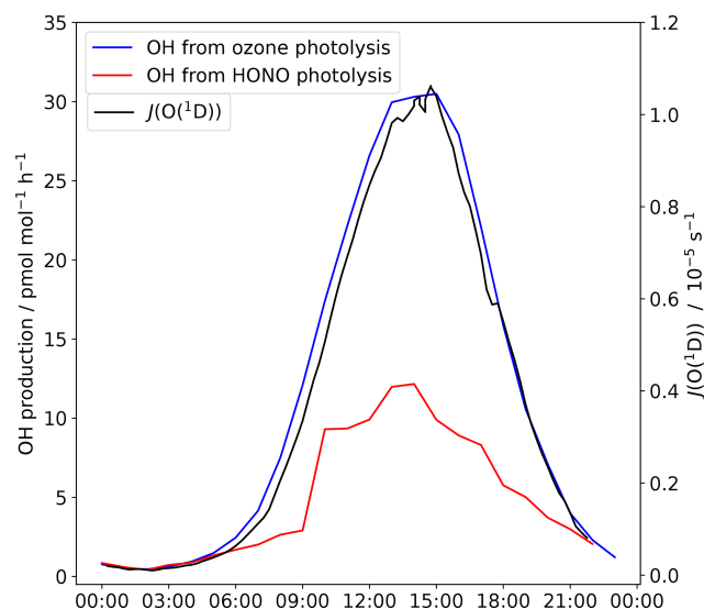
Figure 8. The contribution of HONO and ozone to the OH production rate at Halley. The average J(\text{O}(\text{D})) for Halley is also shown.
