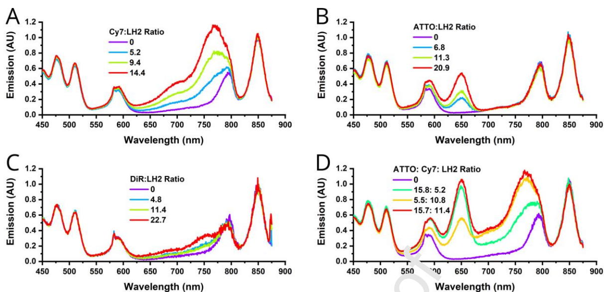
Figure 4. Comparison of the relative enhancement of LH2 by assessment of fluorescence excitation spectra. All spectra were acquired with the selective detection of LH2 emission at 875 nm, ex/em bandwidth 4/2 nm. Fluorescence excitation spectra for LH2 proteoliposomes containing either Cy7-lipids (A), ATTO-lipids (B), injected DiR (C), or both Cy7-lipids and ATTO-lipids together (D). Fluorescence excitation spectra for plant LHCII samples are shown in supplementary Fig. S5.
