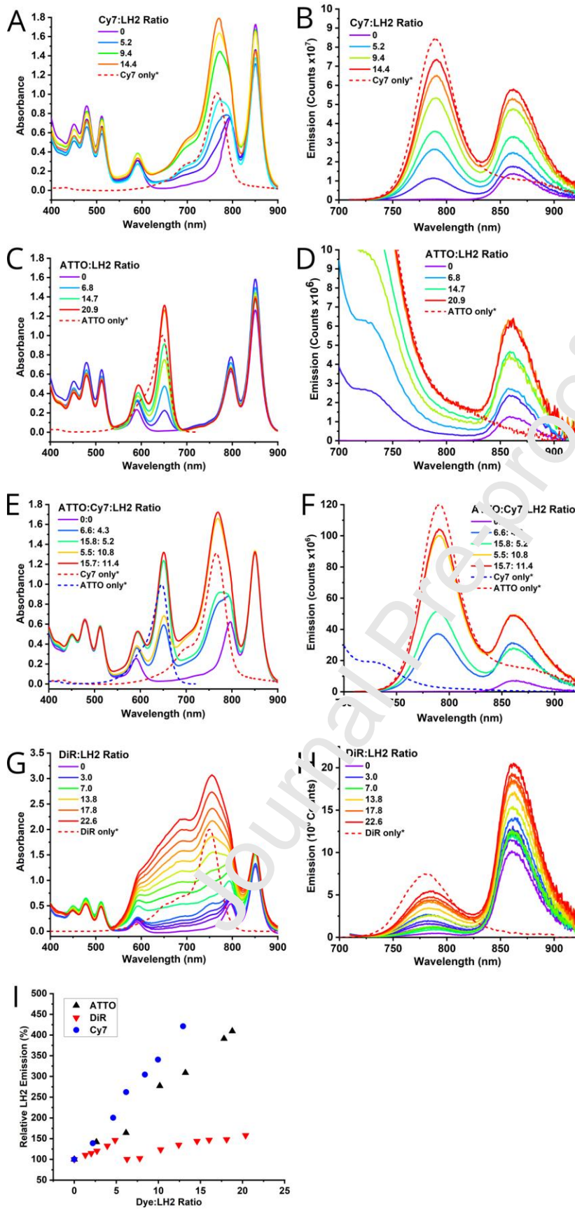
Figure 3. Comparison of the effectiveness of three different types of chromophore for enhancing fluorescence emission from the LH2 complex. Absorption spectra of LH2 proteoliposomes containing either lipid-linked Cy7 ( A ), lipid-linked ATTO ( C ), both Cy7 and
