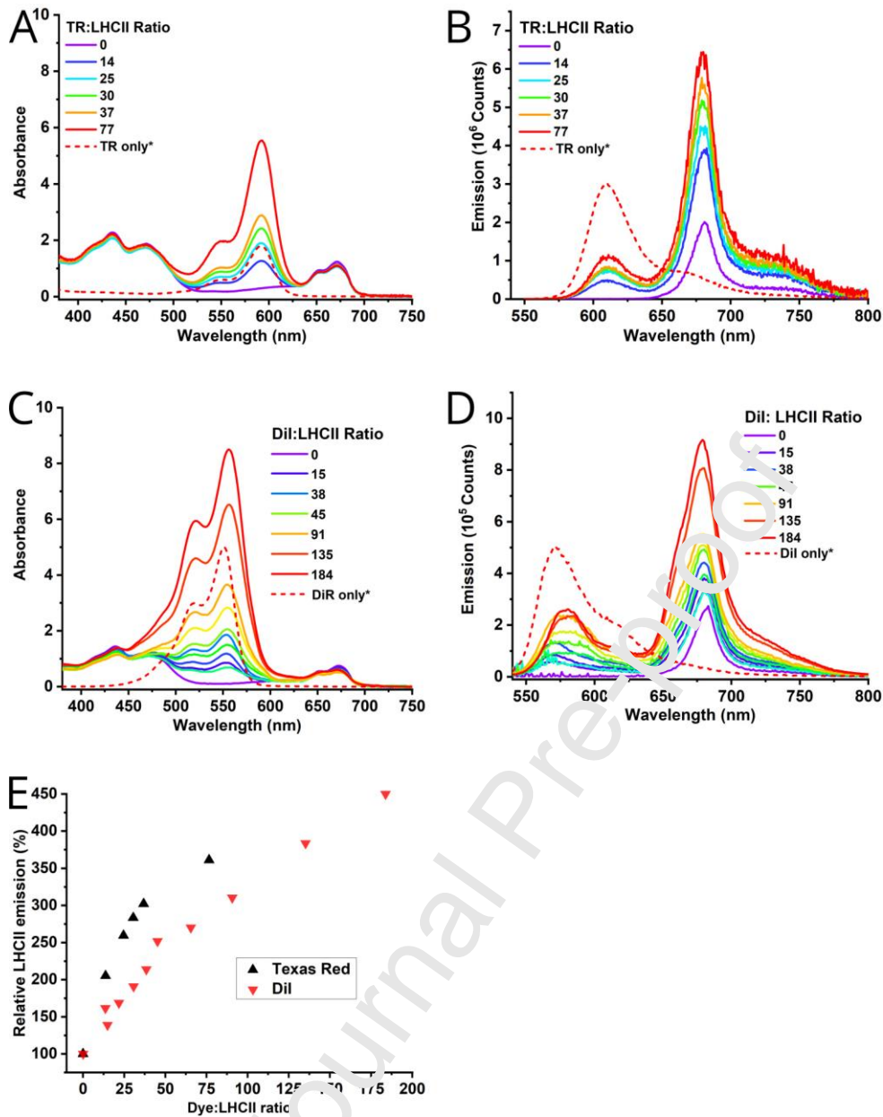
Figure 2. Comparison of the effectiveness of two different types of chromophore for enhancing plant LHCII. (A) Absorption spectra of LHCII proteoliposomes containing lipid-linked TR at the concentrations shown. *Indicates normalised reference data. (B) Fluorescence emission spectra of the same samples as in (A) with selective excitation of TR at 540 nm, ex/em bandwidths 1/1nm. (C) Absorption spectra of LHCII proteoliposomes after injection of Dil to the concentrations shown. (D) Fluorescence emission spectra of the same samples as in (C), with selective excitation of Dil at 525 nm, em/ex bandwidths 2/2 nm. Selective excitation wavelengths for dyes were chosen to minimise direct LHCII excitation rather than to be centred at their peak excitation wavelengths. Legend for each spectrum not shown for visual clarity; the full table of results are shown in supplementary Tables S1 and S3 . (E) Graph comparing the relative enhancement effect between these dyes, where 100% is the intensity of fluorescence at 680 nm in LHCII proteoliposomes in the absence of any dye. The LHCII emission intensity was calculated after subtraction of the overlapping fluorescence due to the dye, the full calculations are shown in supplementary Table S3 .
