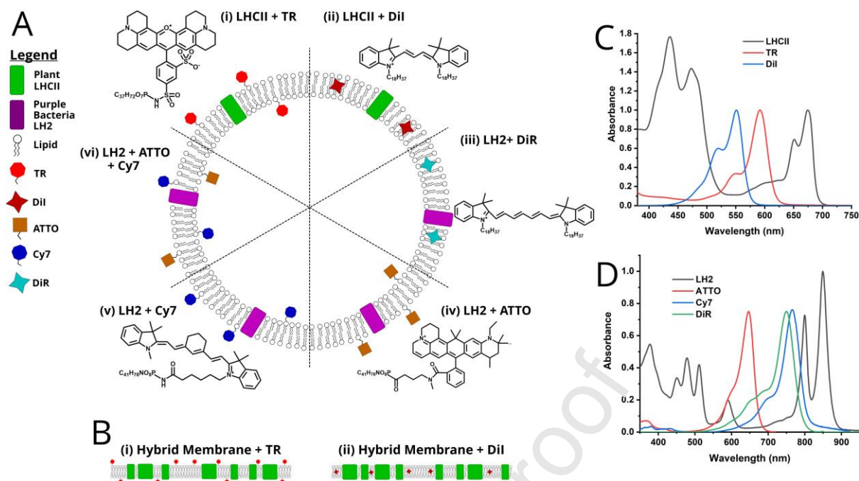
Figure 1. Schematic of the series of model membrane samples studied in this work. Proteoliposomes ( A ) were generated by combining lipids and biochemically-purified proteins in the desired molar ratios, following an established procedure that induces the spontaneous self-assembly of membrane vesicles (see Methods 2.4 ). When lipid-linked chromophores were used (TR, ATTO, Cy7) these were incorporated into the membrane during lipid and protein assembly, whereas the hydrophobic pigments (DiI, DiR) were injected into the buffer solution immediately prior to measurement with multiple sequential injections possible. Full chemical structures of the dyes are given in the Methods 2.1 . Supported membranes ( B ) were assembled onto hydrophilic glass coverslips, following a recently-developed procedure to generate “hybrid membranes” comprising a fusion of thylakoid membranes extracted from spinach chloroplasts and synthetic liposomes. Normalised absorption spectra of plant LHCII ( C ), and LH2 ( D ), with the additional dyes used to enhance the absorption of each protein. All dyes were obtained from commercial suppliers. The LH complexes were purified using established biochemical procedures (see Methods 2.2-2.3 and Fig. S1-S2 ).
