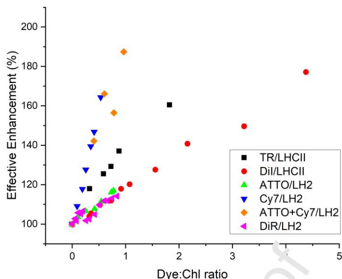
Figure 5. Comparison of LH protein enhancement between all dye and protein combinations, considering an extended spectral range. The “effective absorption” was calculated from the integrated areas under the fluorescence excitation spectra for LH2 (Fig. 4) and plant LHCII (Fig. S2), and normalizing so that 100% absorption (380-680 nm and 450-875 nm for LHCII and LH2, respectively) represents the natural (unmodified) protein complex. The numerical data are tabulated in see supplementary Table S5. The molar Dye:Chl ratio was calculated as [dye:protein] \times 2 for plant LHCII and [dye:protein] \times 27 for plant LH2, using the dye:protein ratios already determined from absorption spectra (see supplementary Table S1).
