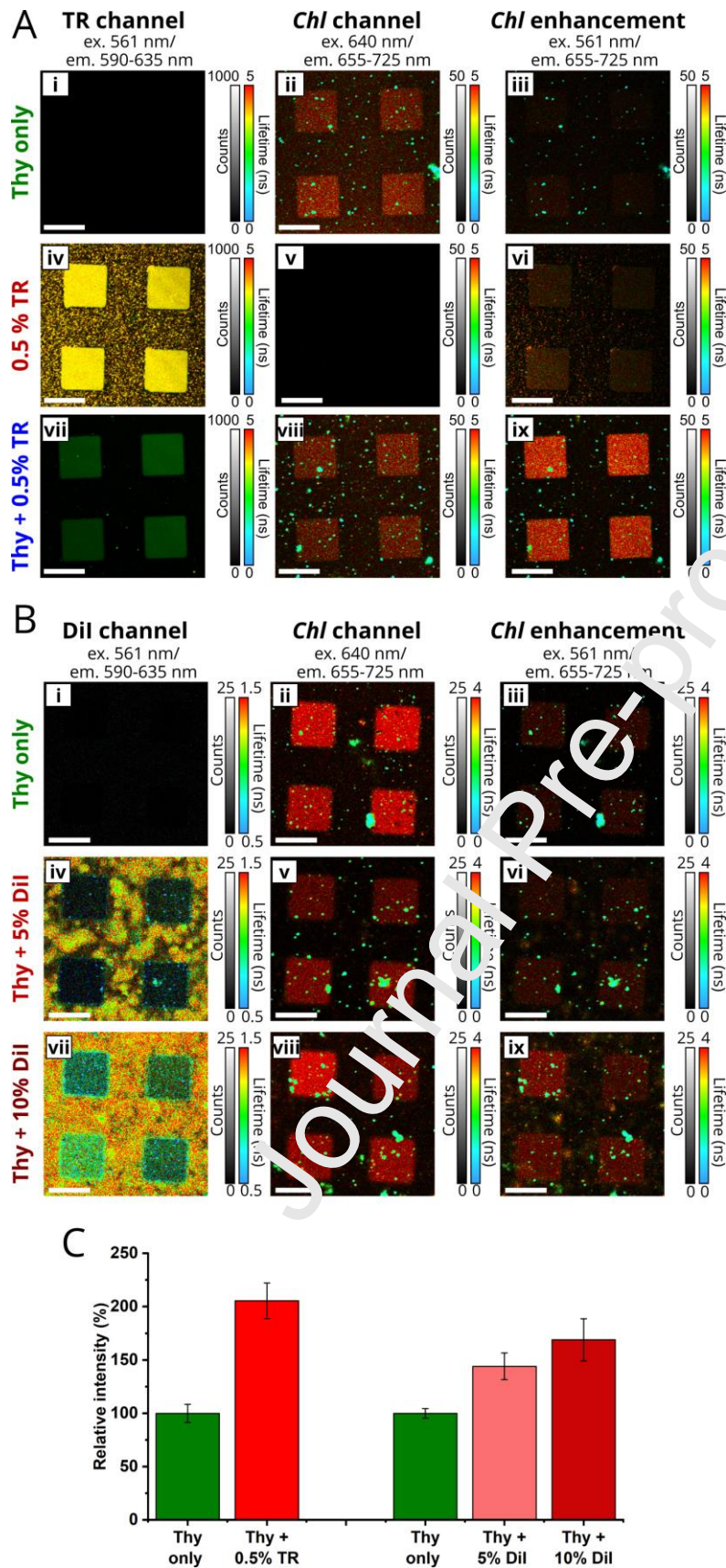
Figure 6. Comparison of the effectiveness of TR and Dil dyes to enhance the fluorescence of surface-supported “hybrid thylakoid membranes”. (A) Series of FLIM images to test the effectiveness of TR. “Thy-only” (panels i-iii) represents hybrid membranes generated by
