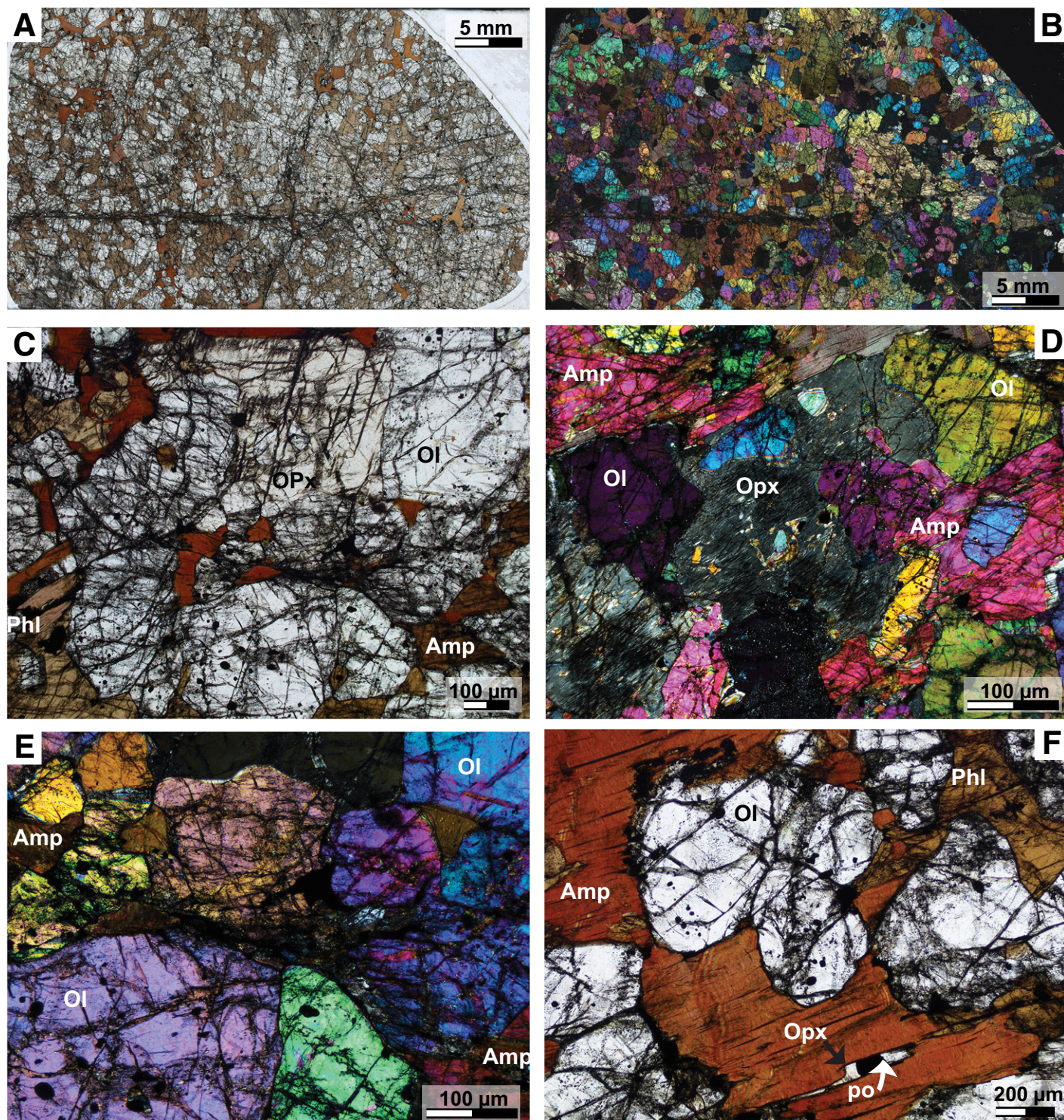
Figure 2. Photomicrographs of I2 (center of the pipe) Ivrea-Verbanò sample. (A) Plane-polarized photomicrograph of the entire thin section. (B) Cross-polarized photomicrograph of the entire thin section. (C) Olivine crystals are enclosed by oikocrysts, composed of amphibole and phlogopite. (D) Oikocryst of altered orthopyroxene surrounding olivine crystals. (E) Fractured olivine crystals with recrystallization zone at the contact between olivine grains. (F) Oikocrystic amphibole contains orthopyroxene and pyrrhotite along the cleavage plane. Abbreviations: Ol—olivine; Amp—amphibole; Opx—orthopyroxene; Phl—phlogopite; po—pyrrhotite.
