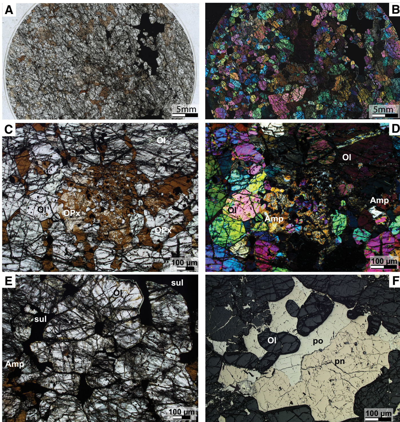
Figure 3. Photomicrographs of I7 (margin of the pipe) Ivrea Verbano sample. (A) Plane-polarized photomicrograph of the 2.5-cm-diameter thin section. (B) Cross-polarized photomicrograph of the 2.5-cm-diameter thin section. (C) Plane-polarized photomicrograph of complex reaction between orthopyroxene and amphibole. (D) Cross-polarized light photomicrograph of the image in C. (E) Plane-polarized light image of fine sulfide crystals (pyrrhotite) enclosed by olivine crystals. (F) Reflected light microphotograph of large sulfide aggregate composed of pyrrhotite and pentlandite. Abbreviations: Ol—olivine; Amp—amphibole; OPx—orthopyroxene; sul—sulphides; po—pyrrhotite; pn—pentlandite.
