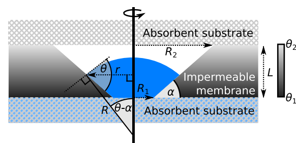
Figure 1. 2D illustration of the axisymmetric pore construction and outgoing meniscus profile. The axis of symmetry is shown as the thick vertical line. Liquid is shown in blue, with vapor shown in white.
