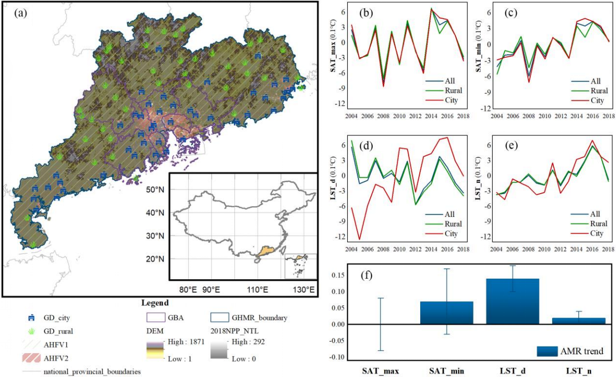
Fig.1 Impacts of urbanization on summer SAT and LST changes in the GHMR from 2004-2018. (a) Regional and observatory distribution, urban and non-urban divisions. (b-e) Comparison of regional mean variations of summer SAT max (b), SAT_min (c), LST_d (d) and LST_n (e), for the whole GHMR, in urban areas and in rural areas; (f) Contribution of urbanization to the trends of summer SAT and LST changes in GHMR and its significance (at the 5% level)
