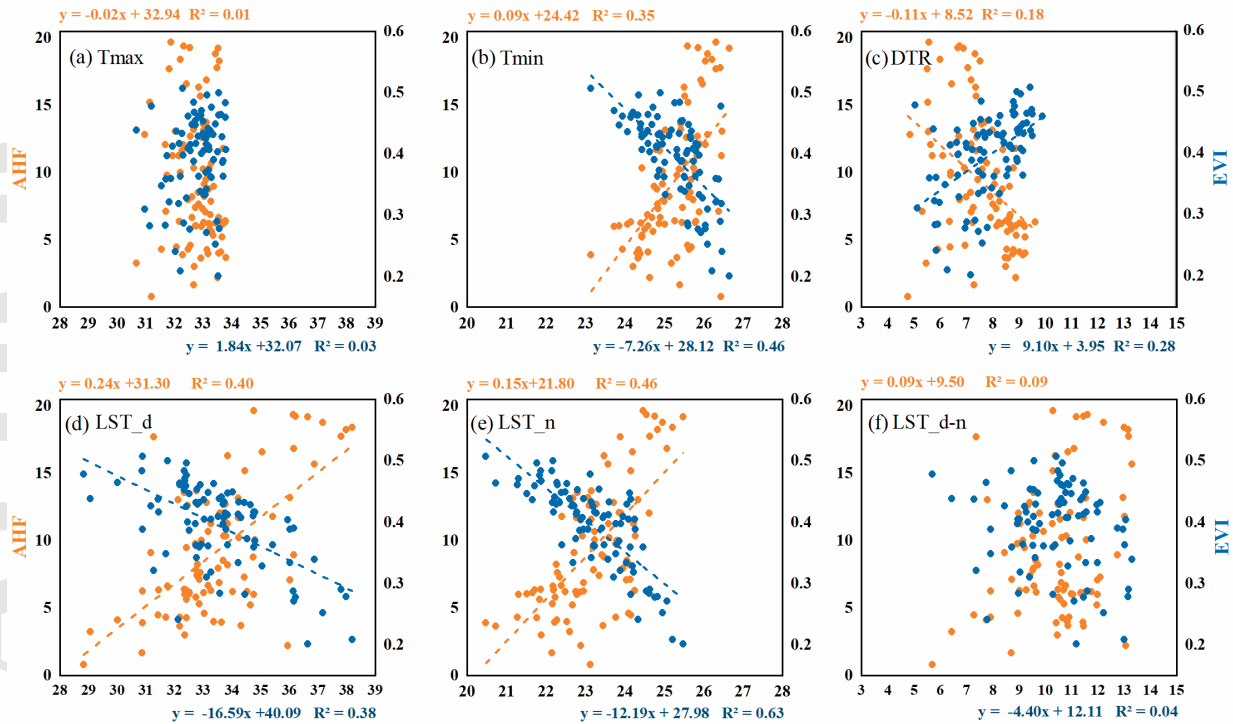
Fig.4 Map of the interrelationship of EVI and AHF distributions with SAT (Tmax, Tmin, DTR) and LST (LST_d, LST_n, LST_d-n) at local sites (86 meteorological stations)
