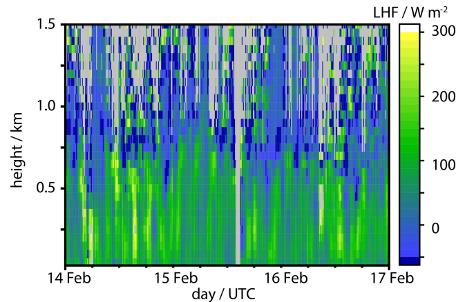
Figure 6. Vertical latent-heat (vaporization enthalpy) flux as a function of time and height above the platform as measured from the combination of water vapor Raman lidar (ARTHUS) and Doppler wind lidar aboard the R/V MS-Merian . The mean value over the 3 d period is 100 \text{ W m}^{-2} at 200 m, and the fluxes are positive throughout the sub-cloud layer.
