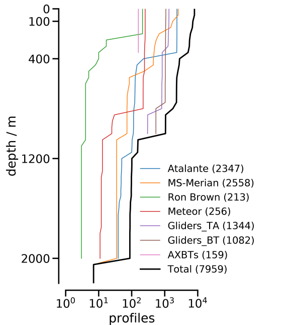
Figure 5. Number of profiles sampling seawater properties at the indicated depth. Ship-based profiling is from CTD casts, underway CTDs, XBTs, and moving vessel profilers. AXBTs were dropped by the P-3.
