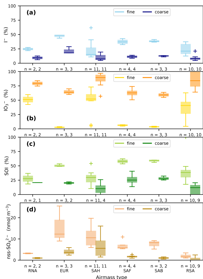
Figure 4. Proportions of (a) \text{I}^- , (b) \text{IO}_3^- , and (c) SOI (expressed as percentage of TSI) and (d) the concentrations of \text{nss-SO}_4^{2-} in fine ( < 1 \mu\text{m} ) and coarse ( > 1 \mu\text{m} ) aerosols in the different air mass types encountered during AMT21. The number of samples in fine and coarse fractions respectively for each group ( n ) is also shown. In some cases, unreliable results for SOI and \text{nss-SO}_4^{2-} in the coarse mode were excluded, as described in the text. Boxes show the interquartile range of the data, with horizontal lines representing the median. Whiskers show the range of the data, except where outliers more than 1.5 times the inter-quartile range beyond each quartile are present (crosses).
