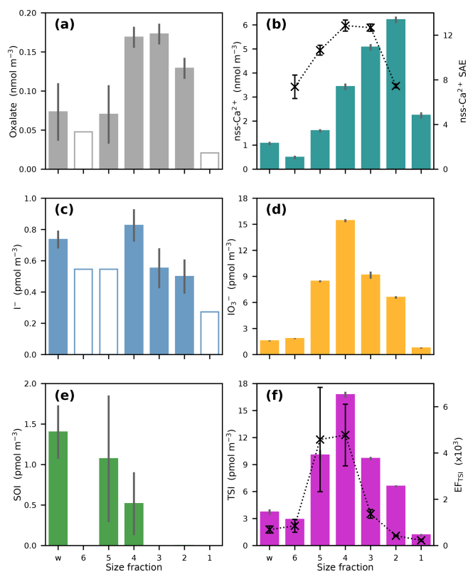
Figure 6. Concentrations of (a) oxalate, (b) \text{nss-Ca}^{2+} , (c) \text{I}^- , (d) \text{IO}_3^- , (e) SOI and (f) TSI in the size fractions of sample 15. ( w indicates the backup filter and particle size increases from stage 6 to stage 1 – stage cut-off diameters are given in the text). Crosses in (b) show the surface area equivalent (SAE) of \text{nss-Ca}^{2+} (arbitrary units) for impactor stages 2–6 and in (f) show the enrichment factors of TSI in each stage.
