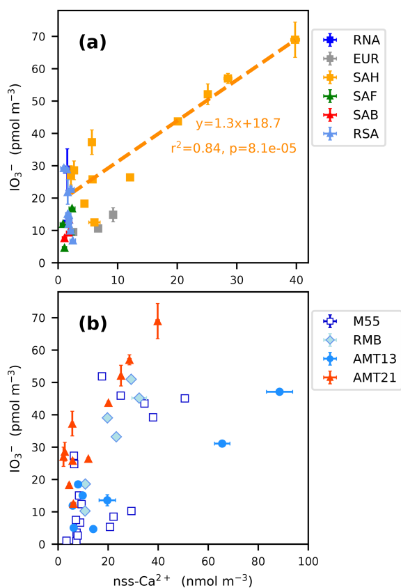
Figure 5. Total (sum of fine and coarse) aerosol \text{IO}_3^- concentrations as a function of \text{nss-Ca}^{2+} concentrations for (a) all of the air mass types encountered during AMT21 and (b) for SAH-type samples during the M55, RHaMBLe (RMB), AMT13 and AMT21 cruises. Air mass type codes are described in the text.
