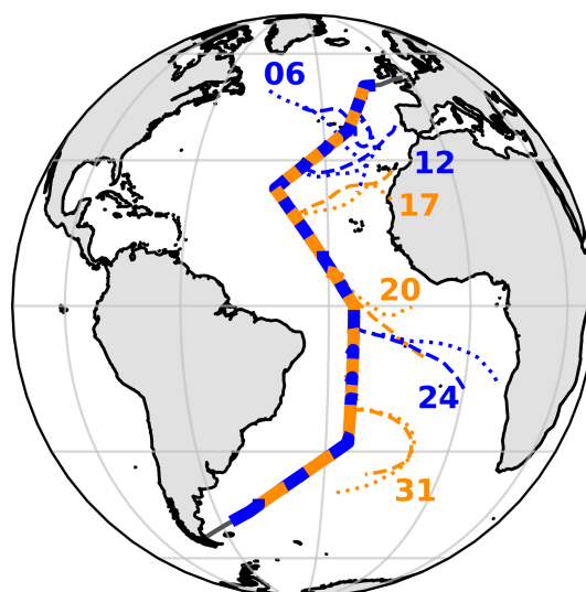
Figure 1. AMT21 cruise track, with aerosol collection periods for each sample shown as alternating blue and orange bars. Five-day air mass back-trajectories for heights of 10 (dashed) and 1000 m (dotted) above the ship's position are shown for samples 06, 12, 17, 20, 24 and 31, representing the RNA, EUR, SAH, SAF, SAB and RSA air mass types respectively (air mass codes are described in the text).
