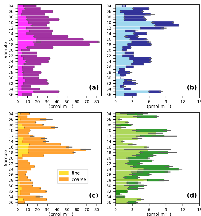
Figure 3. Fine (< 1 \mu\text{m} ) and coarse (> 1 \mu\text{m} ) aerosol concentrations of (a) TSI, (b) \text{I}^- , (c) \text{IO}_3^- , and (d) SOI during the AMT21 cruise. Details are as for Fig. 2.
