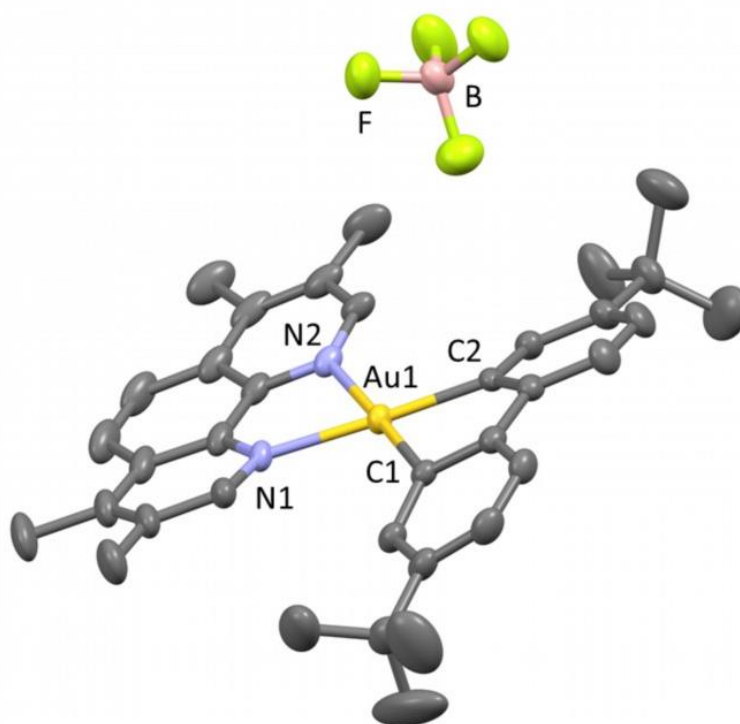
Figure 5: Crystal structure of complex 5a . Ellipsoids set at 50% probability. Hydrogen atoms and toluene have been omitted for clarity. Selected bond distances [Å] and angles [°] measured at 140K:
