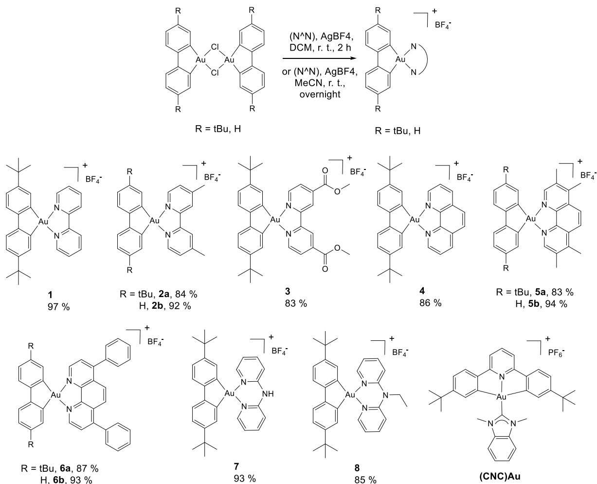
Figure 3: Synthesis and structure of [(\text{C}^{\text{C}})\text{Au}(\text{N}^{\text{N}}\text{)}]\text{BF}_4 complexes 1-8 and (CNC)Au.
