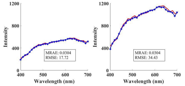
Figure 2. Compare the reconstructed spectra by A+ algorithm [2] (blue curves) with the ground-truth radiance spectra (red curves). RMSE evaluation scales with the brightness level, while MRAE do not.
