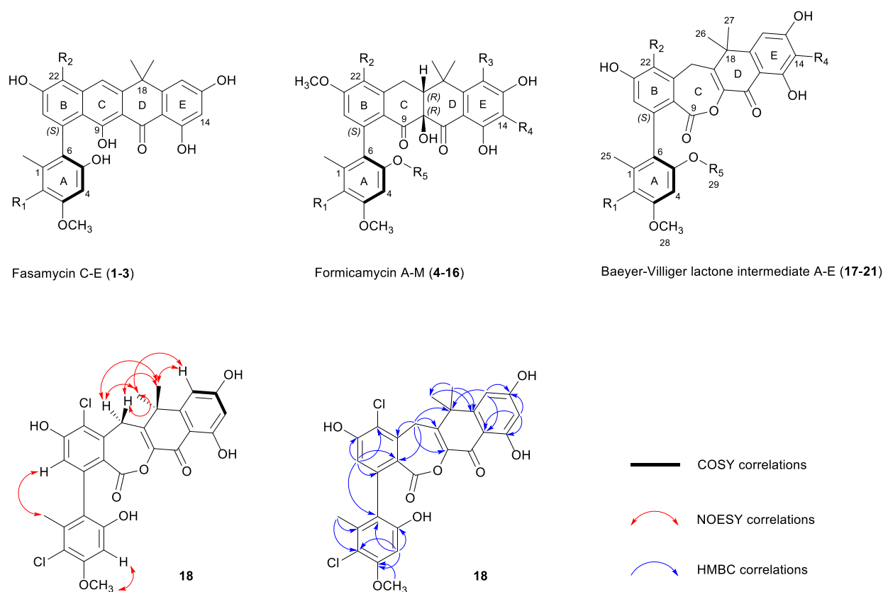
Fig. 1 Chemical skeletons of fasamycins ( 1-3 ) and formicamycins ( 4-16 ) isolated from S. formicae KY5, and Baeyer-Villiger lactone intermediates ( 17-21 ) isolated from the S. formicae \Delta forY mutant in this study (for detailed substituent variations including halogenation or O -methylation, see Fig. S1). The 2D NMR structure determination of 18 is shown by COSY (bold), NOESY (red double-head arrow), and selected HMBC (blue single-head arrow) correlations respectively. R_{1-4} = H or Cl; R_5 = H or \text{CH}_3 .
