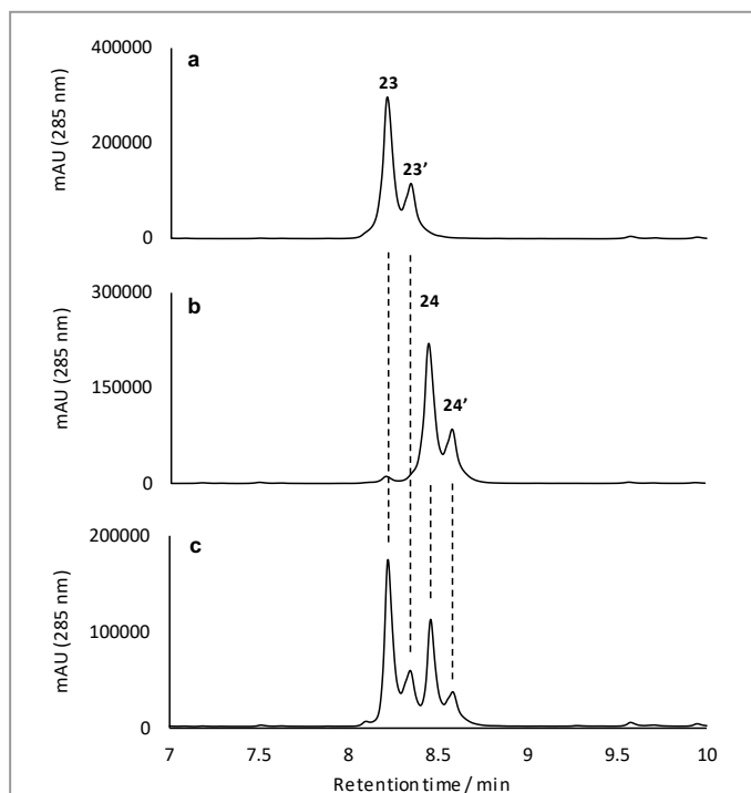
Fig. 5 Reconstituted UPLC-UV (285 nm) analysis for the isolated reduction products 23 (a), 24 (b), and a mixture of the isolated products (c) indicating the diastereomeric composition of these samples.
