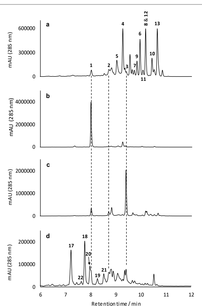
Fig. 2 Mutational analysis of the tailoring enzyme encoding genes involved in formicamycin biosynthesis. Deletion of forX abolishes the production of formicamycins but leads to accumulation of fasamycin E ( 3 ). Deletion of forY abolishes the production of formicamycins and leads to accumulation of six biosynthetic intermediates ( 17–22 ). Reconstituted HPLC traces (UV = 285 nm) showing: (a) S. formicae wild type; (b) S. formicae \Delta forV (for details see 7 ); (c) S. formicae \Delta forX ; (d) S. formicae \Delta forY .
