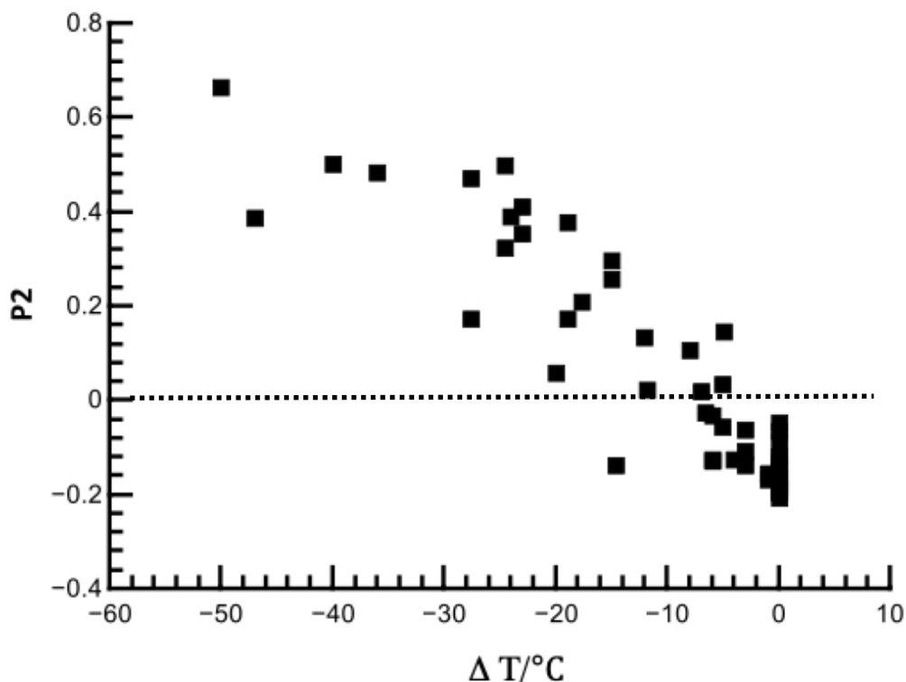
Figure 6 Plot of the values of the second principal component (P2) versus the depression of onset of the melting temperature ( \Delta T ).
