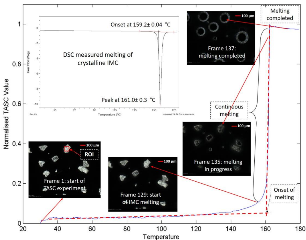
Figure 2 A typical TASC plot of the melting of a crystalline drug particle (IMC) with the microscopic images at different stages of the heating, and the comparison with the melting onset temperature with the DSC (insert). The heating rate was 20 °C/min in both cases.
