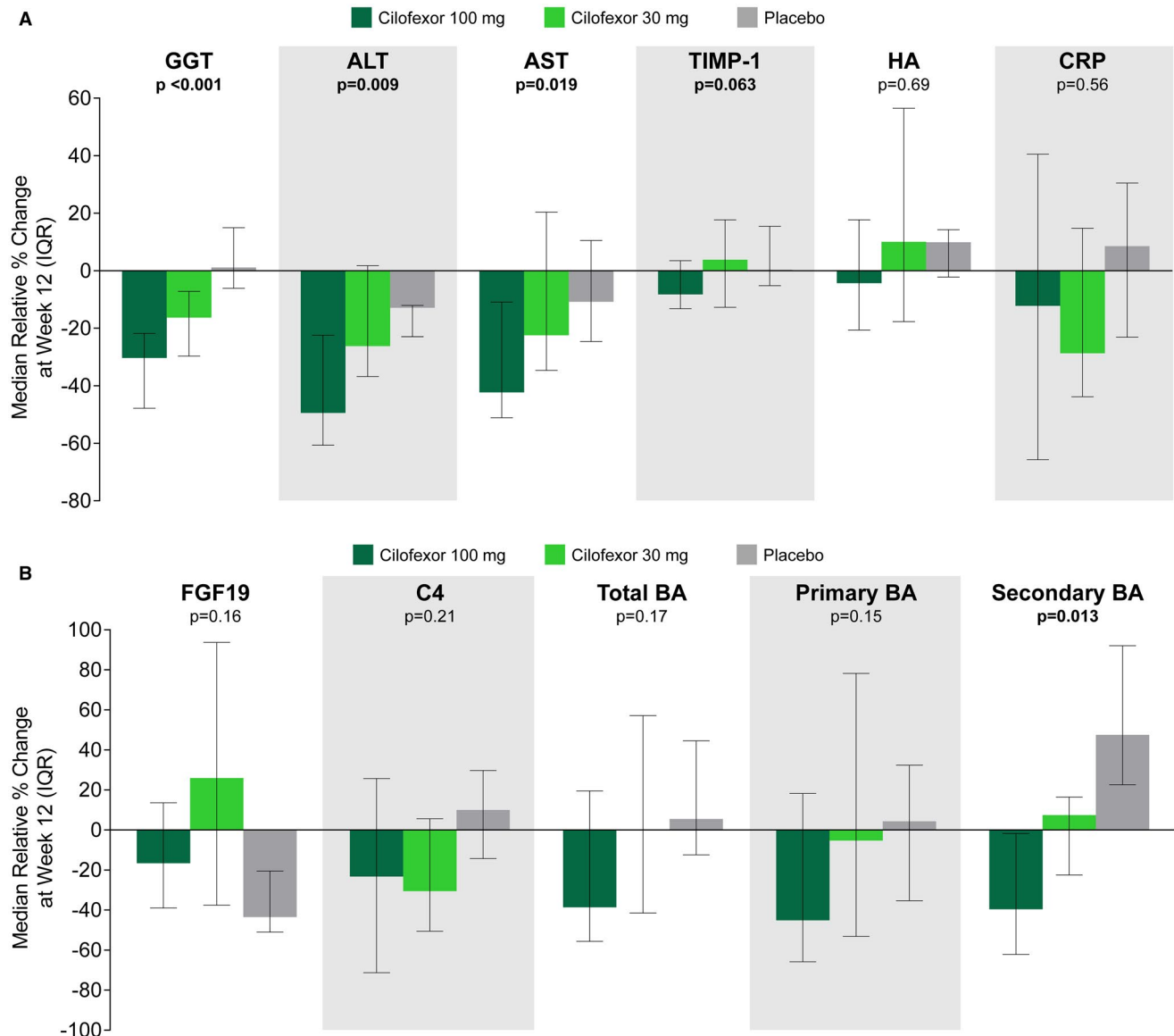
FIG. 2. Effect of cilofexor on liver biochemistry and markers of fibrosis and bile acid homeostasis. (A) Cilofexor 100 mg leads to improvement in serum GGT, ALT, AST, and TIMP-1 compared with placebo. P values for cilofexor 100 mg versus placebo are according to Wilcoxon rank-sum test. (B) Cilofexor leads to reductions in C4, total bile acids, primary bile acids, and secondary bile acids compared with placebo. Total bile acids by enzymatic assay and bile acid species by LC/MS-MS. UDCA and its conjugates have been removed from secondary bile acids. P values for cilofexor 100 mg versus placebo are according to Wilcoxon rank-sum test. Abbreviations: BA, bile acid; HA, hyaluronic acid.
