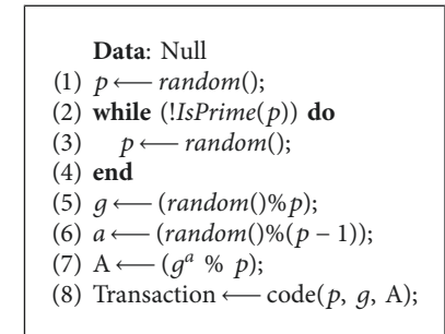
ALGORITHM 2: System parameters are generated and uploaded into blockchain (type-II).
