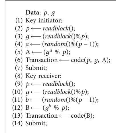
ALGORITHM 3: Master key parameters are generated to blockchain (type-I).
