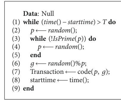
ALGORITHM 1: System parameters are generated and uploaded into blockchain (type-I).
