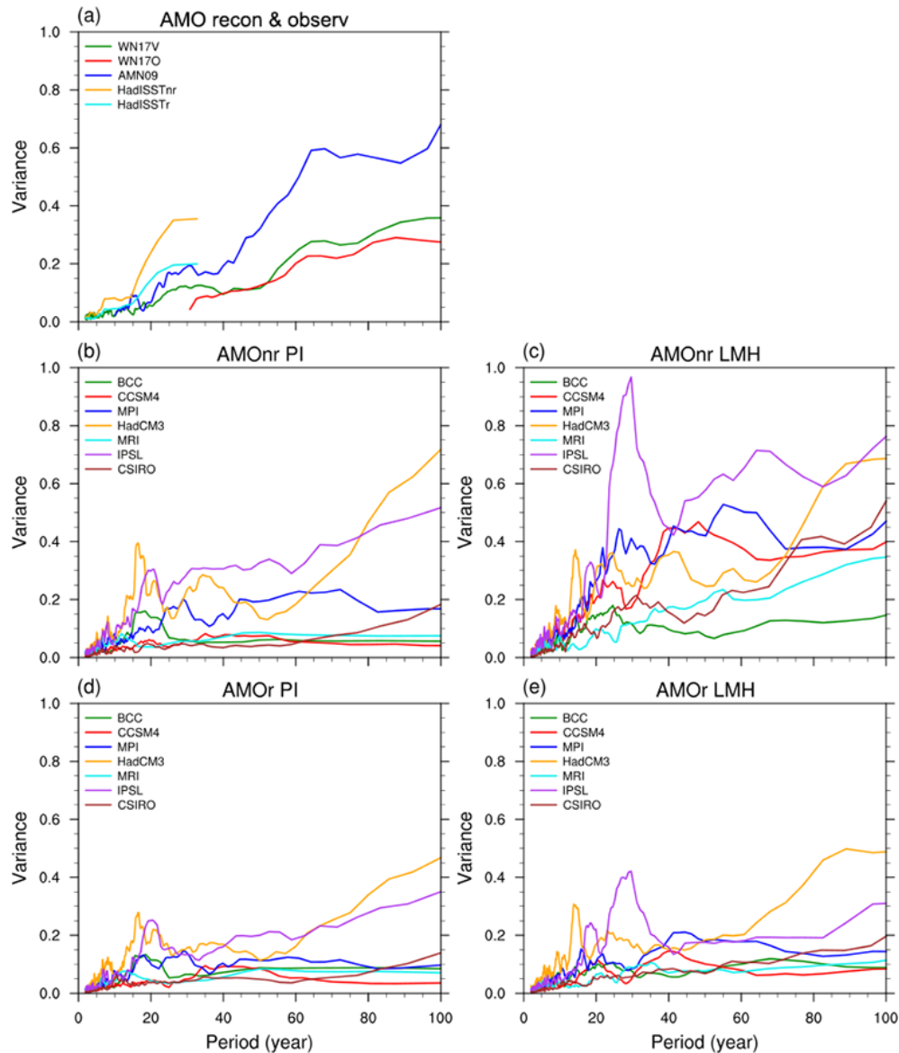
Figure 10. Spectra of AMO index of reconstructions and instrumental data (a) and each of seven GCMs for PI (b, d) and LMH (c, e) experiments. AMOnr and AMOr are the two definitions of AMO index described in Fig. 1. Spectra are not shown for timescales that the underlying data cannot adequately represent (not for < 30 years for WN17O and not for < 10 years for AMN09 because these reconstructions use 30-year and 10-year low-pass-filtered data, respectively, and not for > 30 years for HadISST because the instrumental data are too short to determine power on longer timescales).
