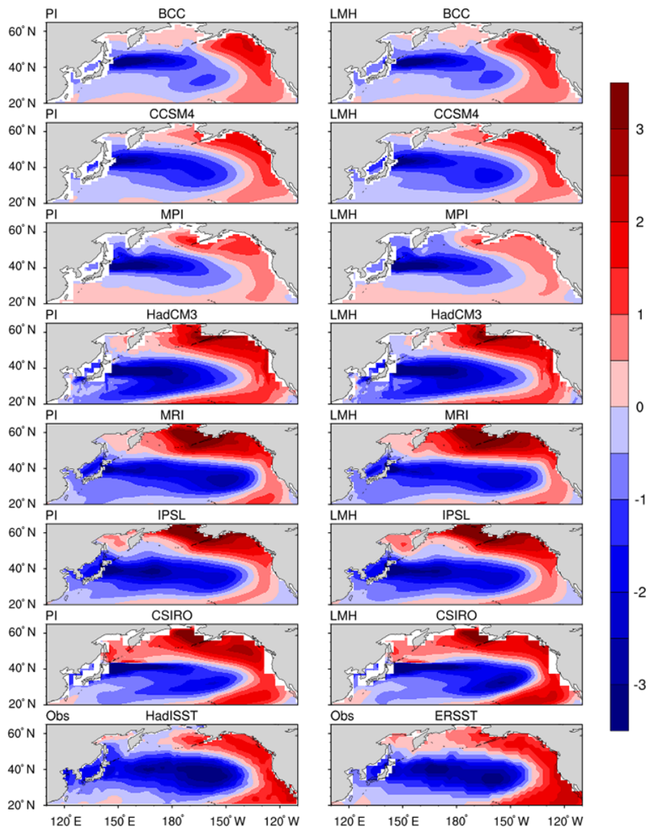
Figure 2. PDO SST patterns defined by the first empirical orthogonal function (EOF) of annual-mean SST for each GCM for the PI (first column) and LMH (second column) experiments compared with the HadISST and ERSST observations (bottom row).
