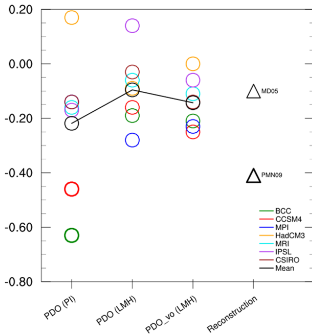
Figure 6. Correlations of annual-mean East Asian regional average surface temperature against PDO index for each GCM (circles) for PI and LMH experiments compared with reconstructions (triangles). The mean correlations for the seven GCMs are marked with black circles connected by a solid line; “vo” indicates that the volcanic influence on East Asian temperature has been removed by linear regression in the LMH experiments. The thick circles and triangles show values significant at 95 % level using a two-tailed Student’s t test. The reconstruction correlations are between the WN18 East Asian temperature and the two PDO reconstructions (Table 2).
