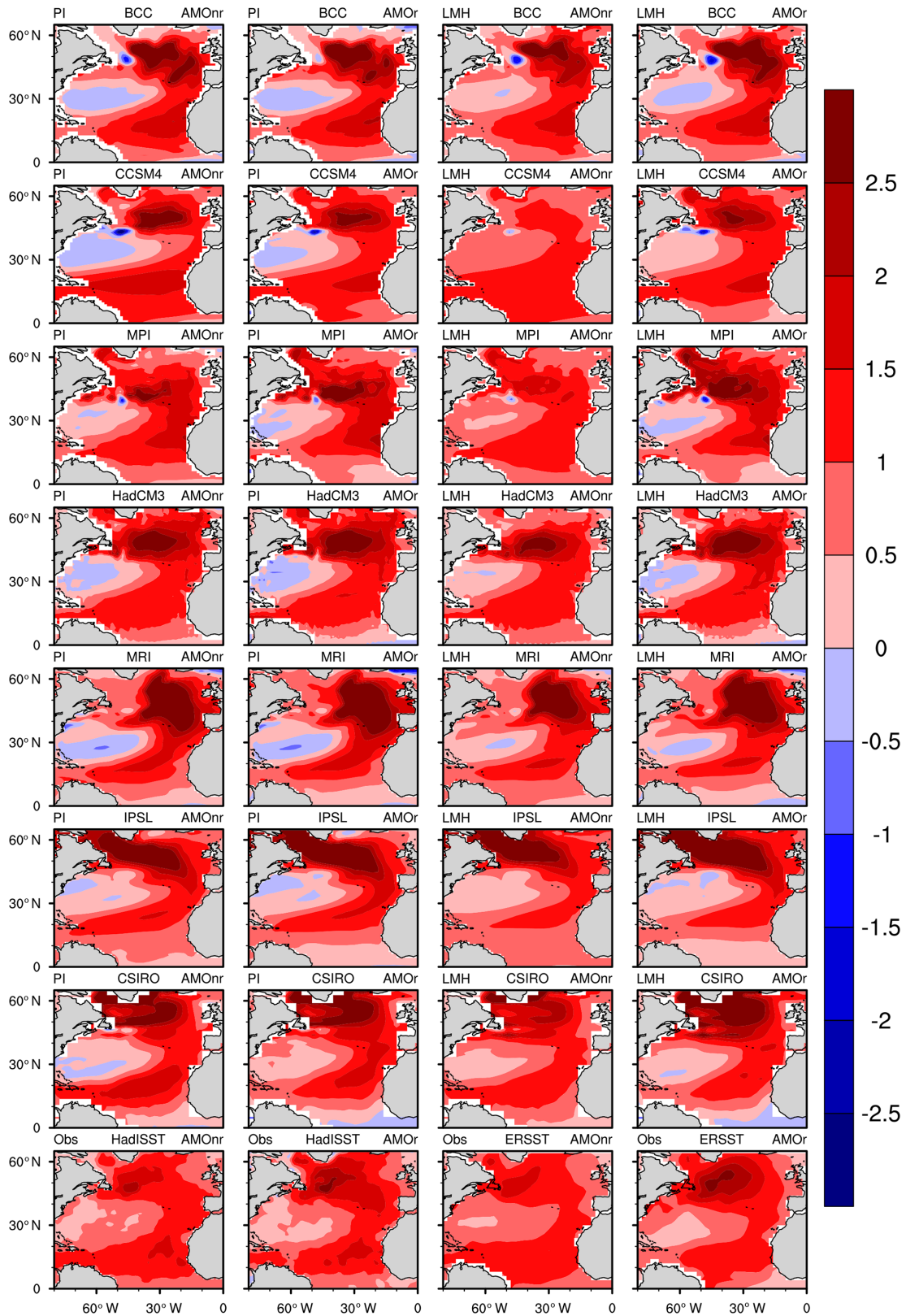
Figure 1. AMO patterns defined by regression of annual-mean SST on the AMO index for each GCM for the PI (first and second columns) and LMH (third and fourth columns) experiments compared with HadISST and ERSST observation (bottom row). The first and third columns use the AMO index calculated without subtracting the global SST anomaly (AMOnr), while the second and fourth columns use the AMO index after subtracting the global SST anomaly (AMOr).
