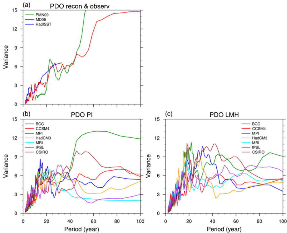
Figure 11. Spectra of PDO index of reconstructions and instrumental data (a) and GCMs for PI (b) and LMH (c) experiments. Spectra are not shown for timescales that the underlying data cannot adequately represent (not for < 10 years for PMN09 because this reconstruction uses 10-year low-pass-filtered data, and not for > 30 years for HadISST because the instrumental data are too short to determine power on longer timescales).
