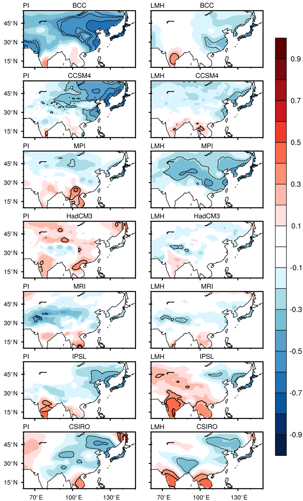
Figure 5. Correlations between annual-mean East Asian surface temperatures and PDO index for each GCM for PI (first column) and LMH (second column) experiments. Correlation values significant at 90 % levels using a two-tailed Student's t test are contoured.
