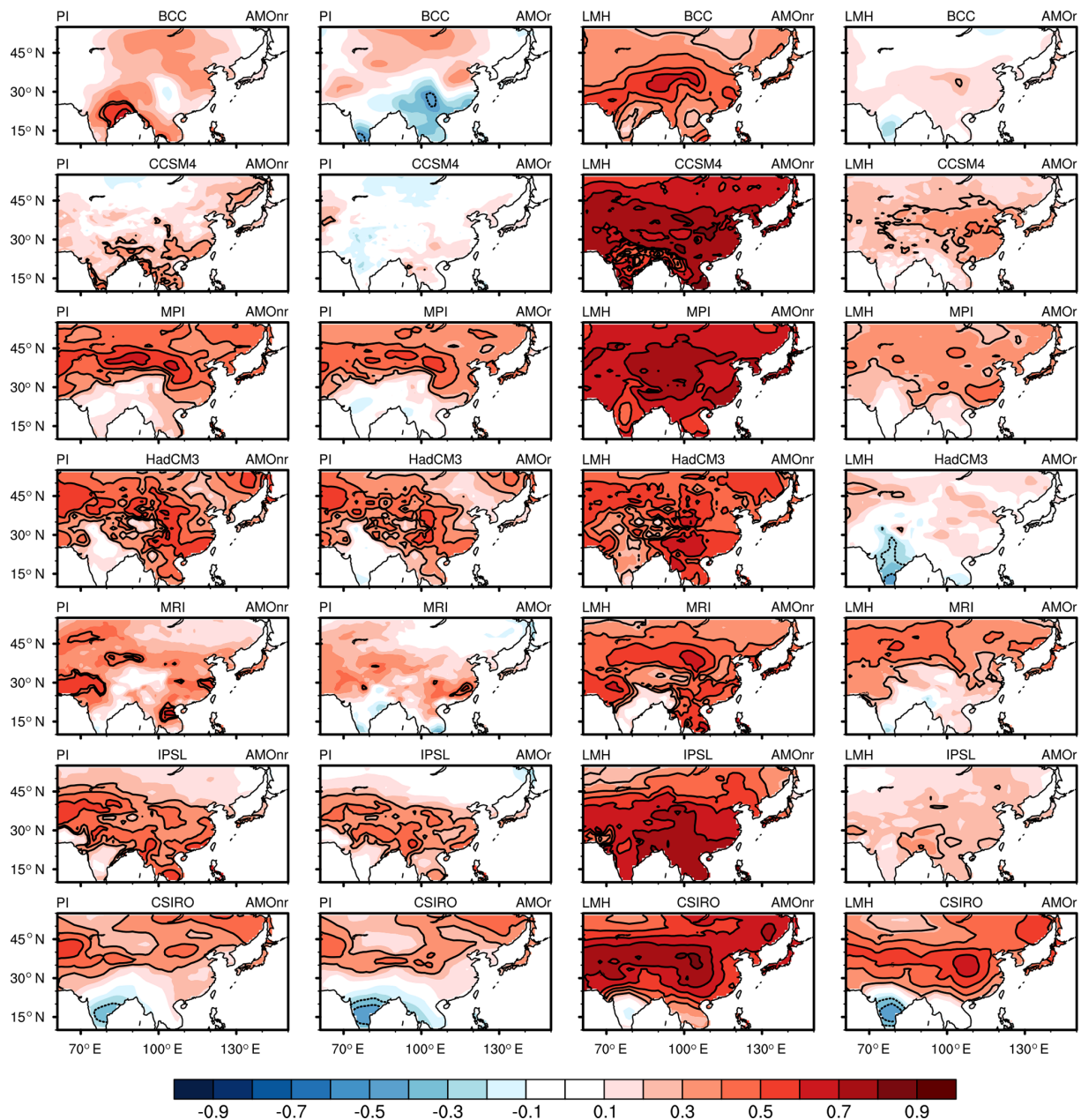
Figure 3. Correlations between annual-mean East Asian surface temperatures and AMO index for each GCM for PI (first and second columns) and LMH (third and fourth columns) experiments. AMONr and AMOr are the two definitions of AMO index as described in Fig. 1. Correlation values significant at 90 % levels using a two-tailed Student's t test are contoured.
