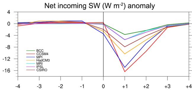
Figure 9. Annual-mean composite anomaly of net shortwave (SW) radiation at the top of the atmosphere for three large volcanic eruption events for each GCM. Individual GCM results are aligned so that their peak negative SW anomalies occur at year+1 (i.e. 1258, 1452, 1815 for BCC, CCSM4, IPSL; 1258, 1452, 1816 for MRI; 1258, 1456, 1816 for MPI, HadCM3, CSIRO).
