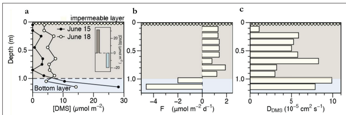
Figure 6: Calculation of the DMS flux and diffusion coefficient in brine. (a) Profiles of DMS concentration ( \mu\text{mol m}^{-2} ) in the sea-ice cover on June 15 and June 18, showing DMS accumulation in the internal ice layer (0 to 1 m) and loss of DMS from the bottom ice (1.0 to 1.25 m) due to upward diffusion across the ice cover, with total amount gained in the internal layer and lost from the bottom layer shown in the insert; (b) DMS fluxes in or out of each 0.1-m ice layer computed as the difference of DMS quantities between June 15 and June 18 as shown in panel (a) divided by the time in days; (c) computed diffusion coefficient D_{\text{DMS/br}} for each 0.1-m ice layer, using Equation 5, the DMS flux F in panel (b), and the difference in DMS quantities observed between June 15 and June 18 ( [\text{DMS}]_{\text{br J18}} - [\text{DMS}]_{\text{br J15}} ) for each 0.1-m ice layer. DOI: https://doi.org/10.1525/elementa.370.f6
