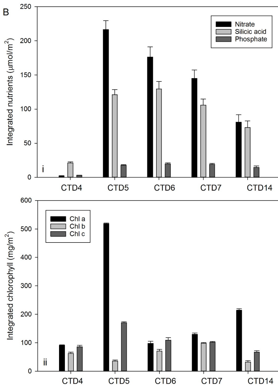
B) Example cross section of integrated (top 50m) macronutrient and algal pigment concentrations from northern section of the Nuuk grid (from CTD 4 to CTD 7, 14, see Figure 2). i) Integrated macronutrients; ii) Integrated pigment concentrations. Error bars show propagated errors on integration calculation (1SD).
