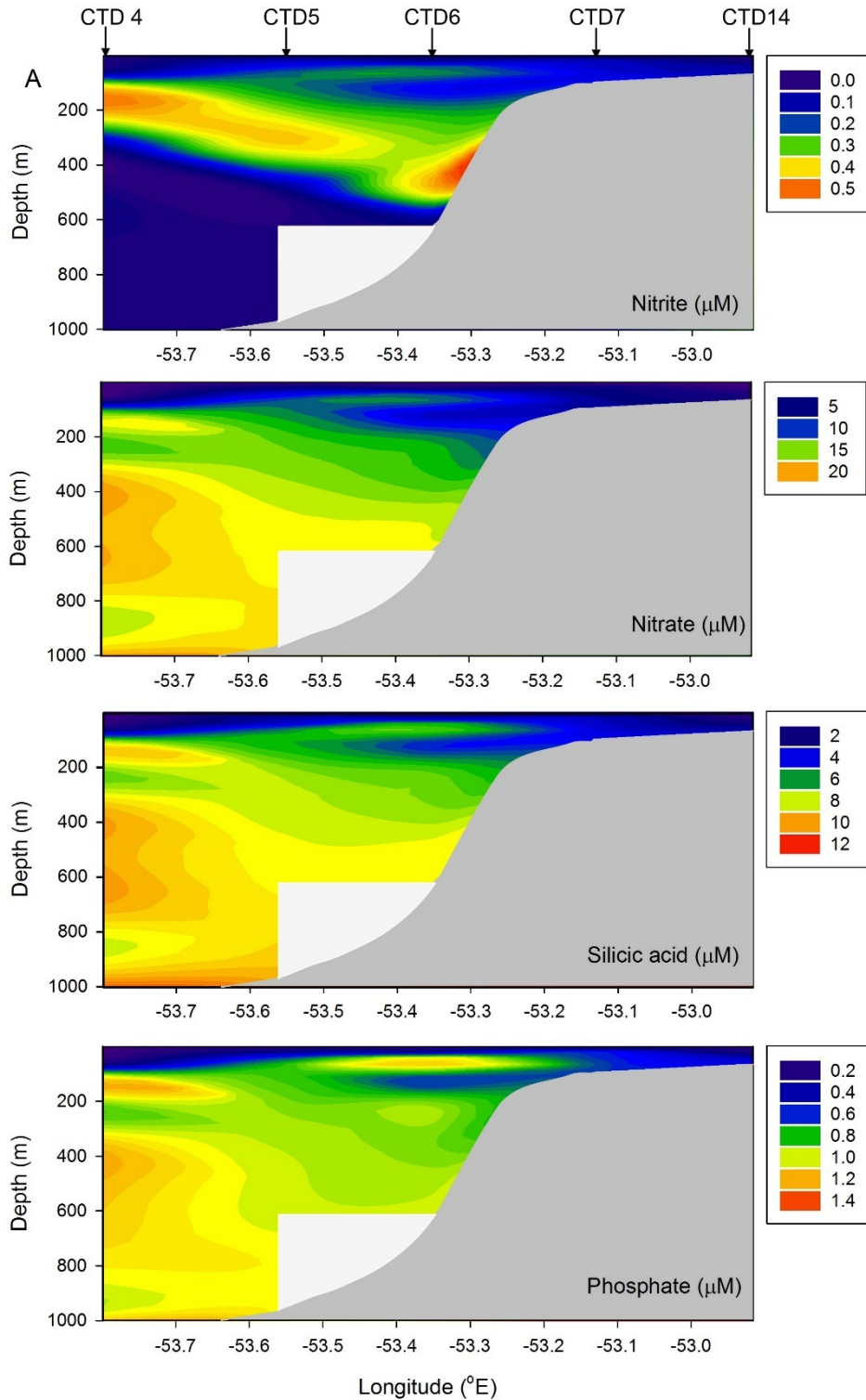
Figure A2: A) Example cross section of macronutrient concentrations from the northern section of the Nuuk grid (from CTD 4,5,6,7,14, see Figure 2), showing (from top to bottom): nitrite, nitrate+nitrite, silicic acid, and phosphate (all in \mu\text{M} ). This section encompasses the margin from the slope onto the shelf, and did not occupy the bathymetric trough (c.f. Figure 3, main text).
