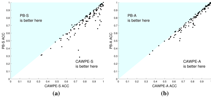
Fig. 9 Accuracy of a CAWPE-S and b CAWPE-A versus picking the best component
