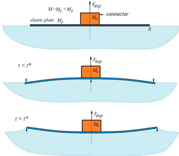
Figure 8: Sketch of the expected motion during the initial stages of the elastic disc lifting from the water surface.
