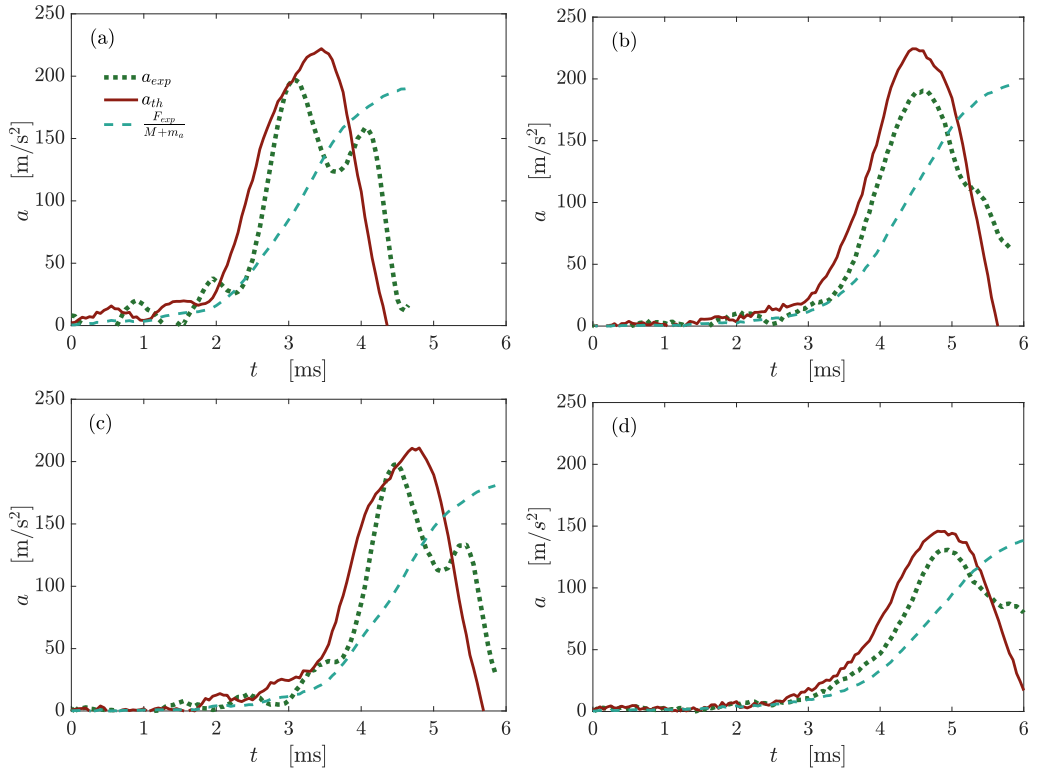
Figure 10: Comparison of the theoretical accelerations at the disc centre with the experimental ones for four runs (session 3, repetitions 2, 3, 4, and 5). Dashed lines represent the rigid wet-body acceleration, F_{exp}(t)/(M + m_a) , solid lines the theoretical accelerations at the disc centre provided by equation (4.25) and the dotted lines are for the measured accelerations.
