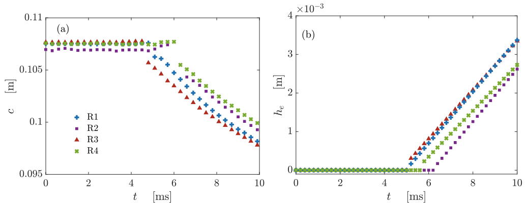
Figure 5: Evolution of the radius of the wetted area and the vertical displacement of the edge of the plate for four experimental realizations of session 3.
