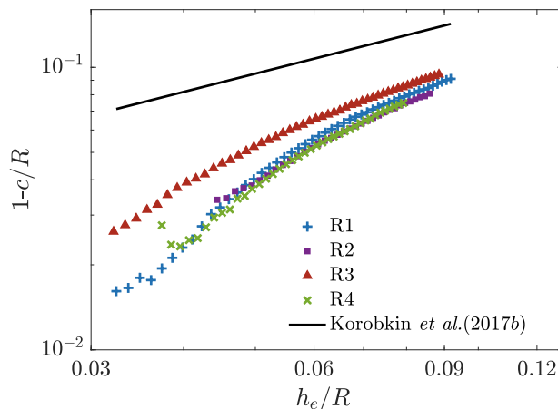
Figure 6: Log-log plot of 1 - c/R versus h_e/R , showing the convergence to the law 1 - c/R \sim (h_e/R)^{2/3} (solid line) predicted by Korobkin et al. (2017b).
