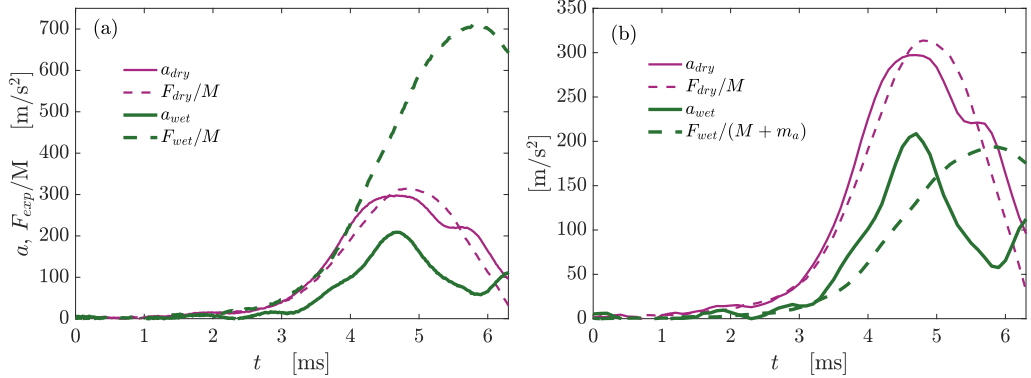
Figure 4: Comparison between the force and acceleration measurements obtained in a dry and a wet case respectively. Sessions 1 and 2 from table 2.
