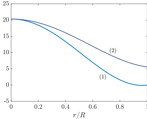
Figure 12: Distributions of radial and tangential normalised stresses along the disc radius, curve (1) corresponds to \tilde{\sigma}_r(\tilde{r}) and (2) to \tilde{\sigma}_t(\tilde{r}) .
