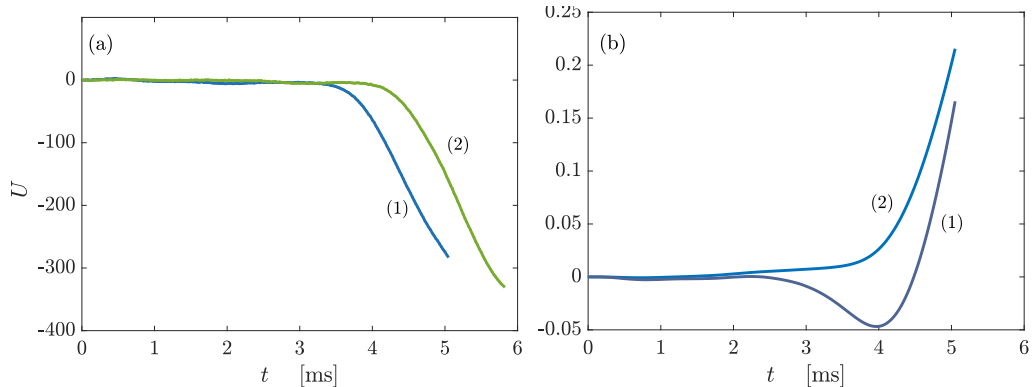
Figure 9: (a) Pressure coefficients U(t) for two repetitions of session 3 (1 and 2). (b) w_t(R, t) (line 1) and V(t) (line 2) for session 3, repetition 1.
