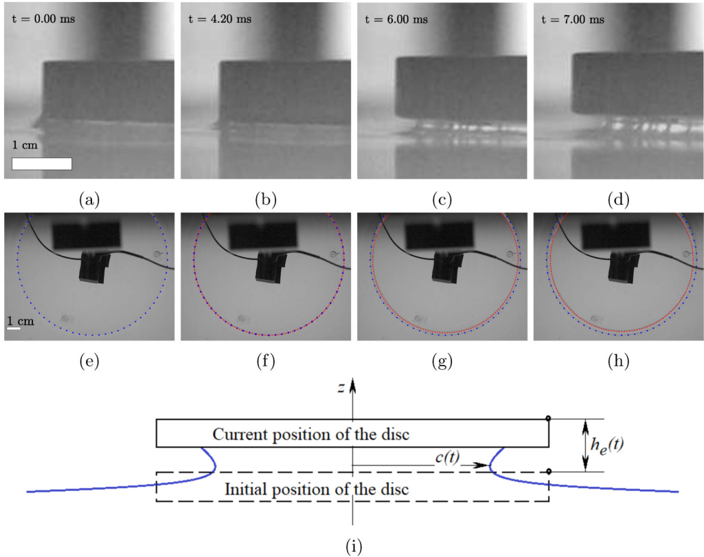
Figure 3: (a–d) Side view of the edge of the plate and (e–h) top view of the plate where the blue dots mark the diameter of the plate and the red dash traces the detection of the contact line. Images acquired at 15000 fps. (i) Definition of c(t) and h_e(t) .
