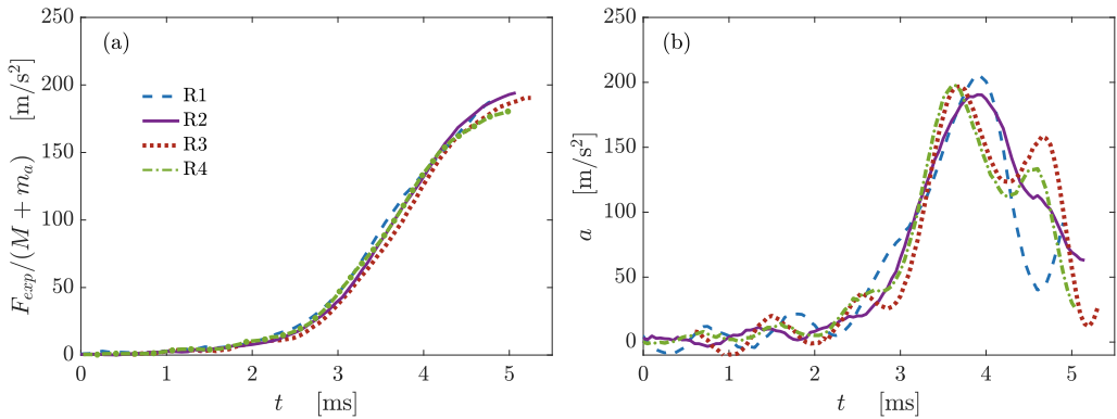
Figure 2: Comparison between force and acceleration measurements obtained under identical experimental conditions for four repetitions of session 3.
