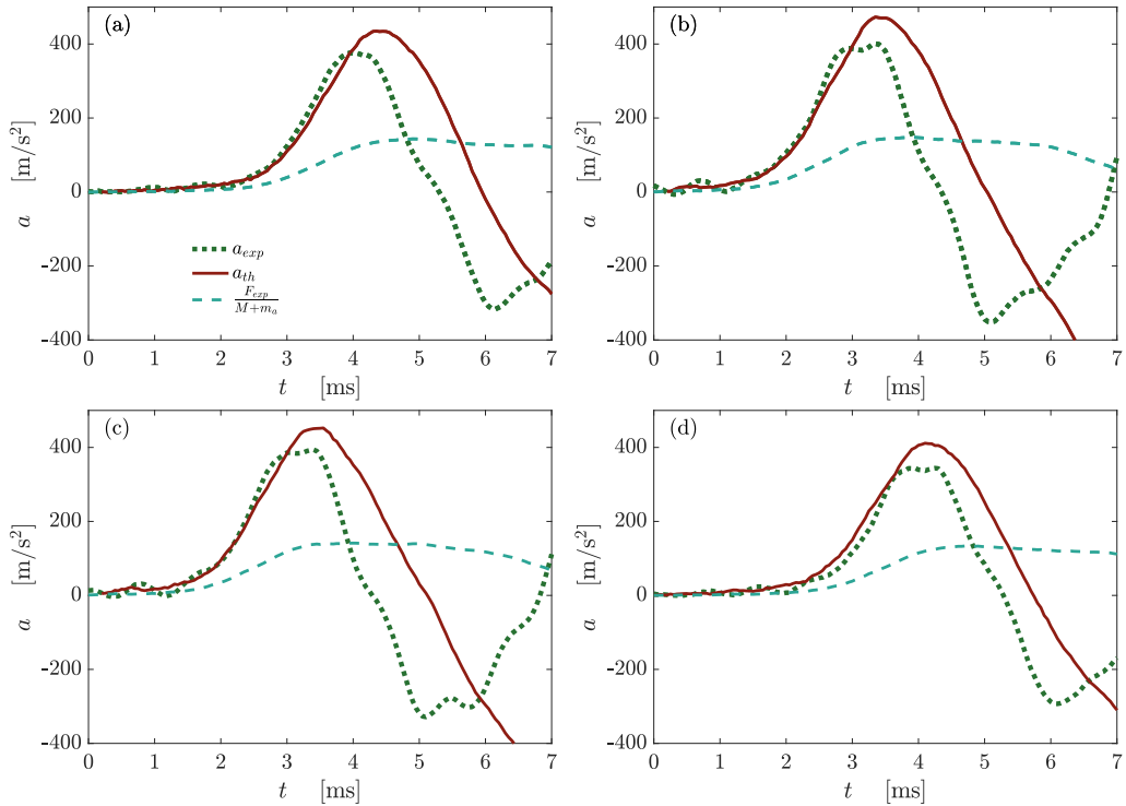
Figure 14: Comparison of theoretical accelerations at the disc centre with the experimental ones (session 5) in four runs for disc thickness, h_p = 0.5 cm. Dashed lines are for the rigid wet-body acceleration, F_{exp}(t)/(M + m_a) , solid lines are for the theoretical accelerations at the disc centre provided by equation (4.25) and dotted lines are for the measured acceleration.
