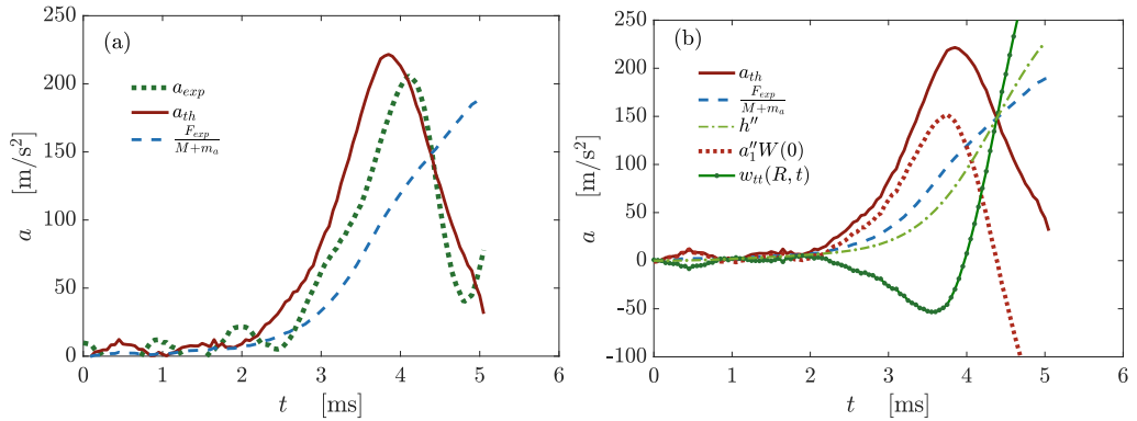
Figure 7: Comparison of experimental and theoretical results for session 3, repetition 1 (see figure 2). (a) Dashed line is for rigid wet-body acceleration F_{exp}(t)/(M + m_a) , solid line is for theoretical acceleration at the disc centre provided by equation (4.33), and the dotted line is for the measured acceleration. (b) rigid wet-body acceleration and theoretical acceleration measured at the center of the disc are the same as in (a), dash-dotted line is for the rigid-body acceleration h''(t) given by (4.32), dotted line is for the elastic acceleration at the plate centre, a_1''W_1(0) , and the solid line with dots markers are for the acceleration of the disc edge, w_{tt}(R, t) .
