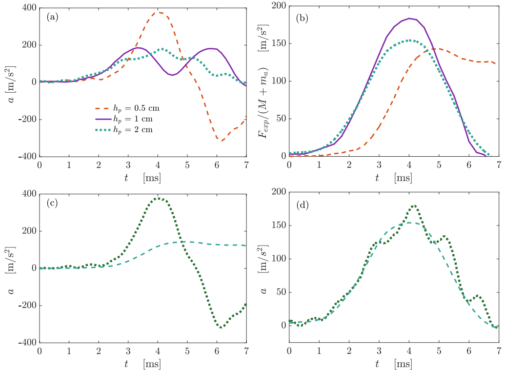
Figure 13: Comparison of the experimental accelerations at the disc centre (a) and the measured rigid wet-body accelerations, F_{exp}(t)/(M + m_a) , (b), for three different plate thicknesses, 0.5, 1, and 2 cm. Comparison between the experimental accelerations (dotted lines) and the rigid wet-body accelerations, F_{exp}(t)/(M + m_a) , (dashed lines) for the plate thicknesses h_p = 0.5 cm (c) and h_p = 2 cm (d).
