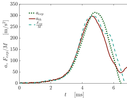
Figure 11: Comparison of the measured acceleration, a_{exp} , the acceleration computed using the load-cell measurements under the rigid-body assumption, F_{exp}/M , and the theoretical acceleration, a_{th} .
