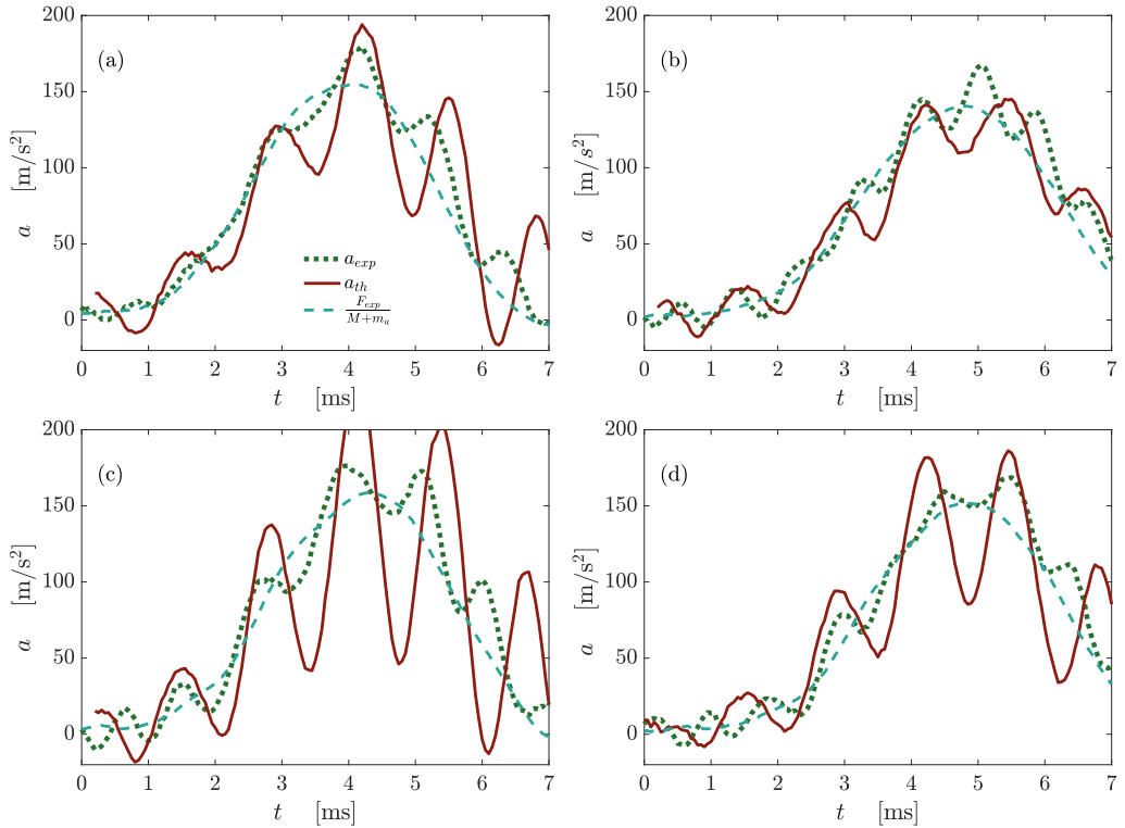
Figure 15: Comparison of theoretical accelerations at the disc centre with the experimental ones (session 4) in other four runs for disc thickness, h_p = 2 cm. See figure 14 for an explanation of the different curves.
