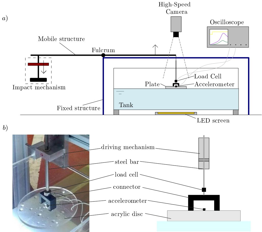
Figure 1: (a) Layout of the experiment. (b) Detail of the plate, which is connected to a driving mechanism through an inverted U-shape structure fixed at its upper surface.
