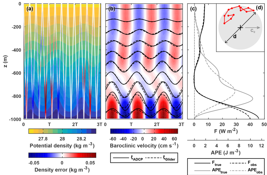
Figure 7. (a) Potential density for an idealized M_2 multi-mode internal tide overlaid with the error in measured density due to imperfect co-location of a glider and ADCP. The x axis is time in M_2 cycles. Positive error indicates an overestimation of density. (b) Baroclinic velocity (colour) for the same idealized internal tide overlaid with vertical isopycnal displacement at the ADCP ( \xi_{\text{ADCP}} , solid black lines) and calculated from measured density ( \xi_{\text{Glider}} , dashed black lines) every 100 m. (c) “True” and “observed” internal tide energy flux (black) and available potential energy (grey). (d) Location of the pseudorandomly distributed glider path (red) relative to the ADCP (black cross). The diameter of the watch circle, d = \lambda/4 , where \lambda = 80 km is the mode-1 horizontal wavelength. c_g is the direction of tide propagation.
