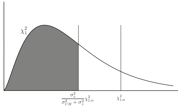
Figure 1: \chi^2 Distribution
