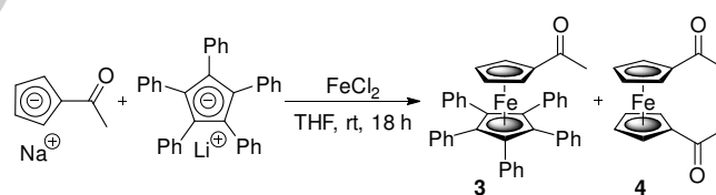
Scheme 2. Previous synthesis of 1-acetyl-1',2',3',4',5'-pentaphenylferrocene. 9
