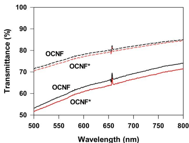
Fig. 3 UV-Vis transmittance spectra of the OCNF and OCNF* dispersions at 0.5 and 1 wt%, dashed and solid line respectively. Error for intrinsic limitation of the equipment of ca. 1 % is within the width of the line.
