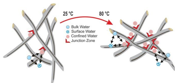
Fig. 6 Schematic representation of the increased overlap of the oxidised cellulose nanofibrils (OCNF) upon heating. After heating, the number junction zones (highlighted in red) between fibrils increase, increasing the amount of confined water, without strong densification of the cluster. Note: cellulose fibrils and water molecules are not to scale
