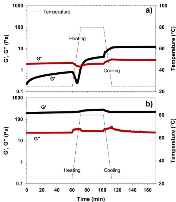
Fig. 1 Storage ( G' ) and loss ( G'' ) moduli as function of temperature and time, a) 1.25 wt% OCNF dispersion and b) 1 wt% CCNF dispersion. The OCNF solid content of 1.25 wt% was selected over 1 wt% as the heat-induced gelation effect is more pronounced at this concentration ( \dagger ESI, Fig. S3 for OCNF at 1, 1.5 and 1.75 wt%). (ii) The concentration of the fibrils used in all experiments is well above the overlap concentration, calculated to be substantially less than 0.1 wt. %. 6 Error for intrinsic limitation of sample loading and equipment of ca. 5%. This is within the size of the symbols used on the graphs.
