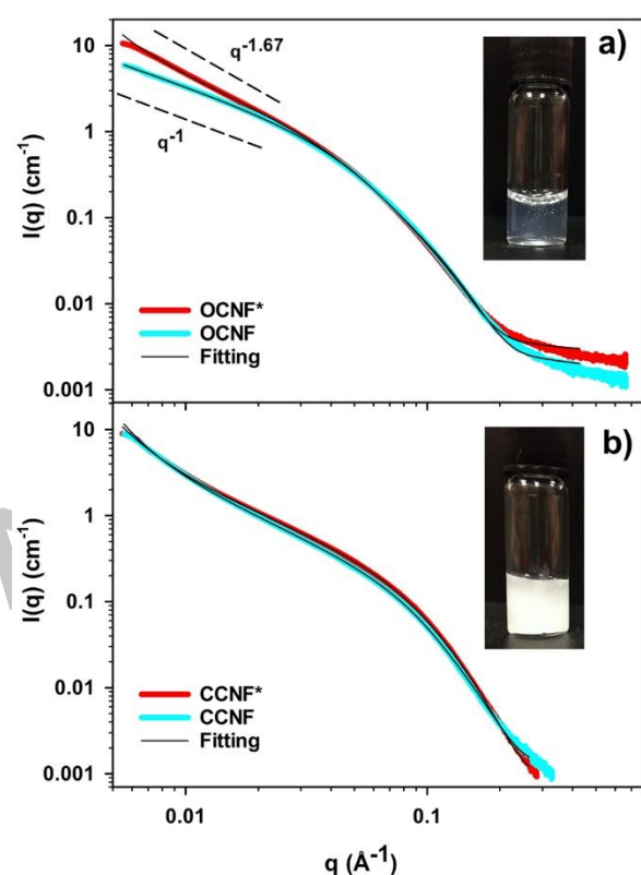
Fig. 4 SAXS patterns for a) 1 wt% OCNF (in blue) and OCNF* (in red) dispersions and b) 1 wt% CCNF (in blue) and CCNF* (in red) dispersions. Intensity is given in absolute scaling ( \text{cm}^{-1} ), errors in the value of the intensity are given on the graph. The black lines are the fits given by a model of interacting rigid cylinders with an elliptical cross-section. Dashed lines indicate the slopes
